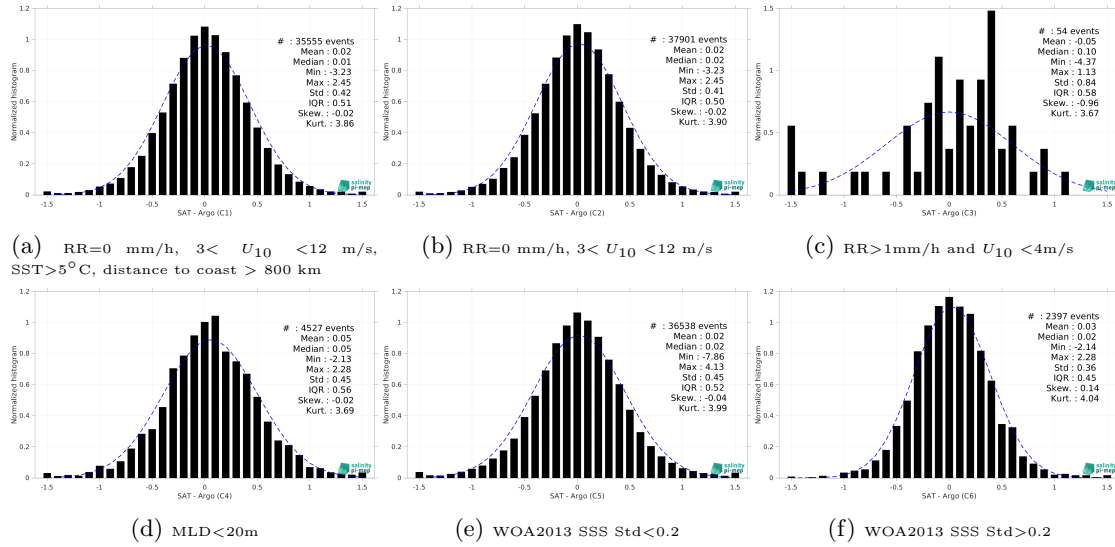
Figure 15: Normalized histogram of \Delta\text{SSS} (SMAP SSS L2 v5.3 (RSS) - Argo) for 6 different subdatasets corresponding to: RR=0 mm/h, 3 < U_{10} < 12 m/s, SST >5^{\circ}\text{C} , distance to coast > 800 km (a), RR=0 mm/h, 3 < U_{10} < 12 m/s (b), RR >1 mm/h and U_{10} < 4 m/s (c), MLD <20 m (d), WOA2013 SSS Std <0.2 (e), WOA2013 SSS Std >0.2 (f).
