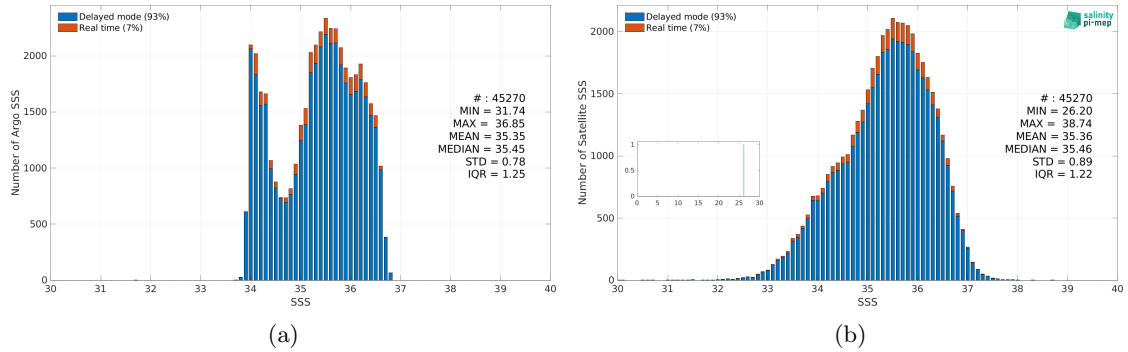
Figure 3: Histograms of SSS from Argo (a) and SMAP SSS L2 v5.3 (RSS) (b) considering all match-up pairs per bins of 0.1 over the OTT zone Pi-MEP region and for the full satellite product period.
