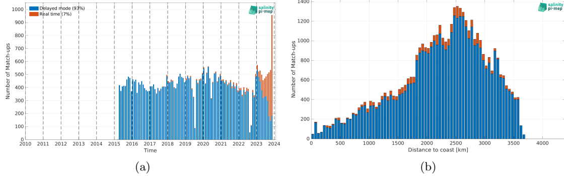
Figure 2: Number of match-ups between Argo and SMAP SSS L2 v5.3 (RSS) SSS as a function of time (a) and as function of the distance to coast (b) over the OTT zone Pi-MEP region and for the full satellite product period.
