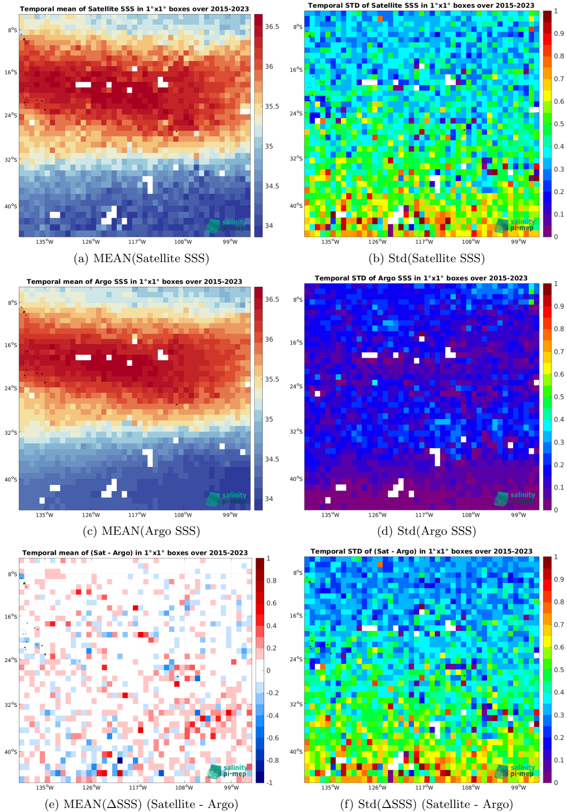
Figure 7: Temporal mean (left) and Std (right) of SSS from SMAP SSS L2 v5.3 (RSS) (top), Argo (middle), and of \Delta SSS (Satellite - Argo). Only match-up pairs are used to generate these maps.
