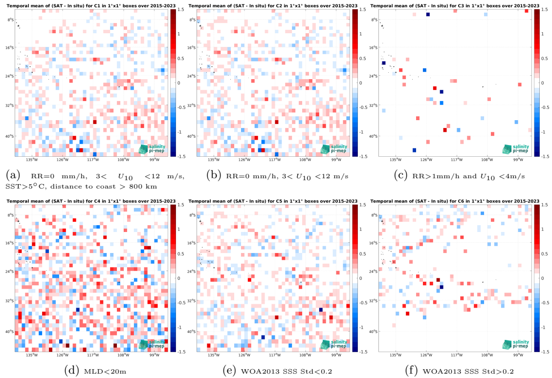
Figure 14: Temporal mean gridded over spatial boxes of size 1^\circ \times 1^\circ of \Delta SSS (SMAP SSS L2 v5.3 (RSS) - Argo) for 6 different subdatasets corresponding to:RR=0 mm/h, 3 < U_{10} < 12 m/s, SST >5^\circ C, distance to coast > 800 km (a), RR=0 mm/h, 3 < U_{10} < 12 m/s (b), RR >1 mm/h and U_{10} < 4 m/s (c),MLD <20 m (d),WOA2013 SSS Std <0.2 (e),WOA2013 SSS Std >0.2 (f).
