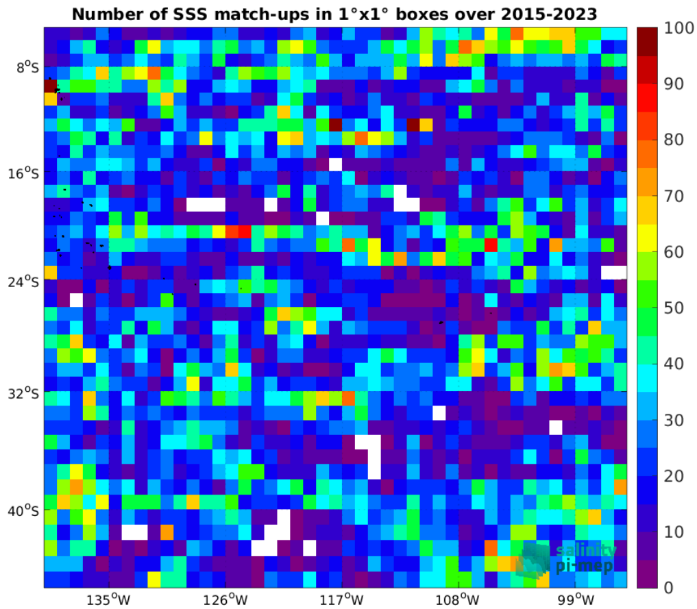
Figure 5: Number of SSS match-ups between Argo SSS and the SMAP SSS L2 v5.3 (RSS) SSS product for the OTT zone Pi-MEP region over 1^\circ \times 1^\circ boxes and for the full satellite product period.
