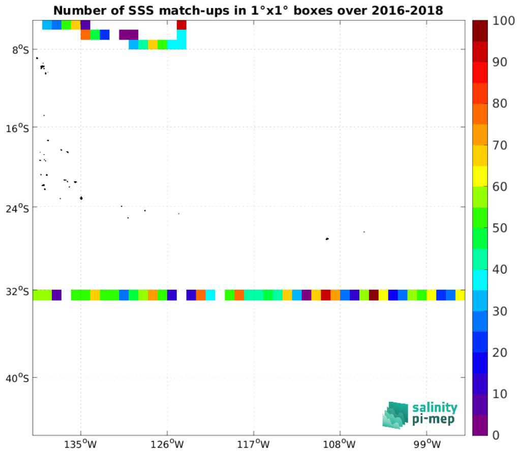
Figure 5: Number of SSS match-ups between TSG (SAMOS) SSS and the SMAP SSS L2 v5.3 - 40 km (RSS) SSS product for the OTT zone Pi-MEP region over 1°x1° boxes and for the full satellite product period.
