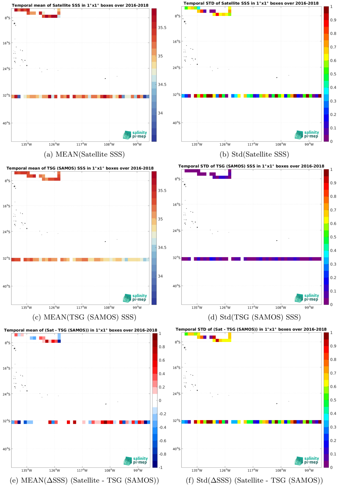
Figure 7: Temporal mean (left) and Std (right) of SSS from SMAP SSS L2 v5.3 - 40 km (RSS) (top), TSG (SAMOS) (middle), and of \Delta SSS (Satellite - TSG (SAMOS)). Only match-up pairs are used to generate these maps.
