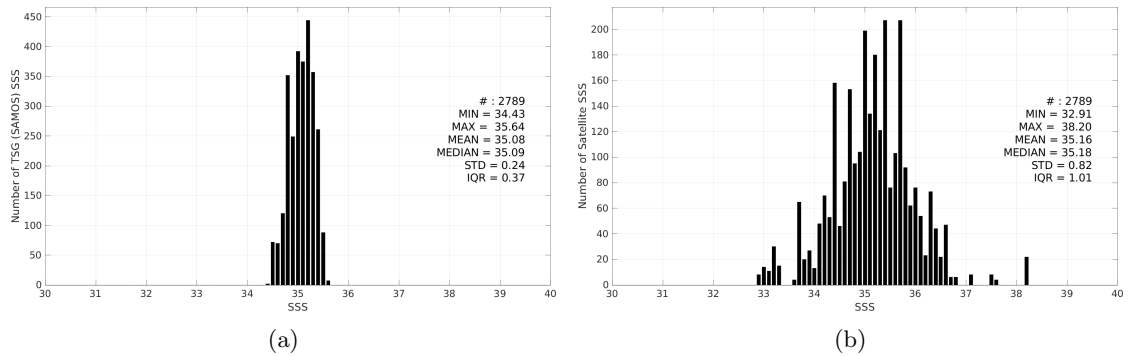
Figure 3: Histograms of SSS from TSG (SAMOS) (a) and SMAP SSS L2 v5.3 - 40 km (RSS) (b) considering all match-up pairs per bins of 0.1 over the OTT zone Pi-MEP region and for the full satellite product period.
