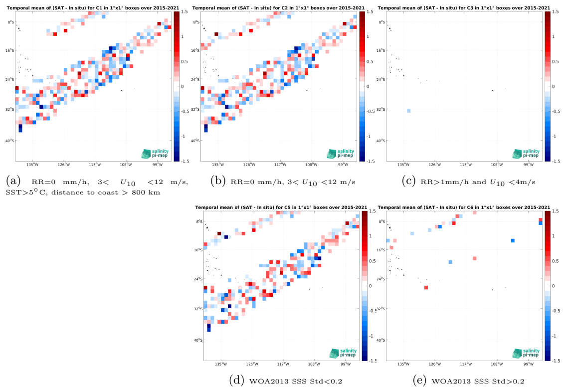
Figure 14: Temporal mean gridded over spatial boxes of size 1^\circ \times 1^\circ of \Delta SSS (SMAP SSS L2 v5.3 - 40 km (RSS) - TSG (LEGOS-DM)) for 5 different subdatasets corresponding to:RR=0 mm/h, 3 < U_{10} < 12 m/s, SST >5^\circ C, distance to coast > 800 km (a), RR=0 mm/h, 3 < U_{10} < 12 m/s (b), RR >1 mm/h and U_{10} < 4 m/s (c), WOA2013 SSS Std <0.2 (d), WOA2013 SSS Std >0.2 (e).
