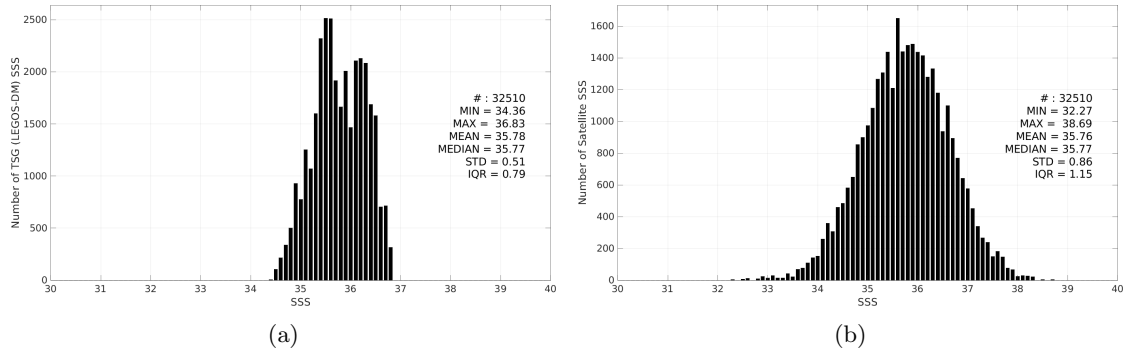
Figure 3: Histograms of SSS from TSG (LEGOS-DM) (a) and SMAP SSS L2 v5.3 - 40 km (RSS) (b) considering all match-up pairs per bins of 0.1 over the OTT zone Pi-MEP region and for the full satellite product period.
