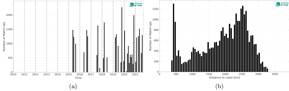
Figure 2: Number of match-ups between TSG (LEGOS-DM) and SMAP SSS L2 v5.3 - 40 km (RSS) SSS as a function of time (a) and as function of the distance to coast (b) over the OTT zone Pi-MEP region and for the full satellite product period.
