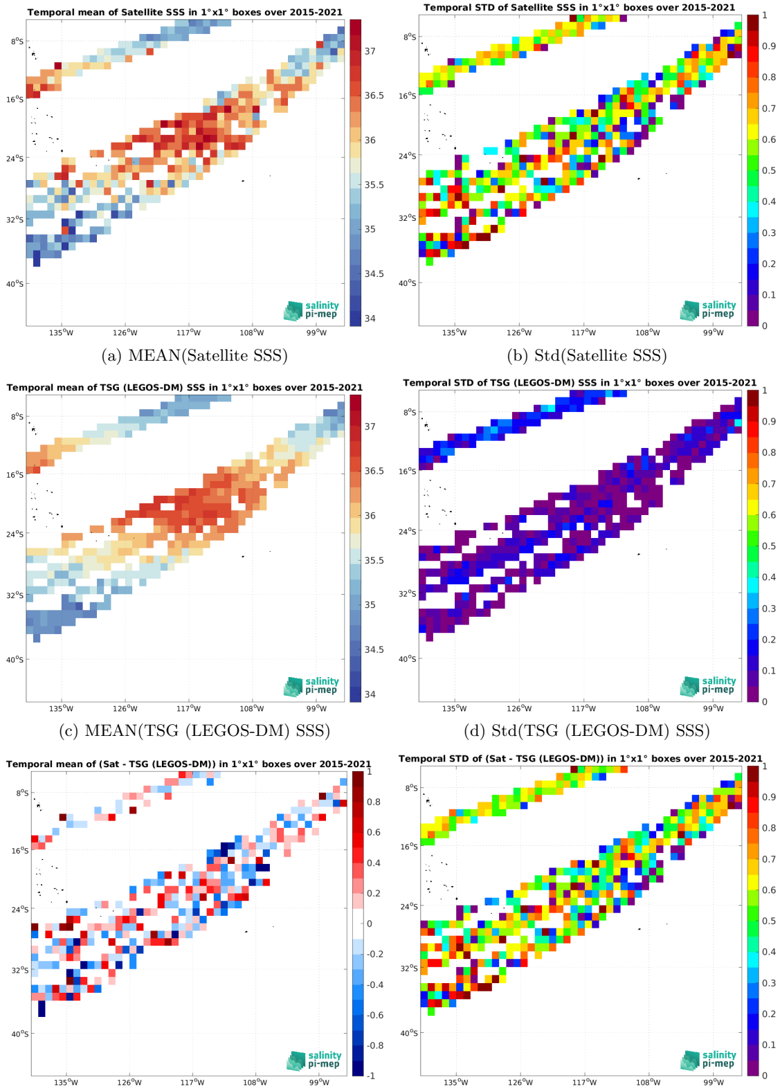
Figure 7: Temporal mean (left) and Std (right) of SSS from SMAP SSS L2 v5.3 - 40 km (RSS) (top), TSG (LEGOS-DM) (middle), and of \Delta SSS (Satellite - TSG (LEGOS-DM)). Only match-up pairs are used to generate these maps.
