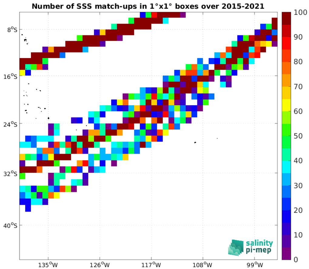
Figure 5: Number of SSS match-ups between TSG (LEGOS-DM) SSS and the SMAP SSS L2 v5.3 - 40 km (RSS) SSS product for the OTT zone Pi-MEP region over 1^\circ \times 1^\circ boxes and for the full satellite product period.
