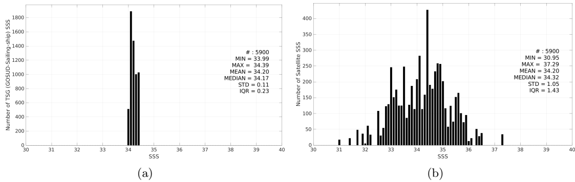
Figure 3: Histograms of SSS from TSG (GOSUD-Sailing-ship) (a) and SMAP SSS L2 v5.3 - 40 km (RSS) (b) considering all match-up pairs per bins of 0.1 over the OTT zone Pi-MEP region and for the full satellite product period.
