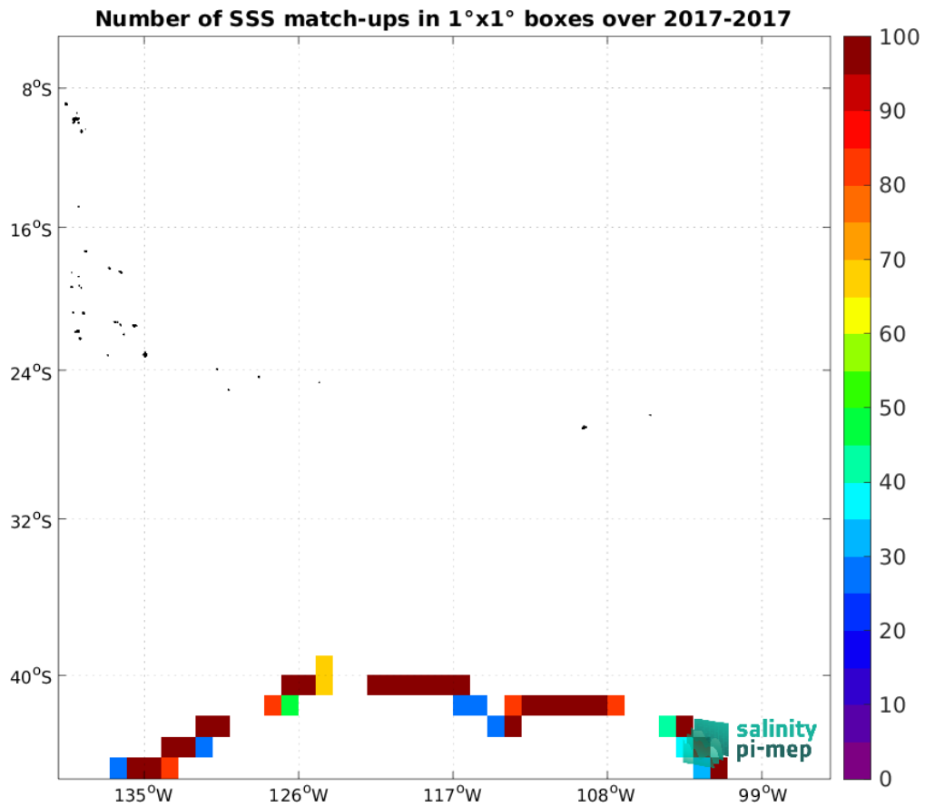
Figure 5: Number of SSS match-ups between TSG (GOSUD-Sailing-ship) SSS and the SMAP SSS L2 v5.3 - 40 km (RSS) SSS product for the OTT zone Pi-MEP region over 1°x1° boxes and for the full satellite product period.
