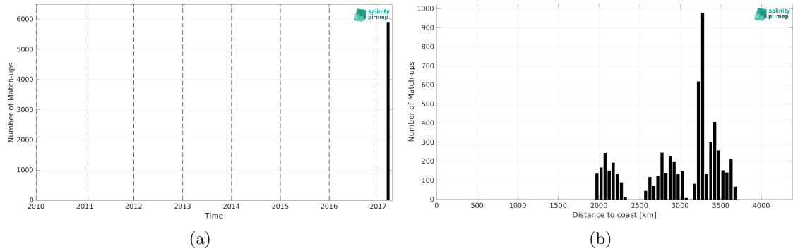
Figure 2: Number of match-ups between TSG (GOSUD-Sailing-ship) and SMAP SSS L2 v5.3 - 40 km (RSS) SSS as a function of time (a) and as function of the distance to coast (b) over the OTT zone Pi-MEP region and for the full satellite product period.
