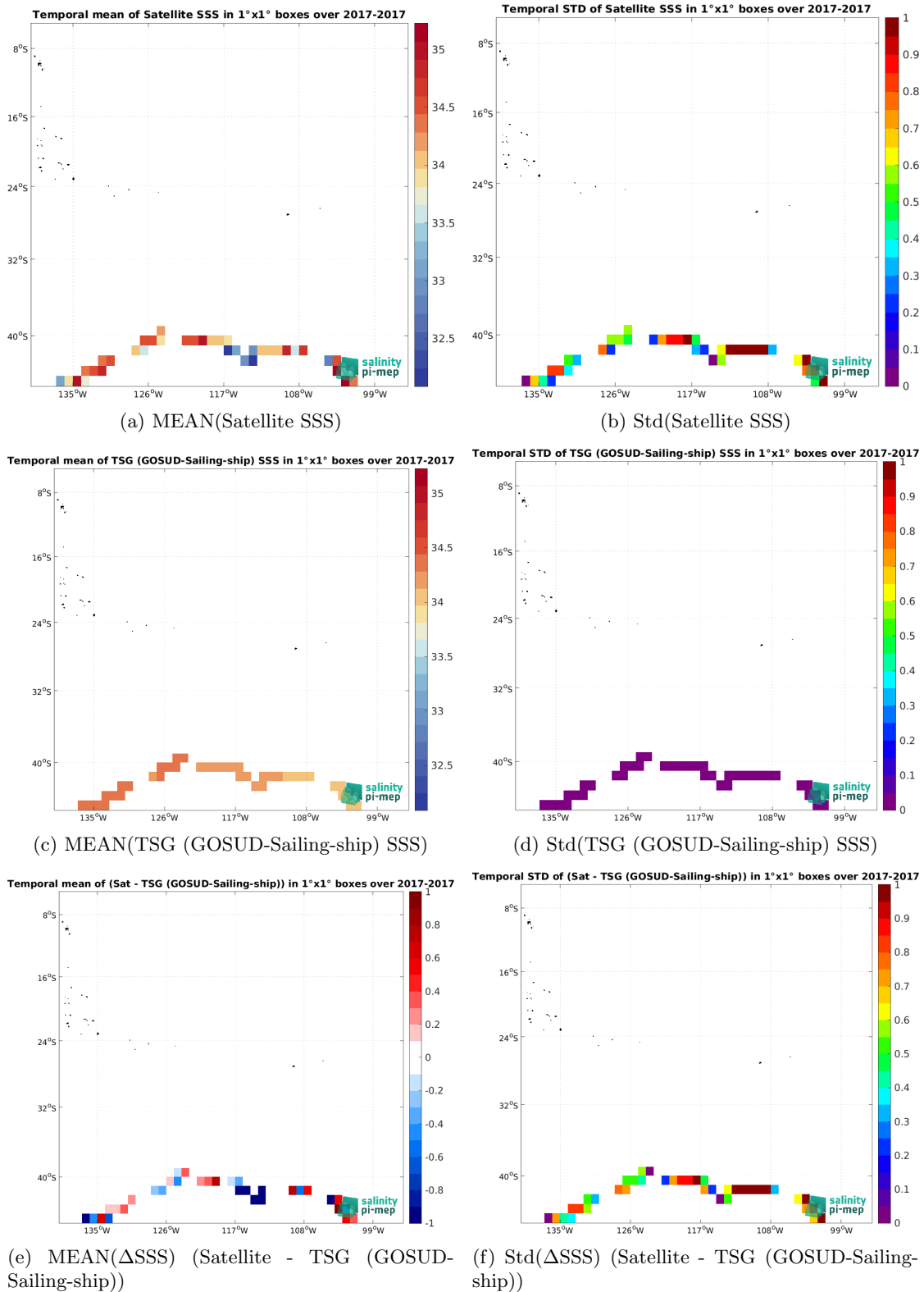
Figure 7: Temporal mean (left) and Std (right) of SSS from SMAP SSS L2 v5.3 - 40 km (RSS) (top), TSG (GOSUD-Sailing-ship) (middle), and of \Delta SSS (Satellite - TSG (GOSUD-Sailing-ship)). Only match-up pairs are used to generate these maps.
