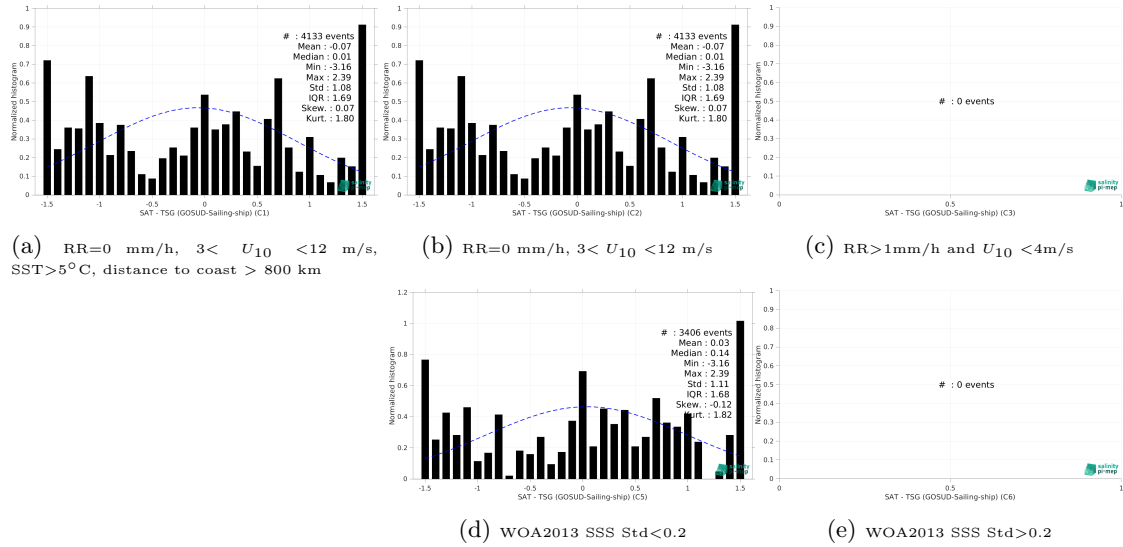
Figure 15: Normalized histogram of \Delta\text{SSS} (SMAP SSS L2 v5.3 - 40 km (RSS) - TSG (GOSUD-Sailing-ship)) for 5 different subdatasets corresponding to: RR=0 mm/h, 3 < U_{10} < 12 m/s, SST >5^{\circ}\text{C} , distance to coast > 800 km (a), RR=0 mm/h, 3 < U_{10} < 12 m/s (b), RR >1 mm/h and U_{10} < 4 m/s (c), WOA2013 SSS Std <0.2 (d), WOA2013 SSS Std >0.2 (e).
