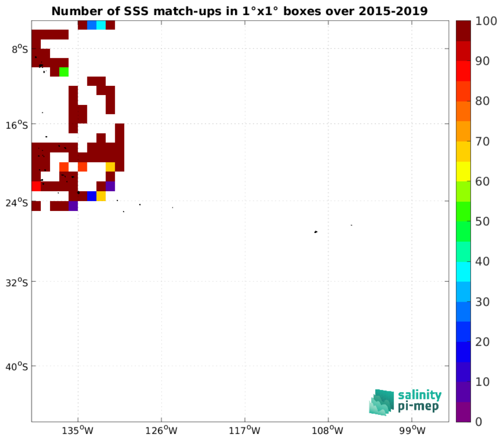
Figure 5: Number of SSS match-ups between TSG (GOSUD-Research-vessel) SSS and the SMAP SSS L2 v5.3 - 40 km (RSS) SSS product for the OTT zone Pi-MEP region over 1^\circ \times 1^\circ boxes and for the full satellite product period.
