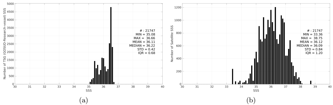
Figure 3: Histograms of SSS from TSG (GOSUD-Research-vessel) (a) and SMAP SSS L2 v5.3 - 40 km (RSS) (b) considering all match-up pairs per bins of 0.1 over the OTT zone Pi-MEP region and for the full satellite product period.
