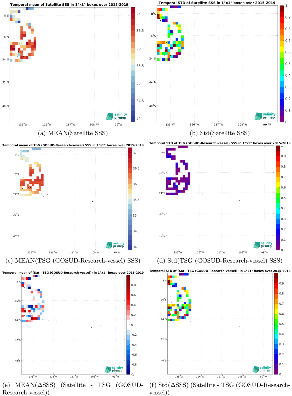
Figure 7: Temporal mean (left) and Std (right) of SSS from SMAP SSS L2 v5.3 - 40 km (RSS) (top), TSG (GOSUD-Research-vessel) (middle), and of \Delta SSS (Satellite - TSG (GOSUD-Research-vessel)). Only match-up pairs are used to generate these maps.
