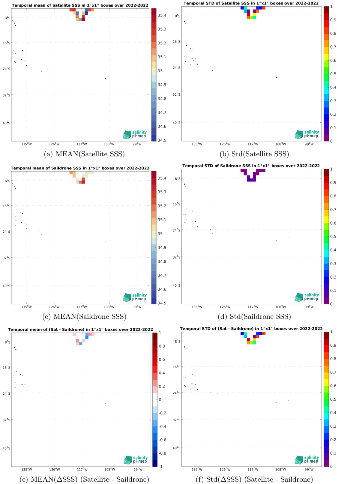
Figure 7: Temporal mean (left) and Std (right) of SSS from SMAP SSS L2 v5.3 - 40 km (RSS) (top), Saildrone (middle), and of \Delta SSS (Satellite - Saildrone). Only match-up pairs are used to generate these maps.
