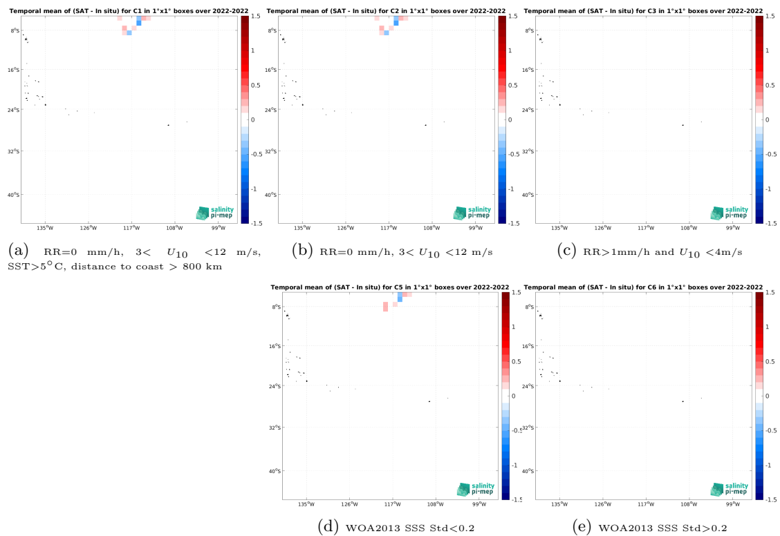
Figure 14: Temporal mean gridded over spatial boxes of size 1^\circ \times 1^\circ of \Delta SSS (SMAP SSS L2 v5.3 - 40 km (RSS) - Sairdrone) for 5 different subdatasets corresponding to:RR=0 mm/h, 3 < U_{10} < 12 m/s, SST > 5^\circ\text{C} , distance to coast > 800 km (a), RR=0 mm/h, 3 < U_{10} < 12 m/s (b), RR > 1 mm/h and U_{10} < 4 m/s (c), WOA2013 SSS Std < 0.2 (d), WOA2013 SSS Std > 0.2 (e).
