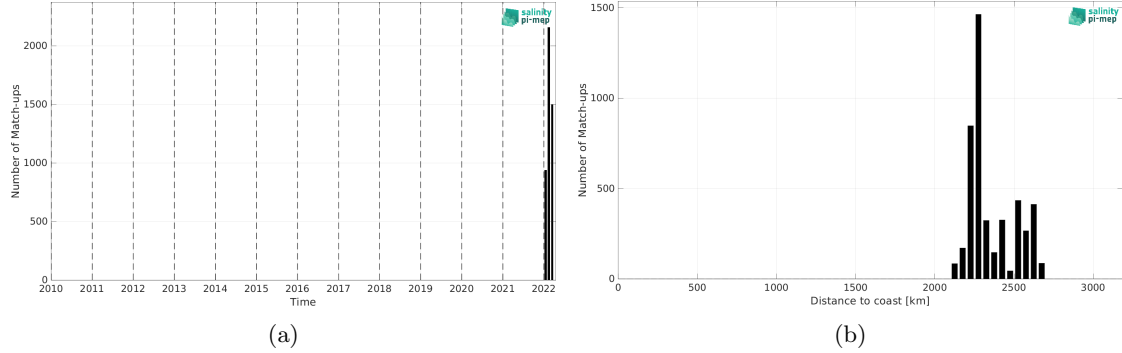
Figure 2: Number of match-ups between Saildrone and SMAP SSS L2 v5.3 - 40 km (RSS) SSS as a function of time (a) and as function of the distance to coast (b) over the OTT zone Pi-MEP region and for the full satellite product period.
