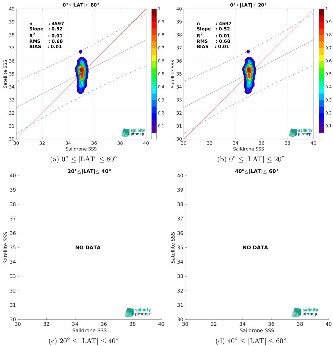
Figure 10: Contour maps of the concentration of SMAP SSS L2 v5.3 - 40 km (RSS) SSS (y-axis) versus Sailldrone SSS (x-axis) at match-up pairs for different latitude bands. For each plot, the red line shows x=y . The black thin and dashed lines indicate a linear fit through the data cloud and the \pm 95\% confidence levels, respectively. The number match-up pairs n , the slope and R^2 coefficient of the linear fit, the root mean square (RMS) and the mean bias between satellite and in situ data are indicated for each latitude band in each plots.
