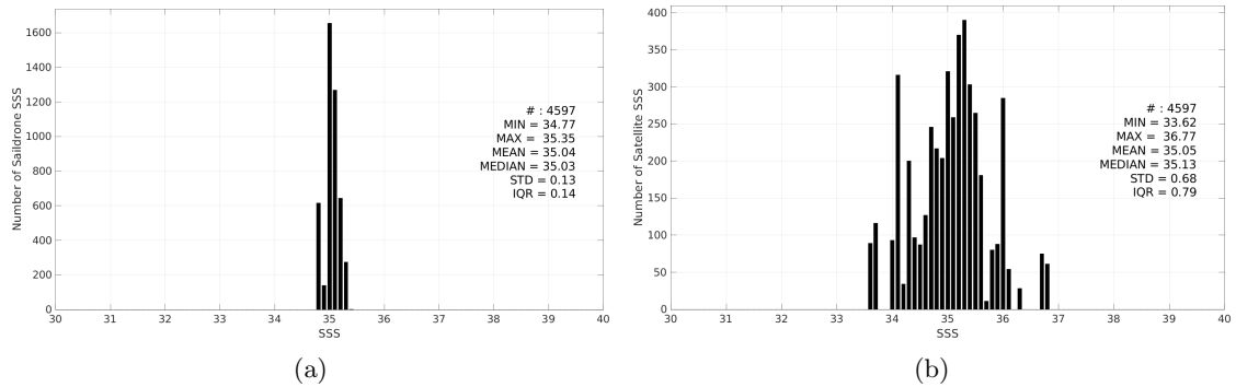
Figure 3: Histograms of SSS from Saildrone (a) and SMAP SSS L2 v5.3 - 40 km (RSS) (b) considering all match-up pairs per bins of 0.1 over the OTT zone Pi-MEP region and for the full satellite product period.
