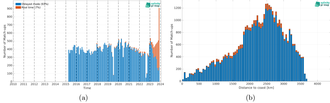
Figure 2: Number of match-ups between Argo and SMAP SSS L2 v5.3 - 40 km (RSS) SSS as a function of time (a) and as function of the distance to coast (b) over the OTT zone Pi-MEP region and for the full satellite product period.
