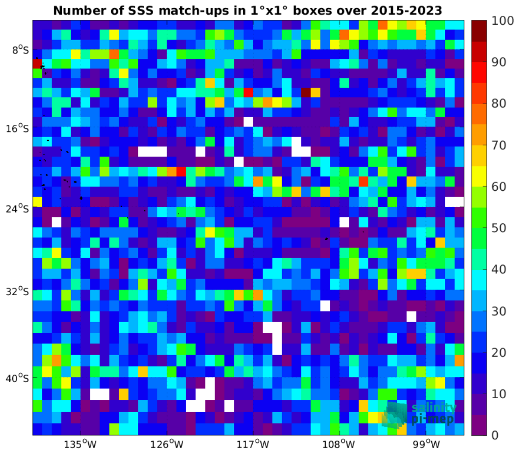
Figure 5: Number of SSS match-ups between Argo SSS and the SMAP SSS L2 v5.3 - 40 km (RSS) SSS product for the OTT zone Pi-MEP region over 1°x1° boxes and for the full satellite product period.
