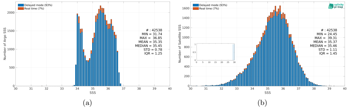
Figure 3: Histograms of SSS from Argo (a) and SMAP SSS L2 v5.3 - 40 km (RSS) (b) considering all match-up pairs per bins of 0.1 over the OTT zone Pi-MEP region and for the full satellite product period.
