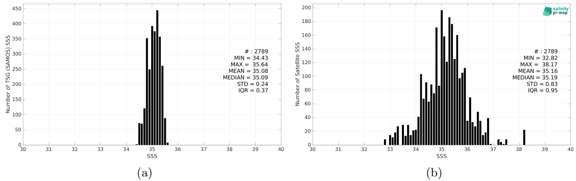
Figure 2: Histograms of SSS from TSG (SAMOS) (a) and SMAP SSS L2 v5 - 40 km (RSS) (b) considering all match-up pairs per bins of 0.1 over the OTT zone Pi-MEP region and for the full satellite product period.
