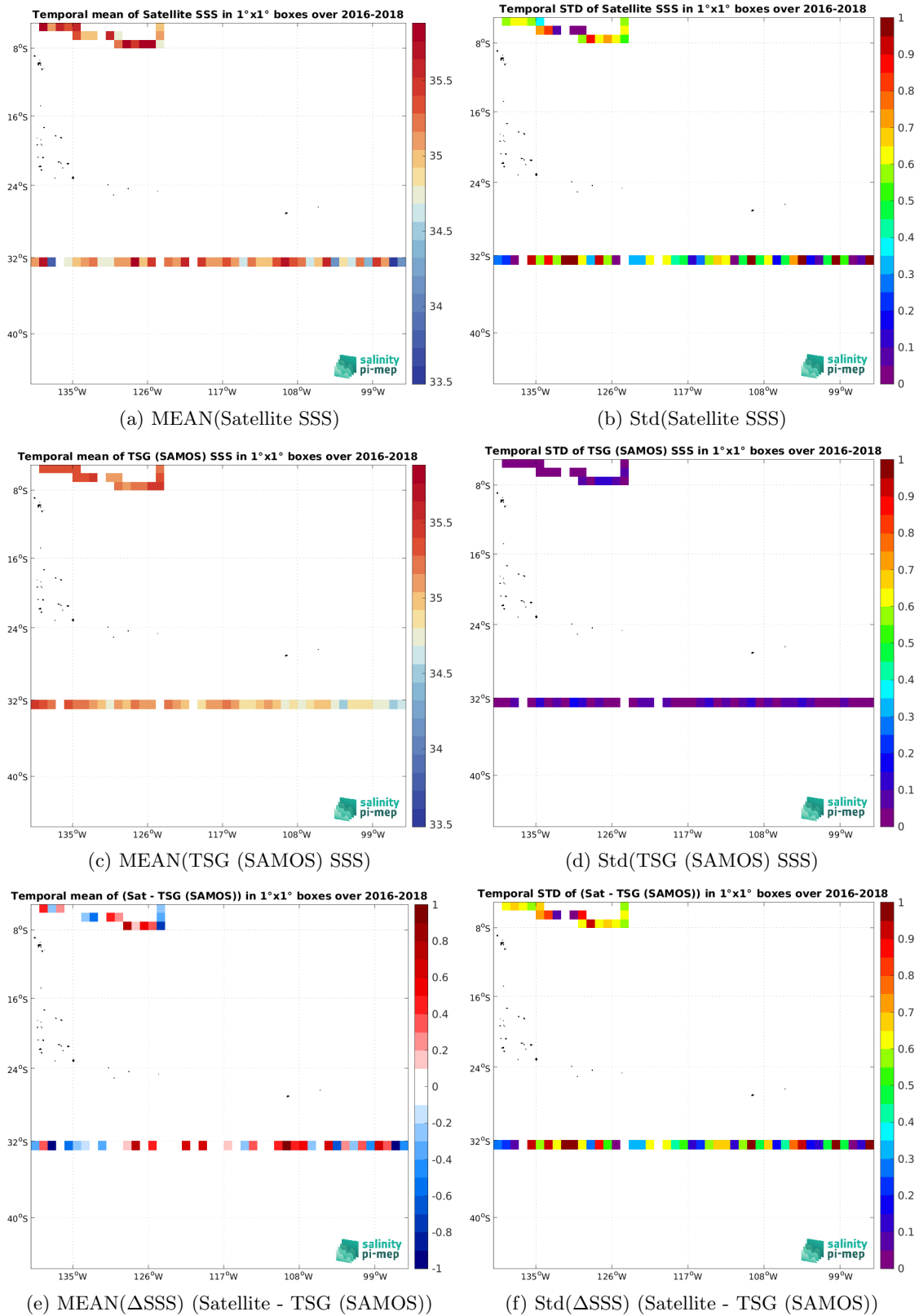
Figure 6: Temporal mean (left) and Std (right) of SSS from SMAP SSS L2 v5 - 40 km (RSS) (top), TSG (SAMOS) (middle), and of \Delta SSS (Satellite - TSG (SAMOS)). Only match-up pairs are used to generate these maps.
