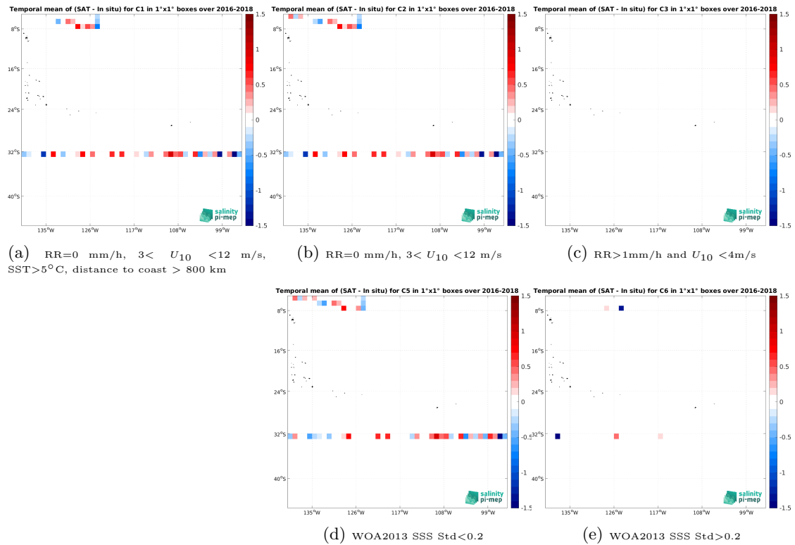
Figure 12: Temporal mean gridded over spatial boxes of size 1^\circ \times 1^\circ of \Delta SSS (SMAP SSS L2 v5 - 40 km (RSS) - TSG (SAMOS)) for 5 different subdatasets corresponding to: RR=0 mm/h, 3 < U_{10} < 12 m/s, SST > 5^\circ C , distance to coast > 800 km (a), RR=0 mm/h, 3 < U_{10} < 12 m/s (b), RR > 1 mm/h and U_{10} < 4 m/s (c), WOA2013 SSS Std < 0.2 (d), WOA2013 SSS Std > 0.2 (e).
