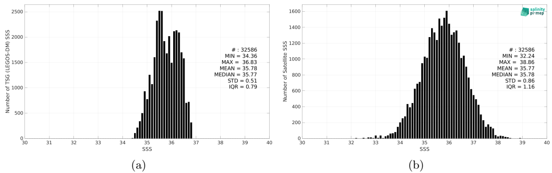
Figure 2: Histograms of SSS from TSG (LEGOS-DM) (a) and SMAP SSS L2 v5 - 40 km (RSS) (b) considering all match-up pairs per bins of 0.1 over the OTT zone Pi-MEP region and for the full satellite product period.
