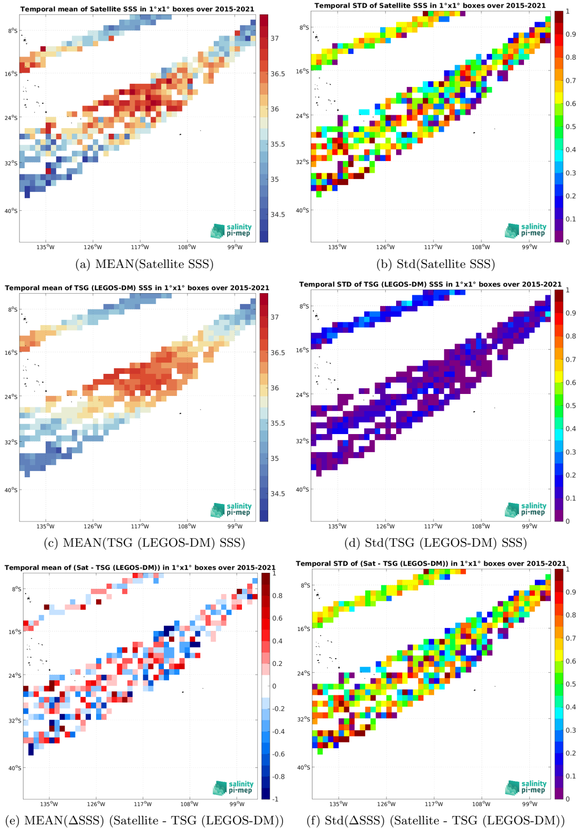
(e) MEAN( \Delta SSS) (Satellite - TSG (LEGOS-DM)) (f) Std( \Delta SSS) (Satellite - TSG (LEGOS-DM)) Figure 6: Temporal mean (left) and Std (right) of SSS from SMAP SSS L2 v5 - 40 km (RSS) (top), TSG (LEGOS-DM) (middle), and of \Delta SSS (Satellite - TSG (LEGOS-DM)). Only match-up pairs are used to generate these maps.
