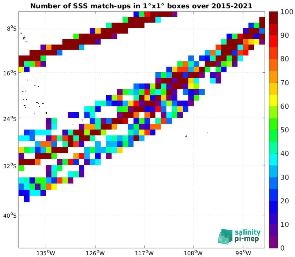
Figure 4: Number of SSS match-ups between TSG (LEGOS-DM) SSS and the SMAP SSS L2 v5 - 40 km (RSS) SSS product for the OTT zone Pi-MEP region over 1^\circ \times 1^\circ boxes and for the full satellite product period.
