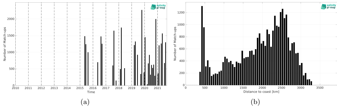
Figure 1: Number of match-ups between TSG (LEGOS-DM) and SMAP SSS L2 v5 - 40 km (RSS) SSS as a function of time (a) and as function of the distance to coast (b) over the OTT zone Pi-MEP region and for the full satellite product period.
