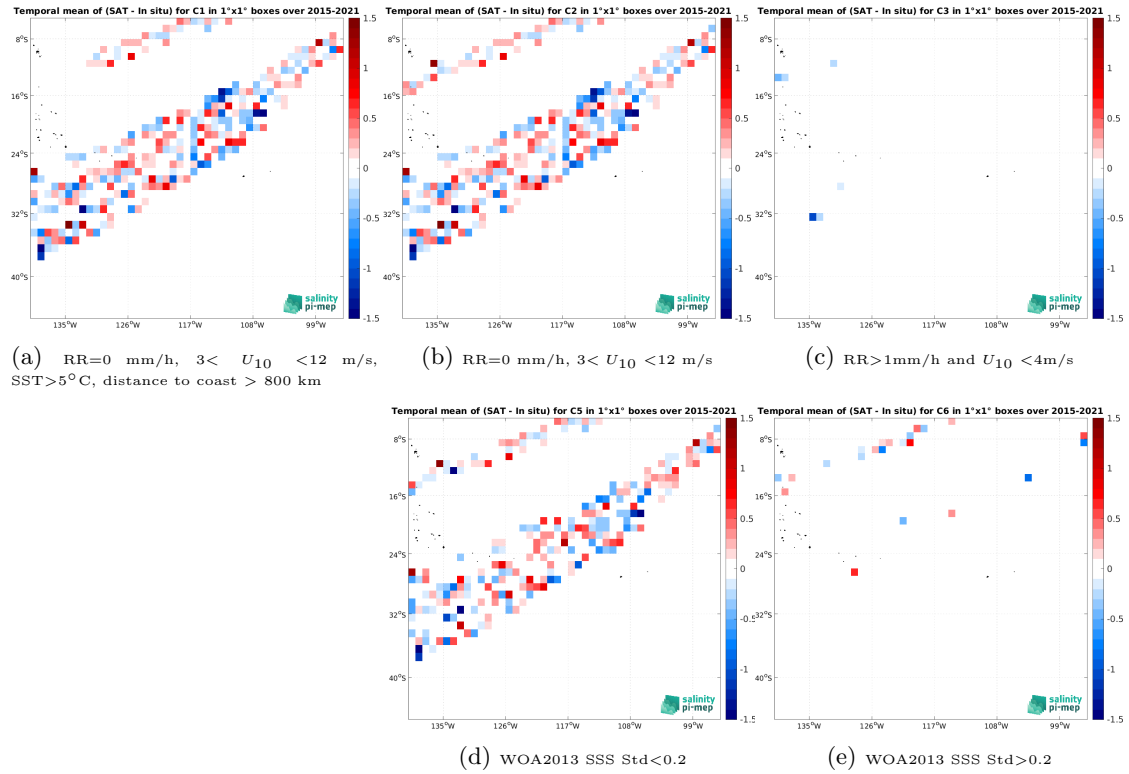
Figure 12: Temporal mean gridded over spatial boxes of size 1^\circ \times 1^\circ of \Delta SSS (SMAP SSS L2 v5 - 40 km (RSS) - TSG (LEGOS-DM)) for 5 different subdatasets corresponding to: RR=0 mm/h, 3 < U_{10} < 12 m/s, SST > 5^\circ C , distance to coast > 800 km (a), RR=0 mm/h, 3 < U_{10} < 12 m/s (b), RR > 1 mm/h and U_{10} < 4 m/s (c), WOA2013 SSS Std < 0.2 (d), WOA2013 SSS Std > 0.2 (e).
