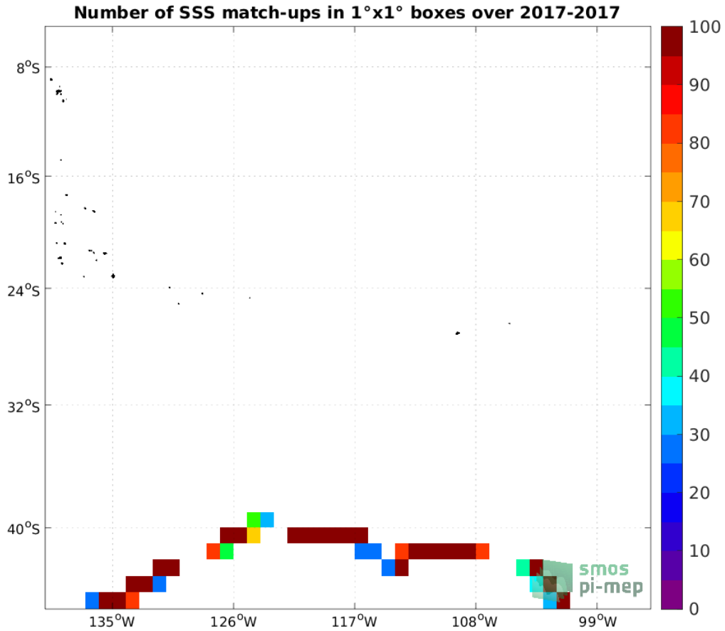
Figure 4: Number of SSS match-ups between TSG (GOSUD-Sailing-ship) SSS and the SMAP SSS L2 v5 - 40 km (RSS) SSS product for the OTT zone Pi-MEP region over 1^\circ \times 1^\circ boxes and for the full satellite product period.
