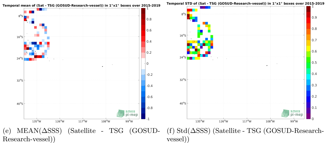
Figure 6: Temporal mean (left) and Std (right) of SSS from SMAP SSS L2 v5 - 40 km (RSS) (top), TSG (GOSUD-Research-vessel) (middle), and of \Delta SSS (Satellite - TSG (GOSUD-Research-vessel)). Only match-up pairs are used to generate these maps.
