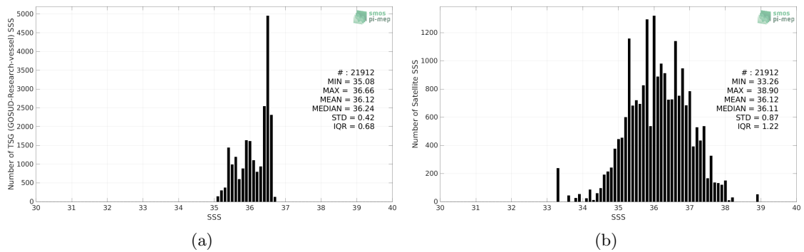
Figure 2: Histograms of SSS from TSG (GOSUD-Research-vessel) (a) and SMAP SSS L2 v5 - 40 km (RSS) (b) considering all match-up pairs per bins of 0.1 over the OTT zone Pi-MEP region and for the full satellite product period.
