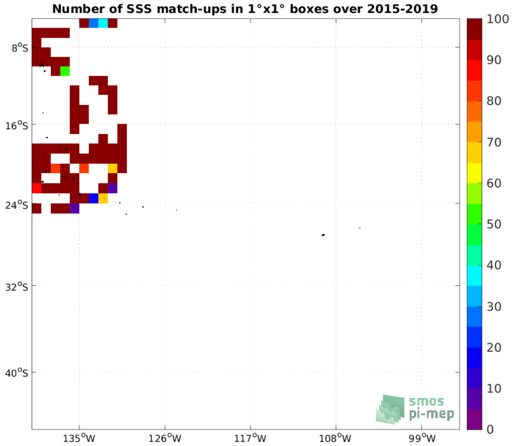
Figure 4: Number of SSS match-ups between TSG (GOSUD-Research-vessel) SSS and the SMAP SSS L2 v5 - 40 km (RSS) SSS product for the OTT zone Pi-MEP region over 1^\circ \times 1^\circ boxes and for the full satellite product period.
