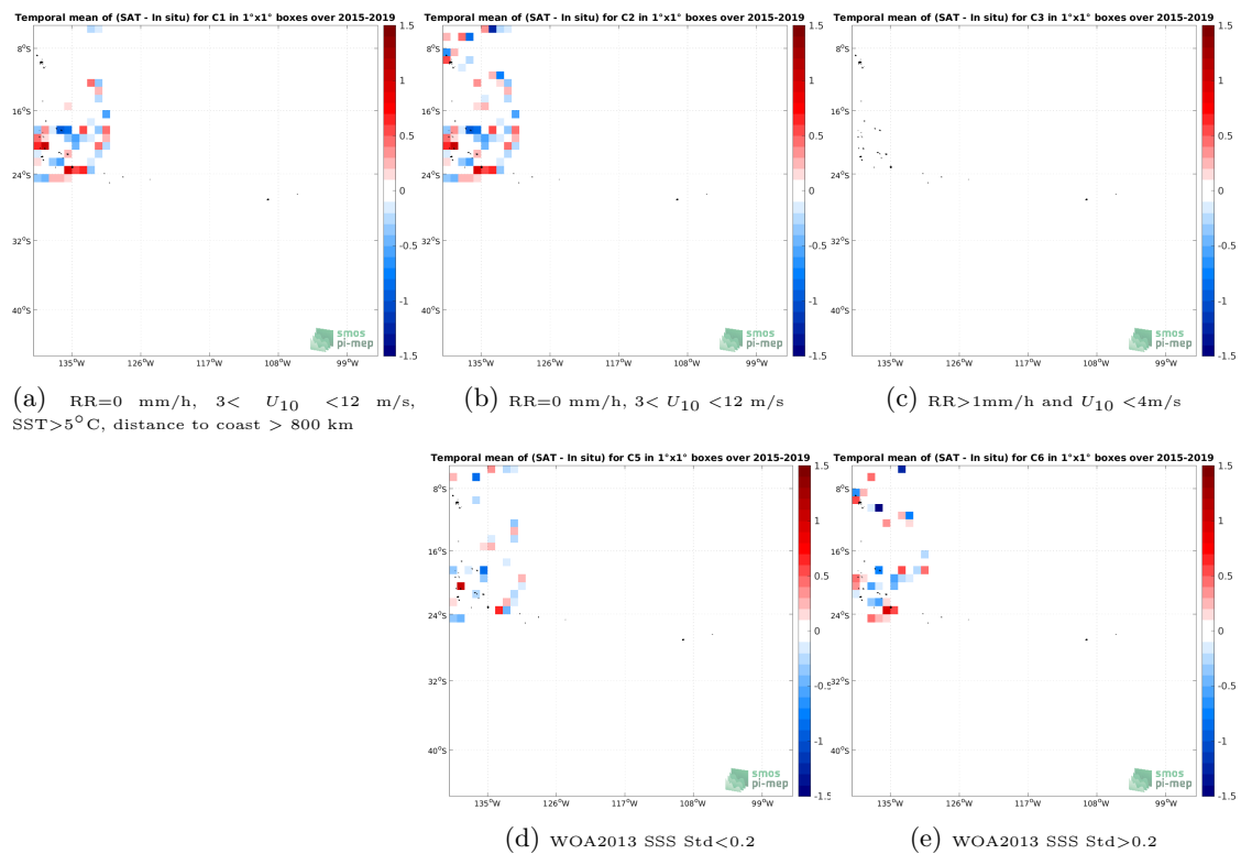
Figure 12: Temporal mean gridded over spatial boxes of size 1^\circ \times 1^\circ of \Delta SSS (SMAP SSS L2 v5 - 40 km (RSS) - TSG (GOSUD-Research-vessel)) for 5 different subdatasets corresponding to:RR=0 mm/h, 3 < U_{10} < 12 m/s, SST>5°C, distance to coast > 800 km (a), RR=0 mm/h, 3 < U_{10} < 12 m/s (b), RR>1mm/h and U_{10} < 4 m/s (c), WOA2013 SSS Std<0.2 (d), WOA2013 SSS Std>0.2 (e).
