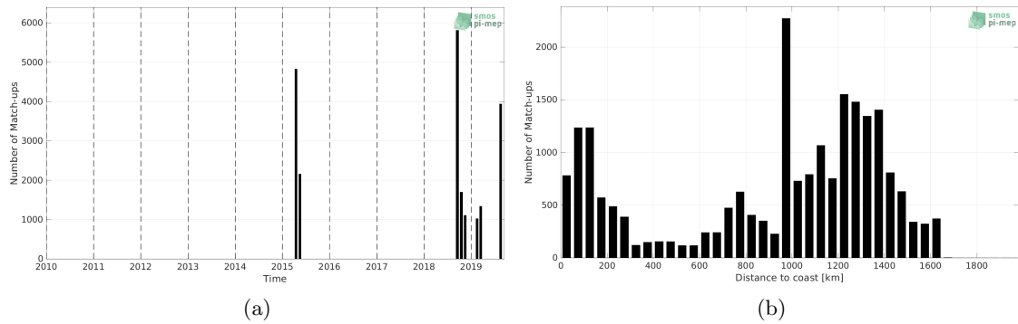
Figure 1: Number of match-ups between TSG (GOSUD-Research-vessel) and SMAP SSS L2 v5 - 40 km (RSS) SSS as a function of time (a) and as function of the distance to coast (b) over the OTT zone Pi-MEP region and for the full satellite product period.
