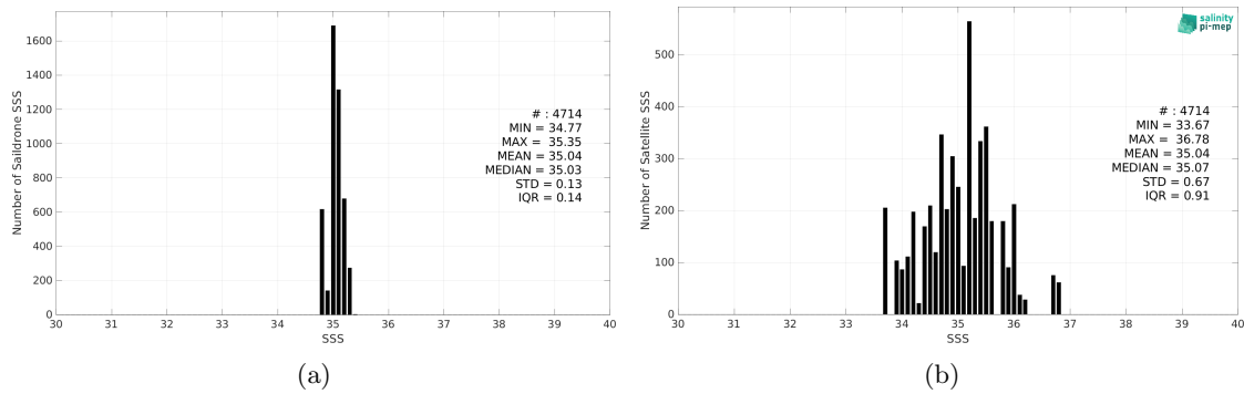
Figure 2: Histograms of SSS from Saildrone (a) and SMAP SSS L2 v5 - 40 km (RSS) (b) considering all match-up pairs per bins of 0.1 over the OTT zone Pi-MEP region and for the full satellite product period.
