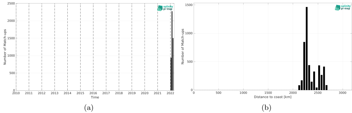
Figure 1: Number of match-ups between Saildrone and SMAP SSS L2 v5 - 40 km (RSS) SSS as a function of time (a) and as function of the distance to coast (b) over the OTT zone Pi-MEP region and for the full satellite product period.
