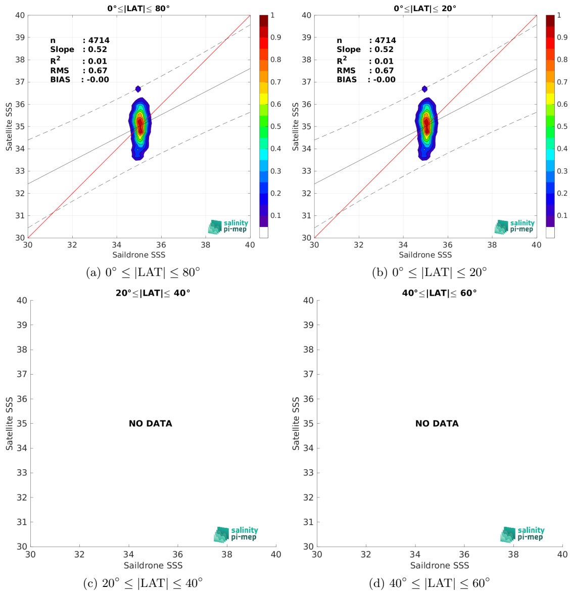
Figure 9: Contour maps of the concentration of SMAP SSS L2 v5 - 40 km (RSS) SSS (y-axis) versus Sailldrone SSS (x-axis) at match-up pairs for different latitude bands. For each plot, the red line shows x=y . The black thin and dashed lines indicate a linear fit through the data cloud and the \pm 95\% confidence levels, respectively. The number match-up pairs n , the slope and R^2 coefficient of the linear fit, the root mean square (RMS) and the mean bias between satellite and in situ data are indicated for each latitude band in each plots.
