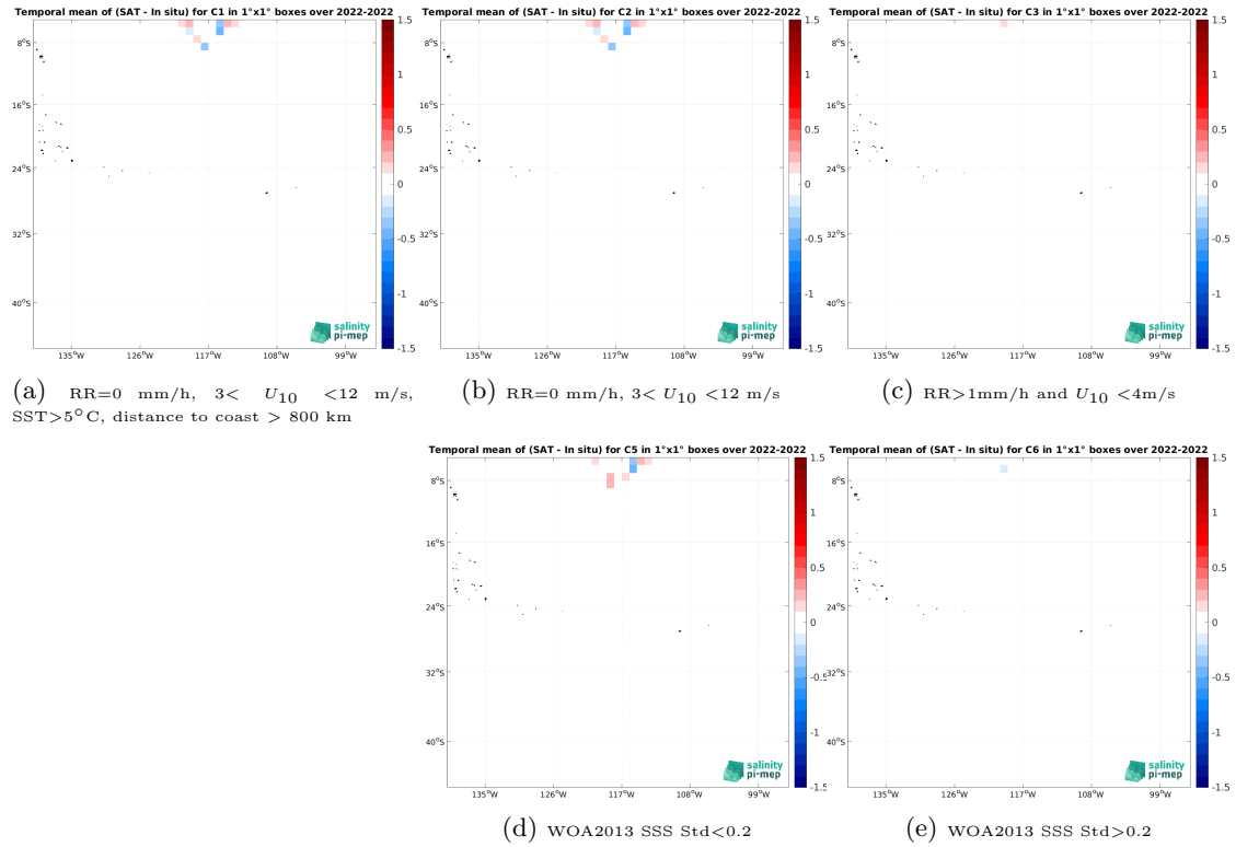
Figure 12: Temporal mean gridded over spatial boxes of size 1^\circ \times 1^\circ of \Delta SSS (SMAP SSS L2 v5 - 40 km (RSS) - Sairdrone) for 5 different subdatasets corresponding to:RR=0 mm/h, 3 < U_{10} < 12 m/s, SST >5^\circ C, distance to coast > 800 km (a), RR=0 mm/h, 3 < U_{10} < 12 m/s (b), RR >1 mm/h and U_{10} < 4 m/s (c), WOA2013 SSS Std <0.2 (d), WOA2013 SSS Std >0.2 (e).
