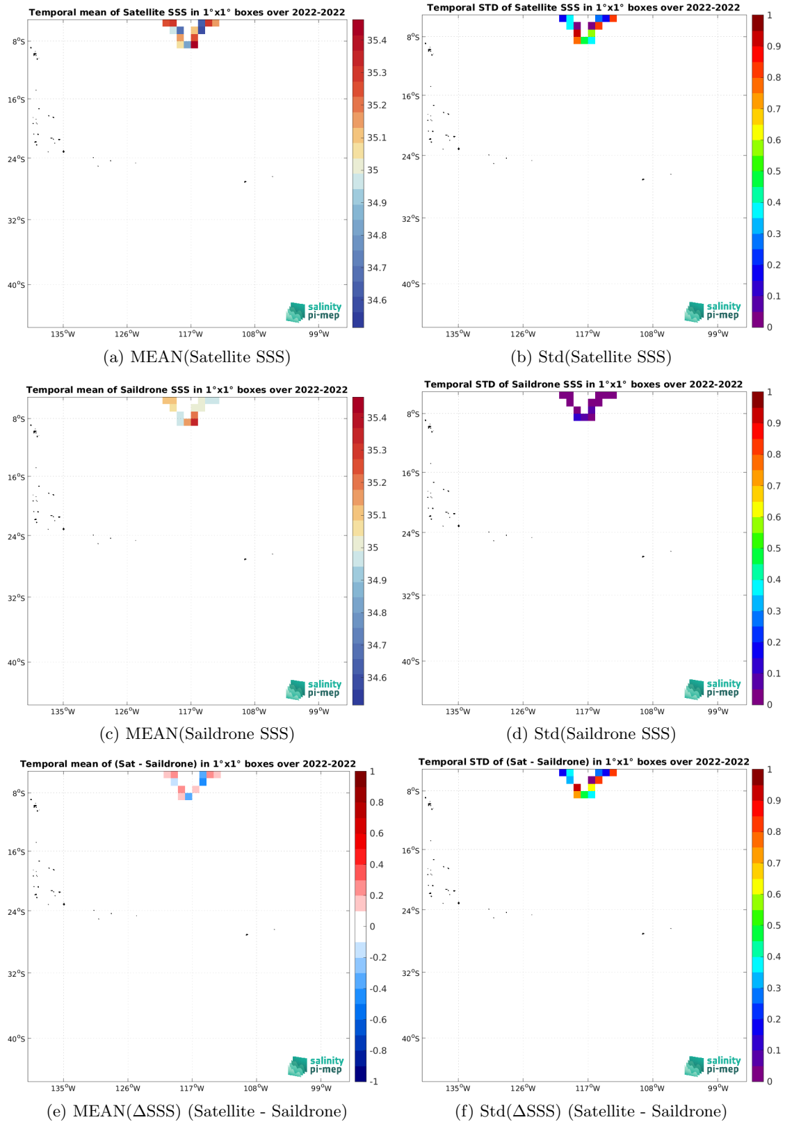
Figure 6: Temporal mean (left) and Std (right) of SSS from SMAP SSS L2 v5 - 40 km (RSS) (top), Saildrone (middle), and of \Delta SSS (Satellite - Saildrone). Only match-up pairs are used to generate these maps.
