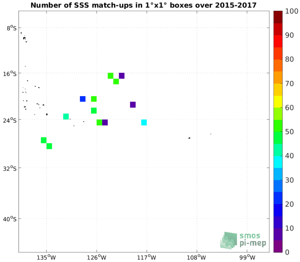
Figure 3: Number of SSS match-ups between Surface drifters SSS and the SMAP SSS L2 v5 - 40 km (RSS) SSS product for the OTT zone Pi-MEP region over 1°x1° boxes and for the full satellite product period.
