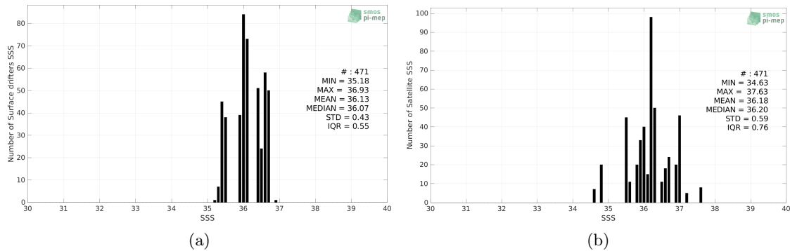
Figure 2: Histograms of SSS from Surface drifters (a) and SMAP SSS L2 v5 - 40 km (RSS) (b) considering all match-up pairs per bins of 0.1 over the OTT zone Pi-MEP region and for the full satellite product period.
