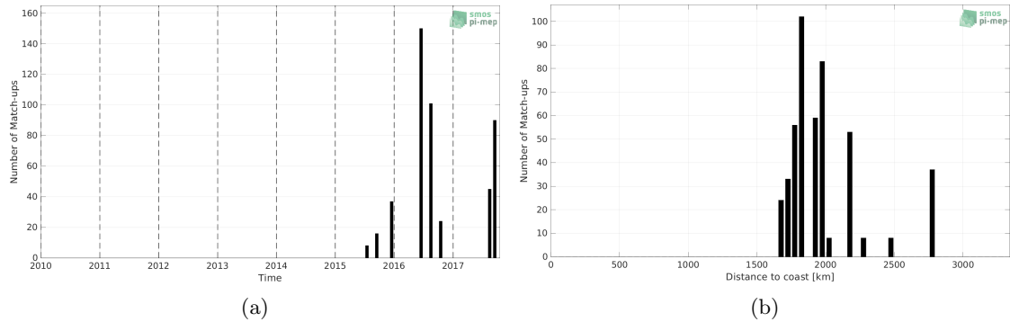
Figure 1: Number of match-ups between Surface drifters and SMAP SSS L2 v5 - 40 km (RSS) SSS as a function of time (a) and as function of the distance to coast (b) over the OTT zone Pi-MEP region and for the full satellite product period.
