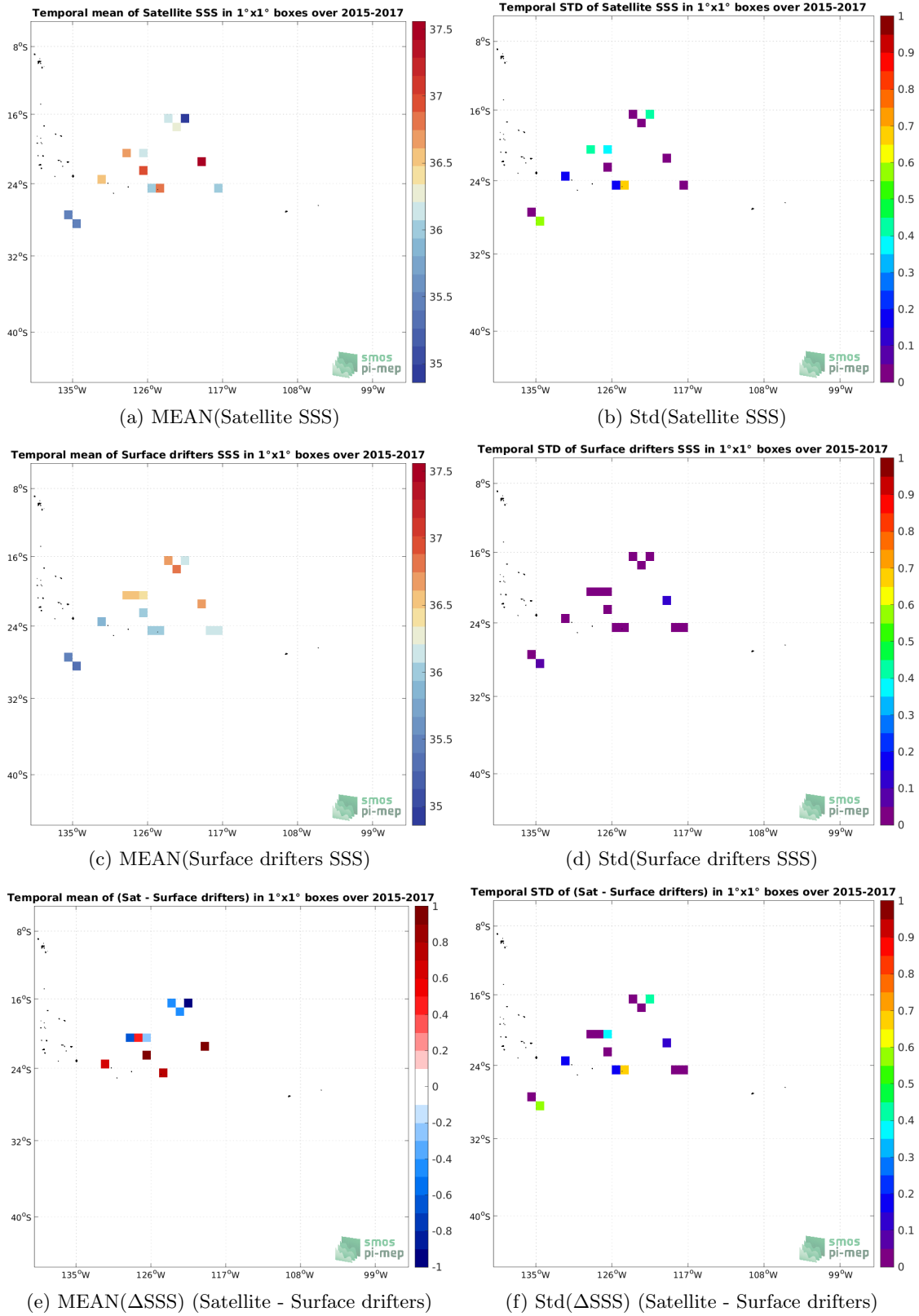
Figure 5: Temporal mean (left) and Std (right) of SSS from SMAP SSS L2 v5 - 40 km (RSS) (top), Surface drifters (middle), and of \Delta SSS (Satellite - Surface drifters). Only match-up pairs are used to generate these maps.
