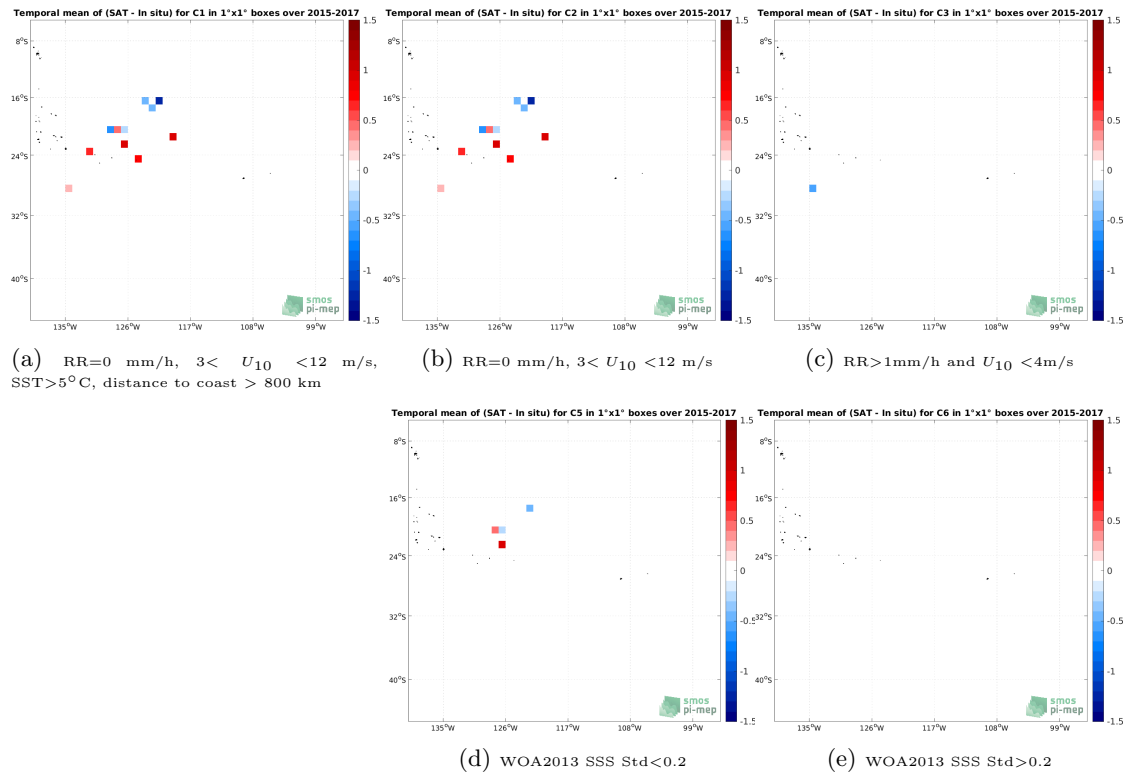
Figure 11: Temporal mean gridded over spatial boxes of size 1^\circ \times 1^\circ of \Delta SSS (SMAP SSS L2 v5 - 40 km (RSS) - Surface drifters) for 5 different subdatasets corresponding to:RR=0 mm/h, 3 < U_{10} < 12 m/s, SST > 5^\circ\text{C} , distance to coast > 800 km (a), RR=0 mm/h, 3 < U_{10} < 12 m/s (b), RR > 1 mm/h and U_{10} < 4 m/s (c), WOA2013 SSS Std < 0.2 (d), WOA2013 SSS Std > 0.2 (e).
