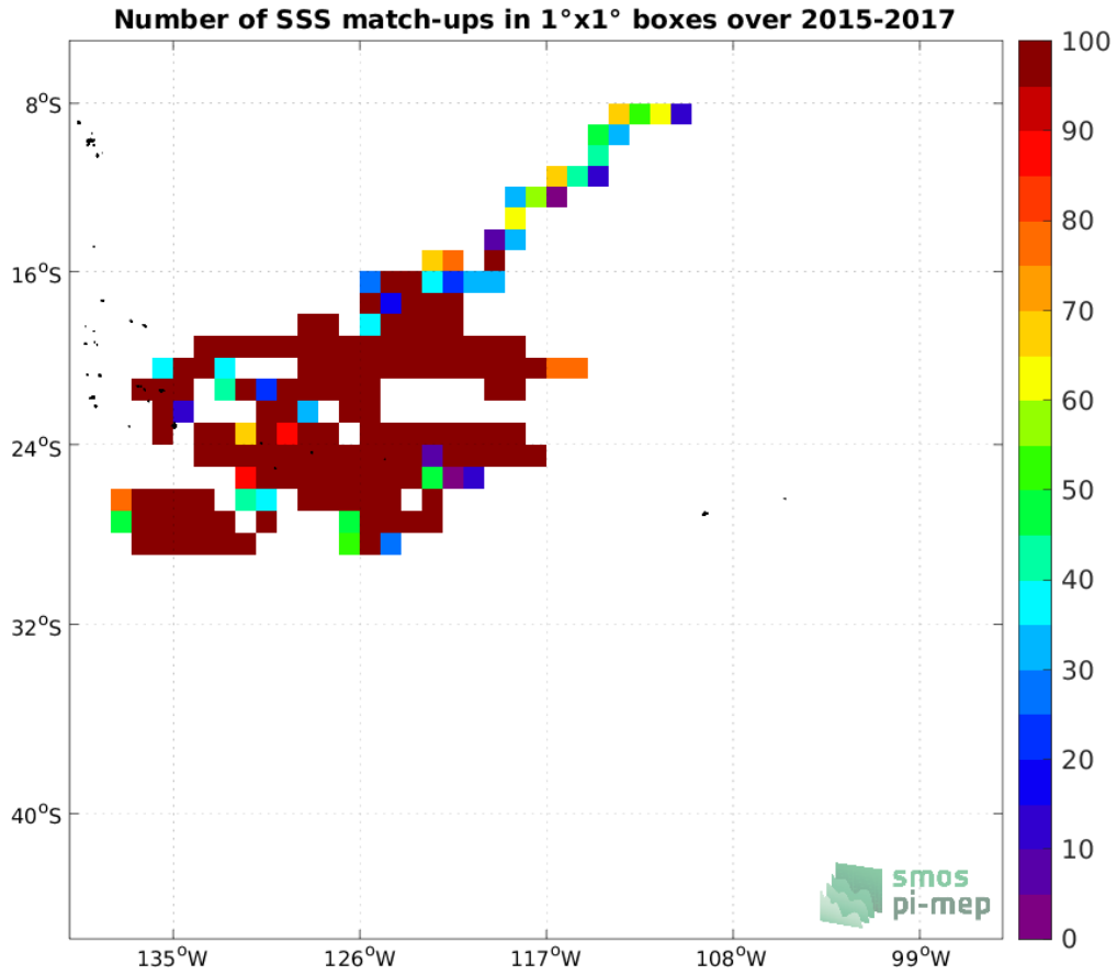
Figure 3: Number of SSS match-ups between Surface drifters SSS and the SMAP SSS L2 v5 - 40 km (RSS) SSS product for the OTT zone Pi-MEP region over 1^\circ \times 1^\circ boxes and for the full satellite product period.
