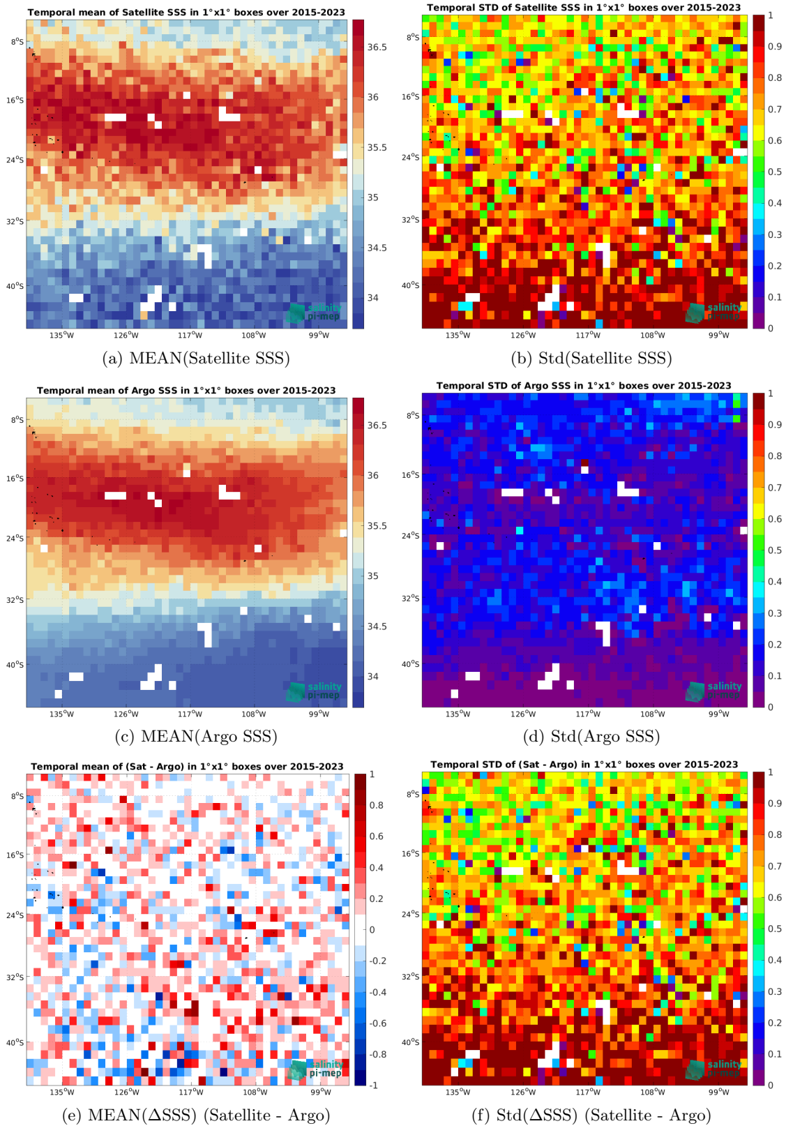
Figure 6: Temporal mean (left) and Std (right) of SSS from SMAP SSS L2 v5 - 40 km (RSS) (top), Argo (middle), and of \Delta\text{SSS} (Satellite - Argo). Only match-up pairs are used to generate these maps.
