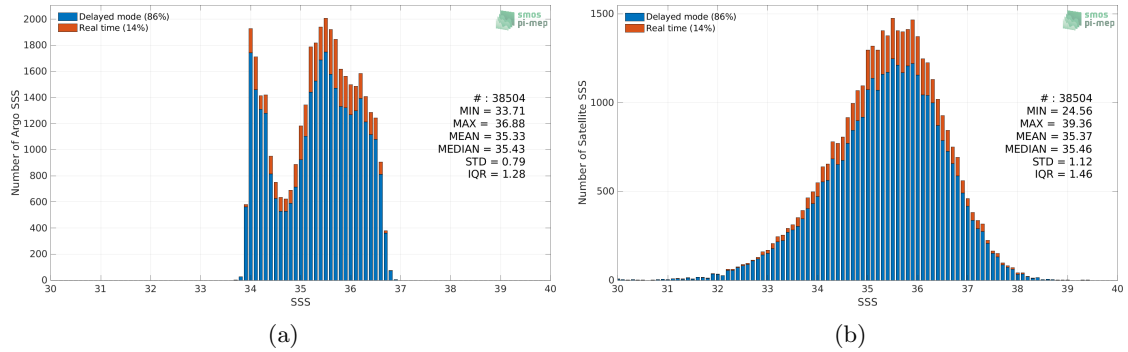
Figure 2: Histograms of SSS from Argo (a) and SMAP SSS L2 v5 - 40 km (RSS) (b) considering all match-up pairs per bins of 0.1 over the OTT zone Pi-MEP region and for the full satellite product period.
