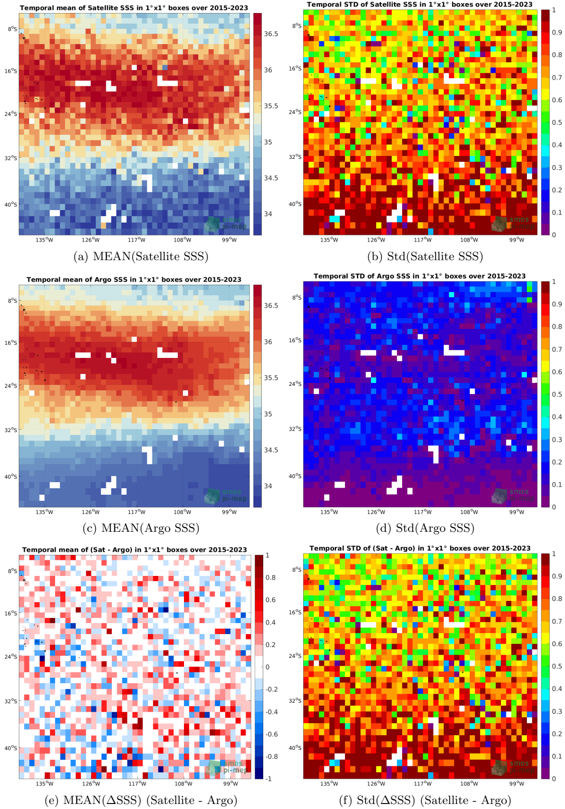
Figure 6: Temporal mean (left) and Std (right) of SSS from SMAP SSS L2 v5 - 40 km (RSS) (top), Argo (middle), and of \Delta SSS (Satellite - Argo). Only match-up pairs are used to generate these maps.
