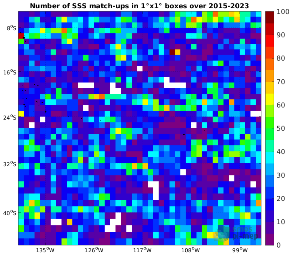
Figure 4: Number of SSS match-ups between Argo SSS and the SMAP SSS L2 v5 - 40 km (RSS) SSS product for the OTT zone Pi-MEP region over 1°×1° boxes and for the full satellite product period.
