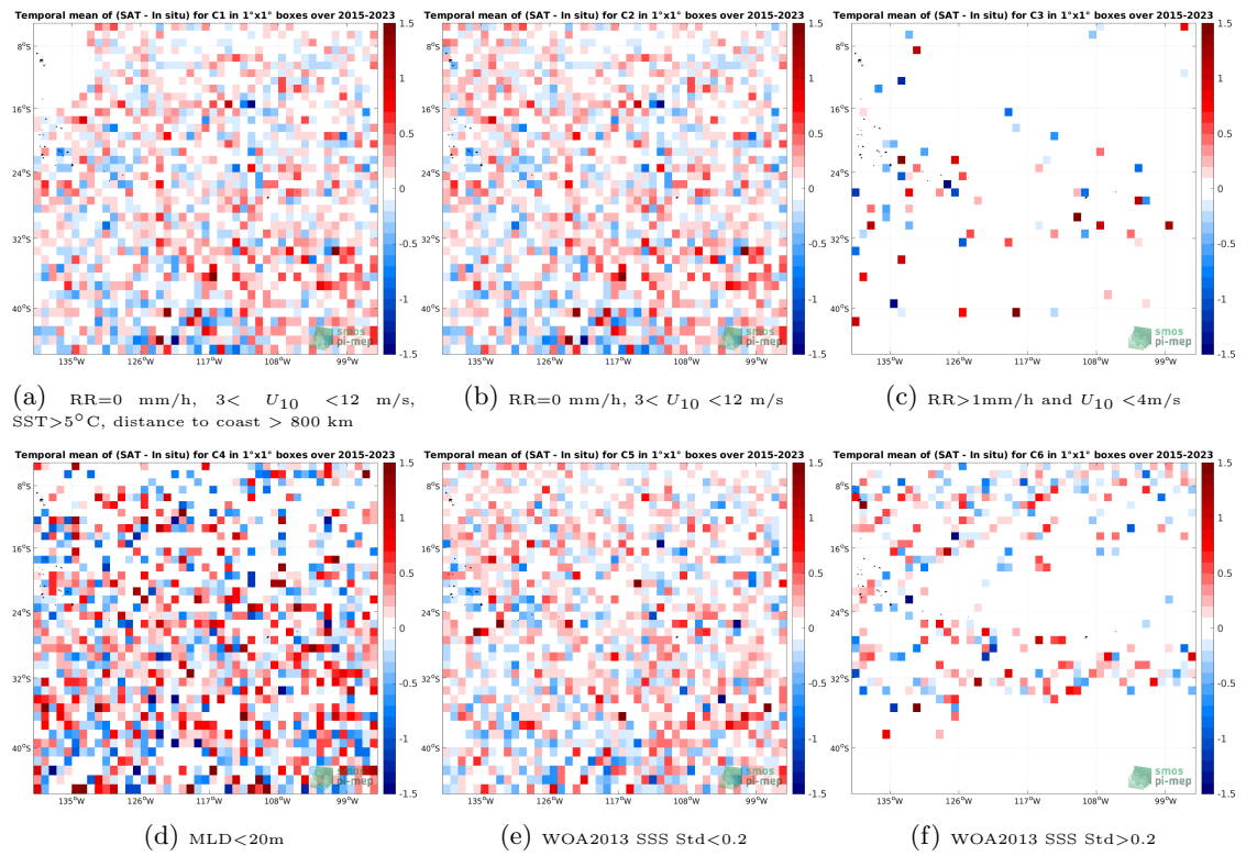
Figure 12: Temporal mean gridded over spatial boxes of size 1^\circ \times 1^\circ of \Delta SSS (SMAP SSS L2 v5 - 40 km (RSS) - Argo) for 6 different subdatasets corresponding to:RR=0 mm/h, 3 < U_{10} < 12 m/s, SST >5^\circ C, distance to coast > 800 km (a), RR=0 mm/h, 3 < U_{10} < 12 m/s (b), RR >1 mm/h and U_{10} < 4 m/s (c),MLD <20 m (d),WOA2013 SSS Std <0.2 (e),WOA2013 SSS Std >0.2 (f).
