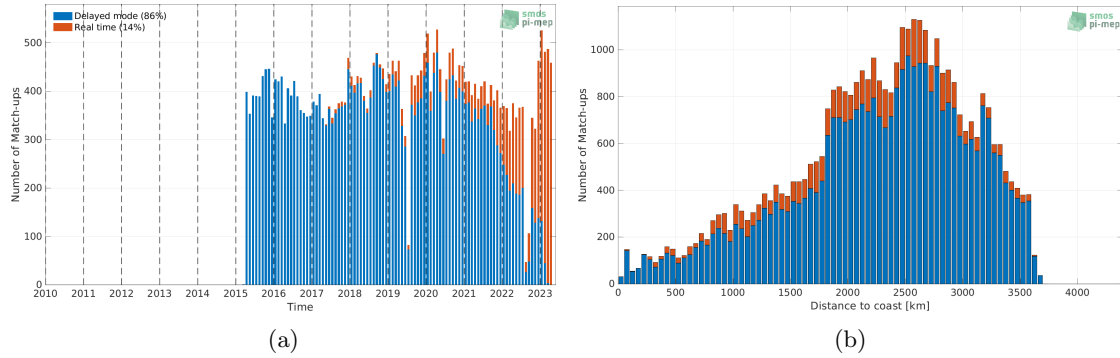
Figure 1: Number of match-ups between Argo and SMAP SSS L2 v5 - 40 km (RSS) SSS as a function of time (a) and as function of the distance to coast (b) over the OTT zone Pi-MEP region and for the full satellite product period.
