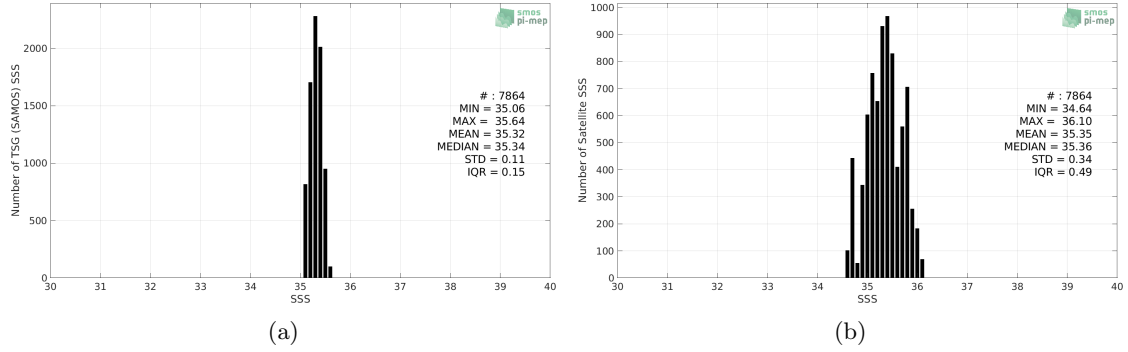
Figure 2: Histograms of SSS from TSG (SAMOS) (a) and SMAP SSS L2 v4 (RSS) (b) considering all match-up pairs per bins of 0.1 over the OTT zone Pi-MEP region and for the full satellite product period.
