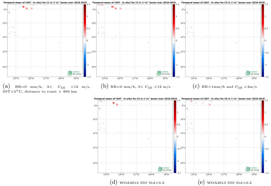
Figure 12: Temporal mean gridded over spatial boxes of size 1^\circ \times 1^\circ of \Delta SSS (SMAP SSS L2 v4 (RSS) - TSG (SAMOS)) for 5 different subdatasets corresponding to: RR=0 mm/h, 3 < U_{10} < 12 m/s, SST > 5^\circ C , distance to coast > 800 km (a), RR=0 mm/h, 3 < U_{10} < 12 m/s (b), RR > 1 mm/h and U_{10} < 4 m/s (c), WOA2013 SSS Std < 0.2 (d), WOA2013 SSS Std > 0.2 (e).
