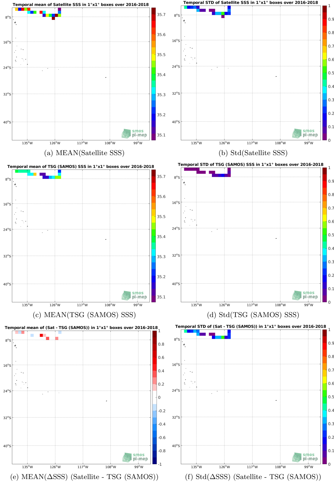
Figure 6: Temporal mean (left) and Std (right) of SSS from SMAP SSS L2 v4 (RSS) (top), TSG (SAMOS) (middle), and of \Delta SSS (Satellite - TSG (SAMOS)). Only match-up pairs are used to generate these maps.
