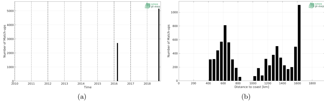
Figure 1: Number of match-ups between TSG (SAMOS) and SMAP SSS L2 v4 (RSS) SSS as a function of time (a) and as function of the distance to coast (b) over the OTT zone Pi-MEP region and for the full satellite product period.
