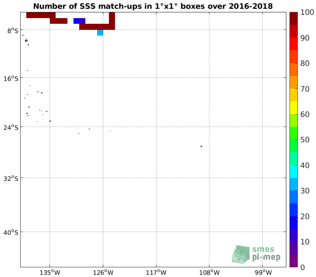
Figure 4: Number of SSS match-ups between TSG (SAMOS) SSS and the SMAP SSS L2 v4 (RSS) SSS product for the OTT zone Pi-MEP region over 1°x1° boxes and for the full satellite product period.
