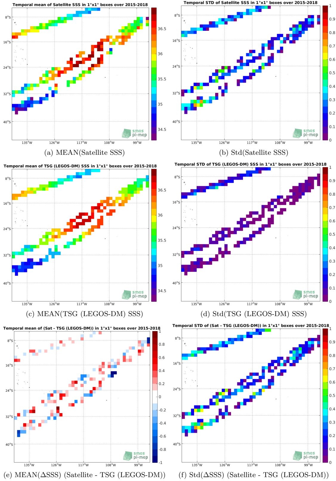
Figure 6: Temporal mean (left) and Std (right) of SSS from SMAP SSS L2 v4 (RSS) (top), TSG (LEGOS-DM) (middle), and of \Delta SSS (Satellite - TSG (LEGOS-DM)). Only match-up pairs are used to generate these maps.
