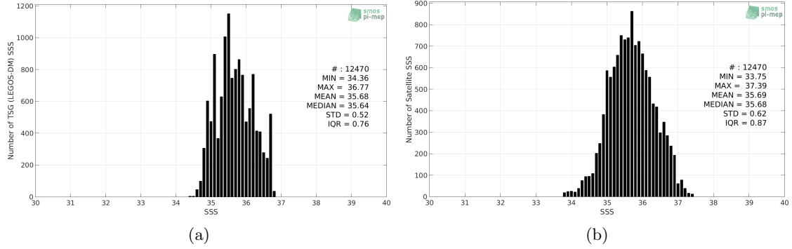
Figure 2: Histograms of SSS from TSG (LEGOS-DM) (a) and SMAP SSS L2 v4 (RSS) (b) considering all match-up pairs per bins of 0.1 over the OTT zone Pi-MEP region and for the full satellite product period.
