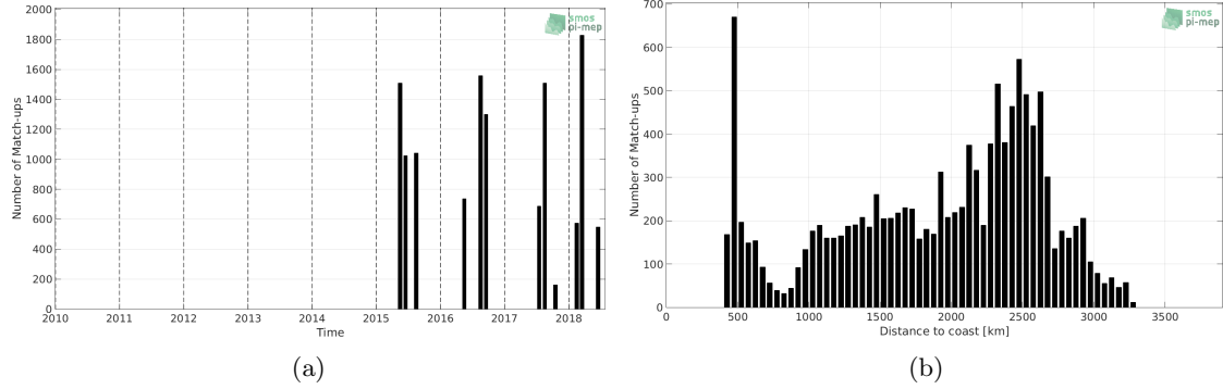
Figure 1: Number of match-ups between TSG (LEGOS-DM) and SMAP SSS L2 v4 (RSS) SSS as a function of time (a) and as function of the distance to coast (b) over the OTT zone Pi-MEP region and for the full satellite product period.
