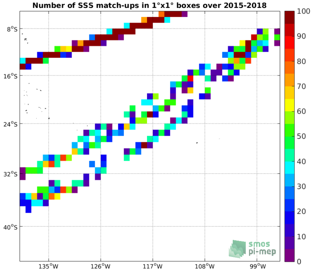
Figure 4: Number of SSS match-ups between TSG (LEGOS-DM) SSS and the SMAP SSS L2 v4 (RSS) SSS product for the OTT zone Pi-MEP region over 1°x1° boxes and for the full satellite product period.
