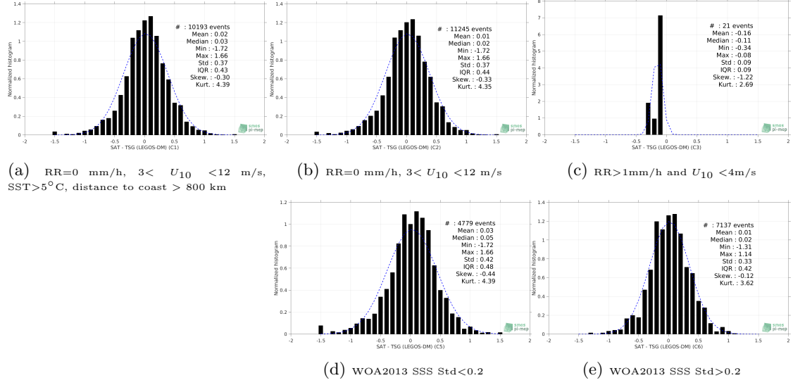
Figure 13: Normalized histogram of \Delta\text{SSS} (SMAP SSS L2 v4 (RSS) - TSG (LEGOS-DM)) for 5 different subdatasets corresponding to: RR=0 mm/h, 3 < U_{10} < 12 m/s, SST>5°C, distance to coast > 800 km (a), RR=0 mm/h, 3 < U_{10} < 12 m/s (b), RR>1mm/h and U_{10} < 4 m/s (c), WOA2013 SSS Std<0.2 (d), WOA2013 SSS Std>0.2 (e).
