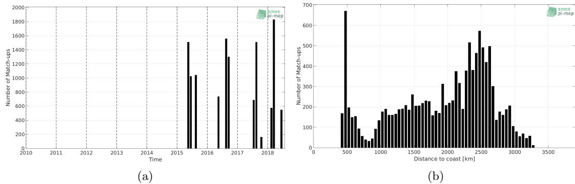
Figure 1: Number of match-ups between TSG-LEGOS-DM and SMAP-L2-RSS-V4 SSS as a function of time (a) and as function of the distance to coast (b) over the OTT zone Pi-MEP region and for the full satellite product period.
