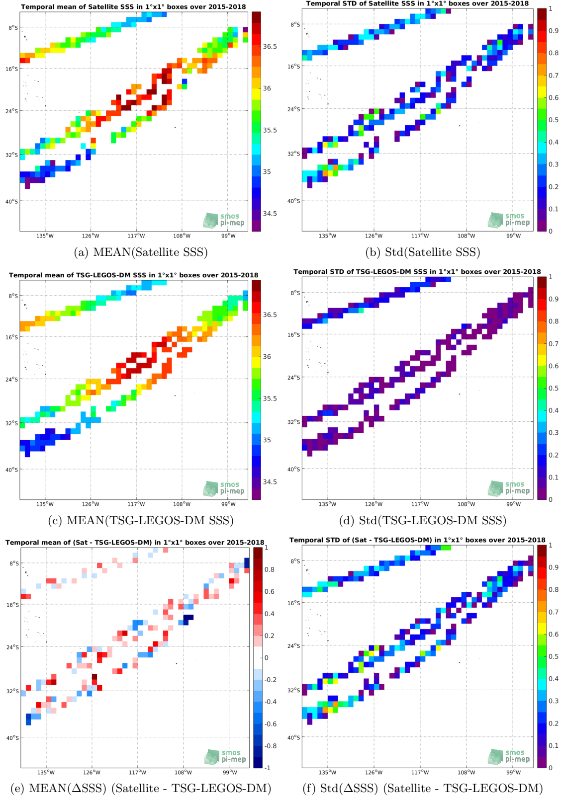
Figure 6: Temporal mean (left) and Std (right) of SSS from SMAP-L2-RSS-V4 (top), TSG-LEGOS-DM (middle), and of \Delta SSS (Satellite - TSG-LEGOS-DM). Only match-up pairs are used to generate these maps.
