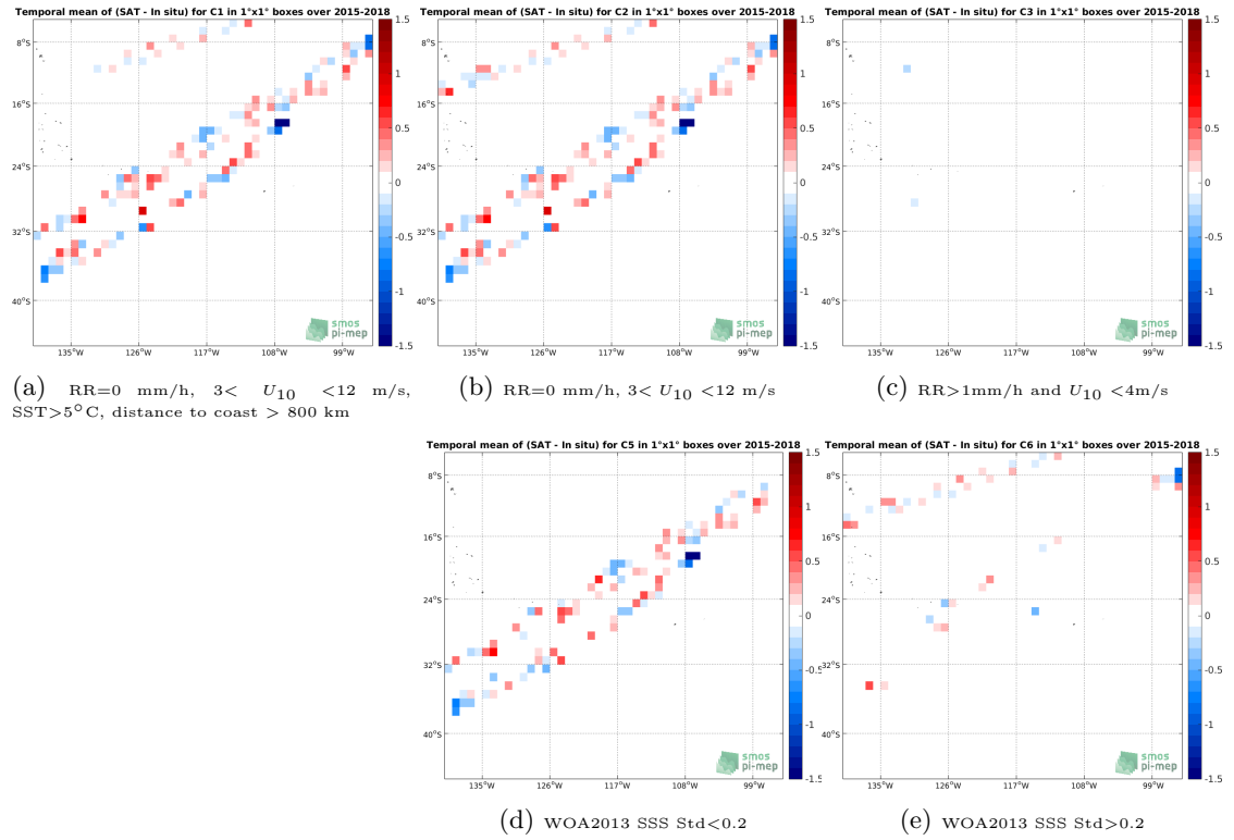
Figure 12: Temporal mean gridded over spatial boxes of size 1^\circ \times 1^\circ of \Delta SSS (SMAP-L2-RSS-V4 - TSG-LEGOS-DM) for 5 different subdatasets corresponding to: RR=0 mm/h, 3 < U_{10} < 12 m/s, SST >5^\circ\text{C} , distance to coast > 800 km (a), RR=0 mm/h, 3 < U_{10} < 12 m/s (b), RR >1 mm/h and U_{10} < 4 m/s (c), WOA2013 SSS Std <0.2 (d), WOA2013 SSS Std >0.2 (e).
