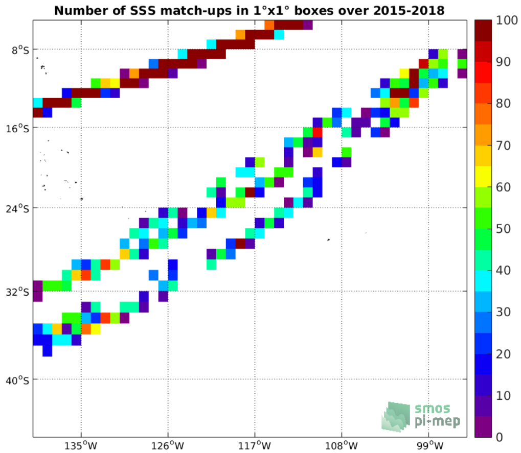
Figure 4: Number of SSS match-ups between TSG-LEGOS-DM SSS and the SMAP-L2-RSS-V4 SSS product for the OTT zone Pi-MEP region over 1°x1° boxes and for the full satellite product period.
