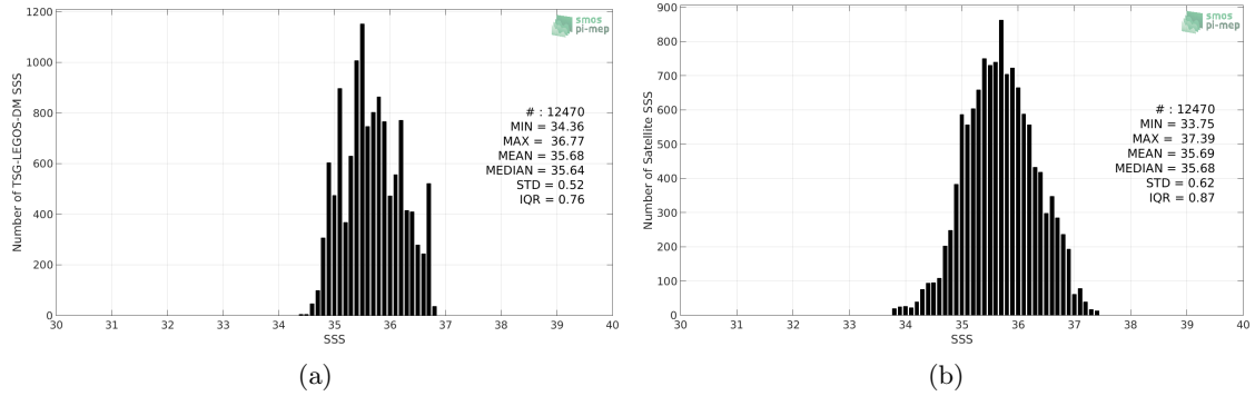
Figure 2: Histograms of SSS from TSG-LEGOS-DM (a) and SMAP-L2-RSS-V4 (b) considering all match-up pairs per bins of 0.1 over the OTT zone Pi-MEP region and for the full satellite product period.
