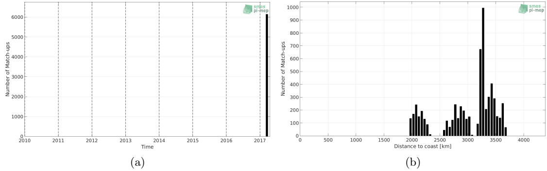
Figure 1: Number of match-ups between TSG (GOSUD-Sailing-ship) and SMAP SSS L2 v4 (RSS) SSS as a function of time (a) and as function of the distance to coast (b) over the OTT zone Pi-MEP region and for the full satellite product period.
