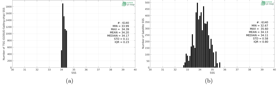
Figure 2: Histograms of SSS from TSG (GOSUD-Sailing-ship) (a) and SMAP SSS L2 v4 (RSS) (b) considering all match-up pairs per bins of 0.1 over the OTT zone Pi-MEP region and for the full satellite product period.
