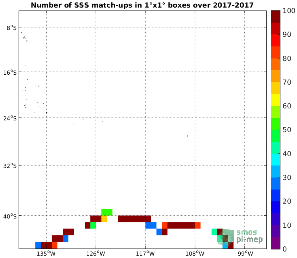
Figure 4: Number of SSS match-ups between TSG (GOSUD-Sailing-ship) SSS and the SMAP SSS L2 v4 (RSS) SSS product for the OTT zone Pi-MEP region over 1°x1° boxes and for the full satellite product period.
