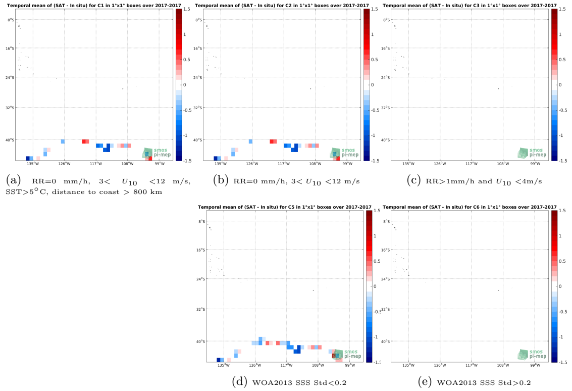
Figure 12: Temporal mean gridded over spatial boxes of size 1^\circ \times 1^\circ of \Delta SSS (SMAP SSS L2 v4 (RSS) - TSG (GOSUD-Sailing-ship)) for 5 different subdatasets corresponding to: RR=0 mm/h, 3 < U_{10} < 12 m/s, SST > 5^\circ C , distance to coast > 800 km (a), RR=0 mm/h, 3 < U_{10} < 12 m/s (b), RR > 1 mm/h and U_{10} < 4 m/s (c), WOA2013 SSS Std < 0.2 (d), WOA2013 SSS Std > 0.2 (e).
