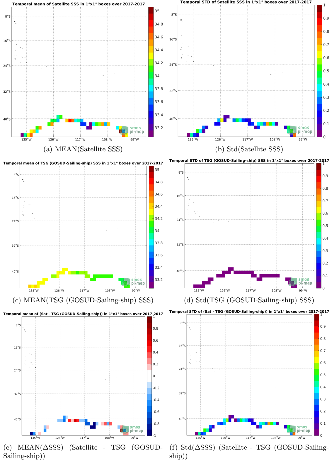
Figure 6: Temporal mean (left) and Std (right) of SSS from SMAP SSS L2 v4 (RSS) (top), TSG (GOSUD-Sailing-ship) (middle), and of \Delta SSS (Satellite - TSG (GOSUD-Sailing-ship)). Only match-up pairs are used to generate these maps.
