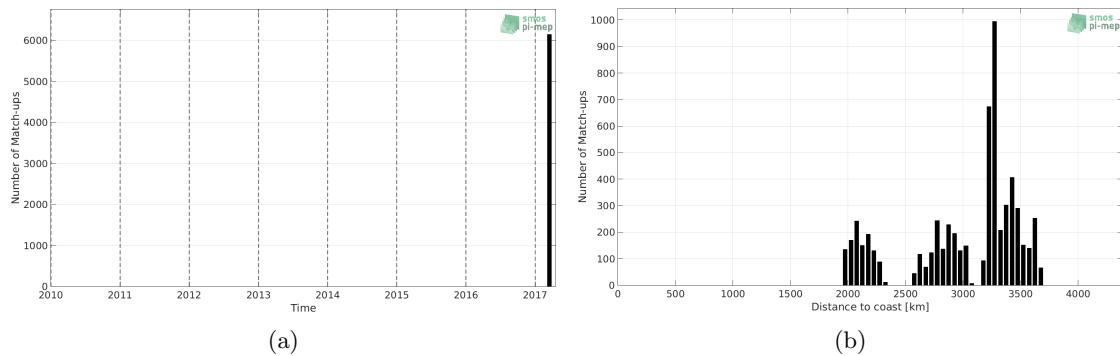
Figure 1: Number of match-ups between TSG-GOSUD-Sailing-ship and SMAP-L2-RSS-V4 SSS as a function of time (a) and as function of the distance to coast (b) over the OTT zone Pi-MEP region and for the full satellite product period.
