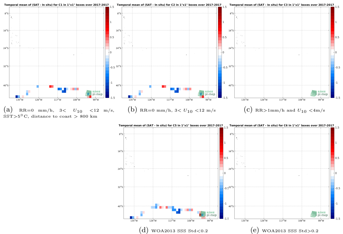
Figure 12: Temporal mean gridded over spatial boxes of size 1^\circ \times 1^\circ of \Delta SSS (SMAP-L2-RSS-V4 - TSG-GOSUD-Sailing-ship) for 5 different subdatasets corresponding to:RR=0 mm/h, 3 < U_{10} < 12 m/s, SST >5^\circ C, distance to coast > 800 km (a), RR=0 mm/h, 3 < U_{10} < 12 m/s (b), RR >1 mm/h and U_{10} < 4 m/s (c), WOA2013 SSS Std <0.2 (d), WOA2013 SSS Std >0.2 (e).
