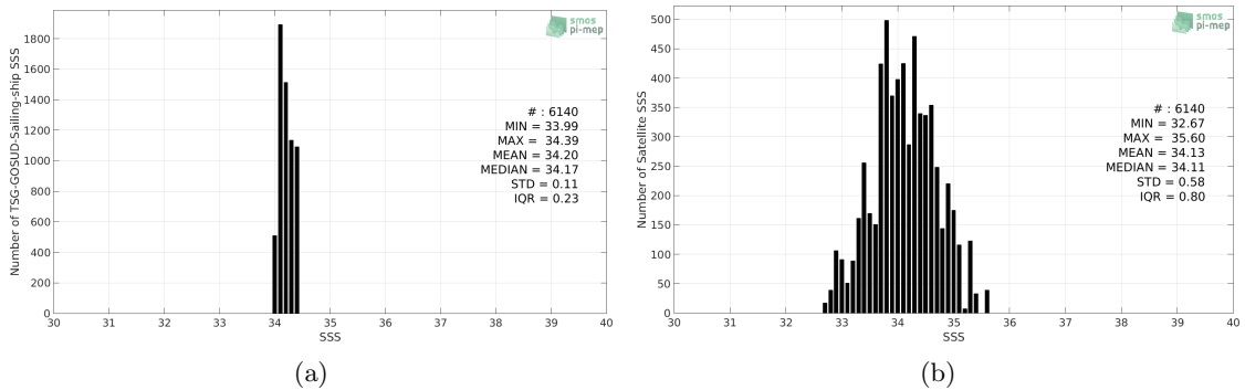
Figure 2: Histograms of SSS from TSG-GOSUD-Sailing-ship (a) and SMAP-L2-RSS-V4 (b) considering all match-up pairs per bins of 0.1 over the OTT zone Pi-MEP region and for the full satellite product period.
