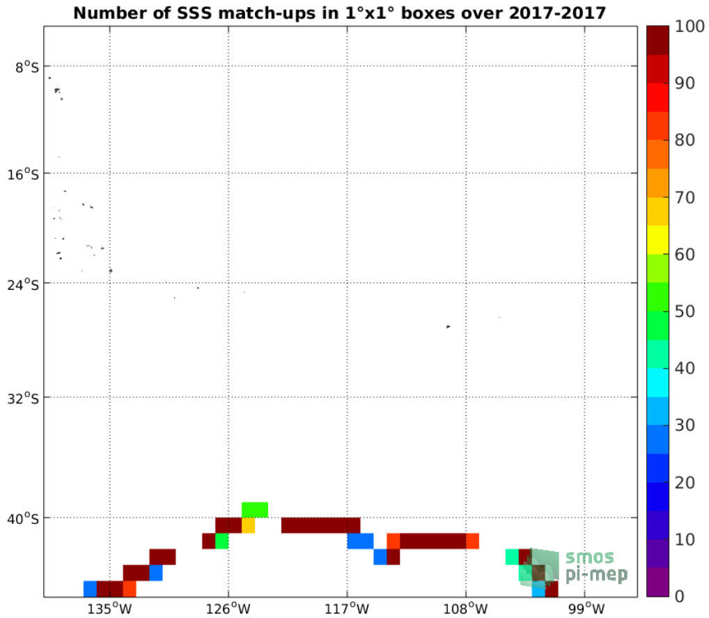
Figure 4: Number of SSS match-ups between TSG-GOSUD-Sailing-ship SSS and the SMAP-L2-RSS-V4 SSS product for the OTT zone Pi-MEP region over 1°x1° boxes and for the full satellite product period.
