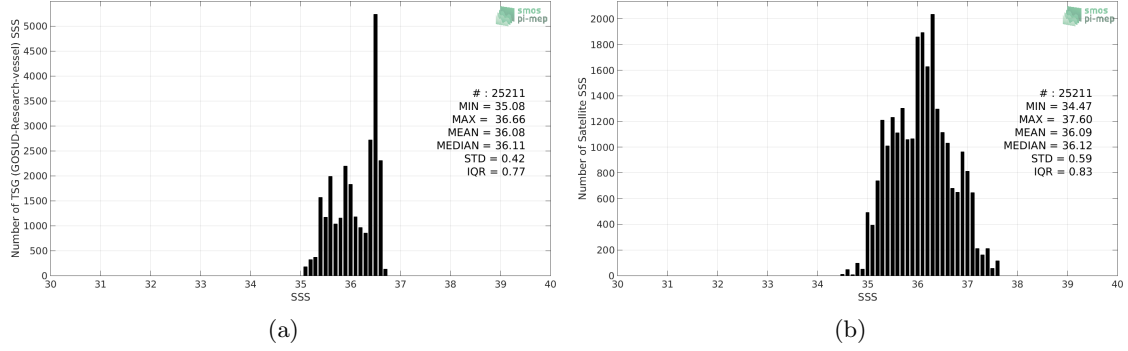
Figure 2: Histograms of SSS from TSG (GOSUD-Research-vessel) (a) and SMAP SSS L2 v4 (RSS) (b) considering all match-up pairs per bins of 0.1 over the OTT zone Pi-MEP region and for the full satellite product period.
