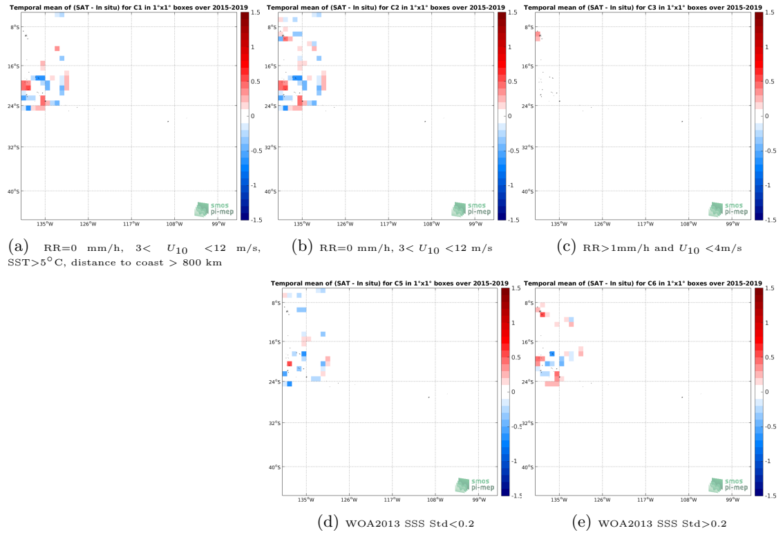
Figure 12: Temporal mean gridded over spatial boxes of size 1^\circ \times 1^\circ of \Delta SSS (SMAP SSS L2 v4 (RSS) - TSG (GOSUD-Research-vessel)) for 5 different subdatasets corresponding to: RR=0 mm/h, 3 < U_{10} < 12 m/s, SST > 5^\circ C , distance to coast > 800 km (a), RR=0 mm/h, 3 < U_{10} < 12 m/s (b), RR > 1 mm/h and U_{10} < 4 m/s (c), WOA2013 SSS Std < 0.2 (d), WOA2013 SSS Std > 0.2 (e).
