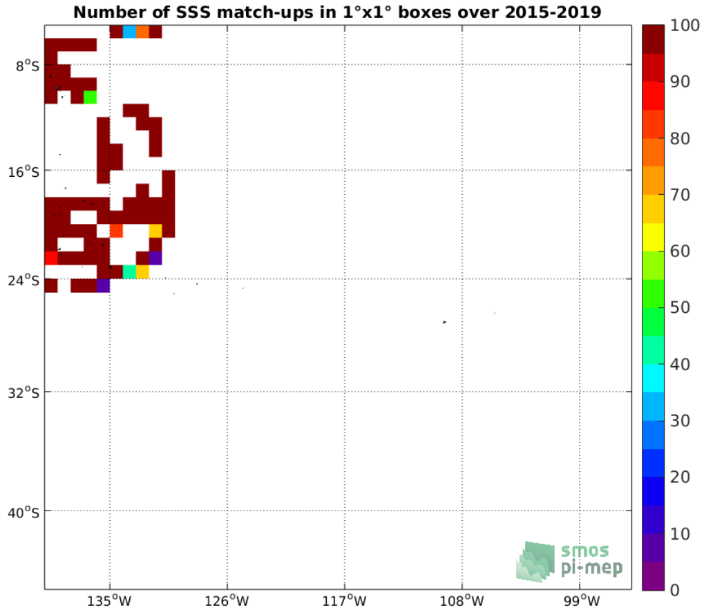
Figure 4: Number of SSS match-ups between TSG (GOSUD-Research-vessel) SSS and the SMAP SSS L2 v4 (RSS) SSS product for the OTT zone Pi-MEP region over 1°x1° boxes and for the full satellite product period.
