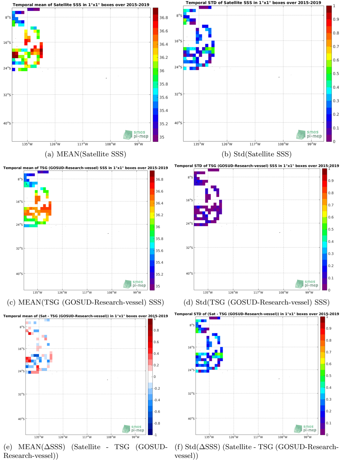
Figure 6: Temporal mean (left) and Std (right) of SSS from SMAP SSS L2 v4 (RSS) (top), TSG (GOSUD-Research-vessel) (middle), and of \Delta SSS (Satellite - TSG (GOSUD-Research-vessel)). Only match-up pairs are used to generate these maps.
