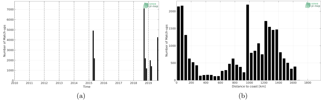
Figure 1: Number of match-ups between TSG (GOSUD-Research-vessel) and SMAP SSS L2 v4 (RSS) SSS as a function of time (a) and as function of the distance to coast (b) over the OTT zone Pi-MEP region and for the full satellite product period.
