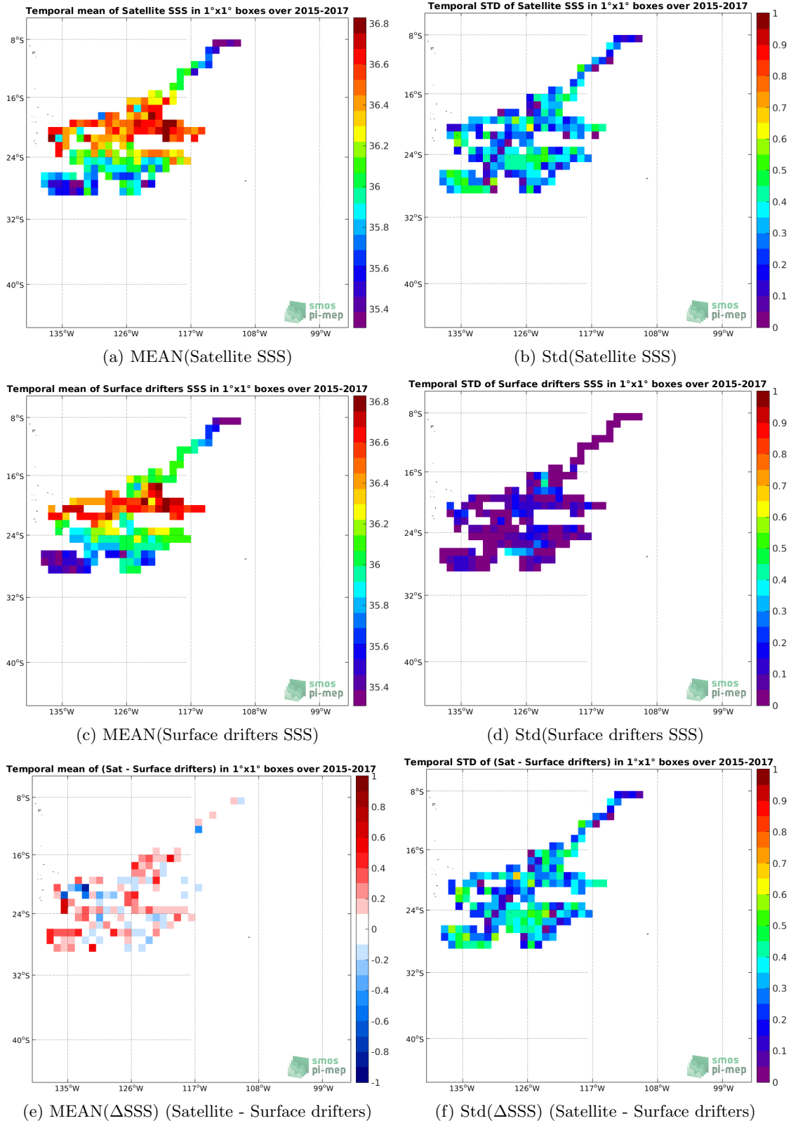
Figure 5: Temporal mean (left) and Std (right) of SSS from SMAP SSS L2 v4 (RSS), Surface drifters (middle), and of \Delta SSS (Satellite - Surface drifters). Only match-up pairs are used to generate these maps.
