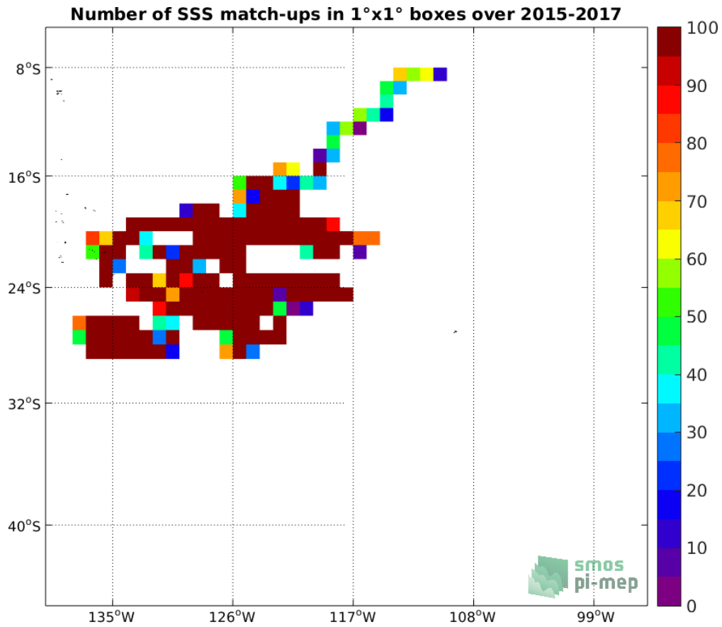
Figure 3: Number of SSS match-ups between Surface drifters SSS and the SMAP SSS L2 v4 (RSS) SSS product for the OTT zone Pi-MEP region over 1°×1° boxes and for the full satellite product period.
