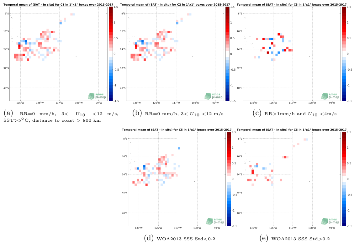
Figure 11: Temporal mean gridded over spatial boxes of size 1^\circ \times 1^\circ of \Delta\text{SSS} (SMAP SSS L2 v4 (RSS) - Surface drifters) for 5 different subdatasets corresponding to:RR=0 mm/h, 3 < U_{10} < 12 m/s, SST >5^\circ\text{C} , distance to coast > 800 km (a), RR=0 mm/h, 3 < U_{10} < 12 m/s (b), RR >1 mm/h and U_{10} < 4 m/s (c), WOA2013 SSS Std <0.2 (d), WOA2013 SSS Std >0.2 (e).
