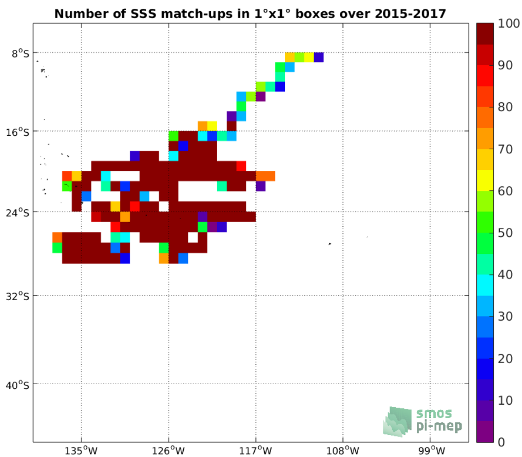
Figure 3: Number of SSS match-ups between Surface drifters SSS and the SMAP-L2-RSS-V4 SSS product for the OTT zone Pi-MEP region over 1°x1° boxes and for the full satellite product period.
