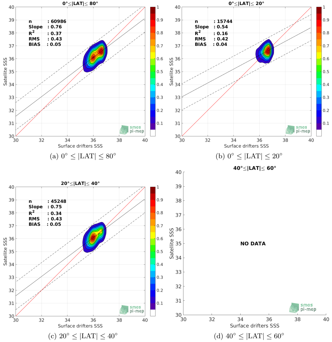
Figure 8: Contour maps of the concentration of SMAP-L2-RSS-V4 SSS (y-axis) versus Surface drifters SSS (x-axis) at match-up pairs for different latitude bands. For each plot, the red line shows x=y . The black thin and dashed lines indicate a linear fit through the data cloud and the \pm 95\% confidence levels, respectively. The number match-up pairs n , the slope and R^2 coefficient of the linear fit, the root mean square (RMS) and the mean bias between satellite and in situ data are indicated for each latitude band in each plots.
