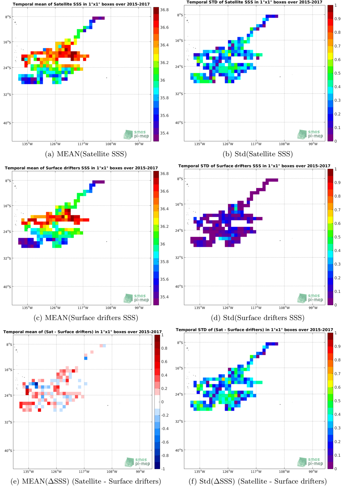
Figure 5: Temporal mean (left) and Std (right) of SSS from SMAP-L2-RSS-V4 (top), Surface drifters (middle), and of \Delta SSS (Satellite - Surface drifters). Only match-up pairs are used to generate these maps.
