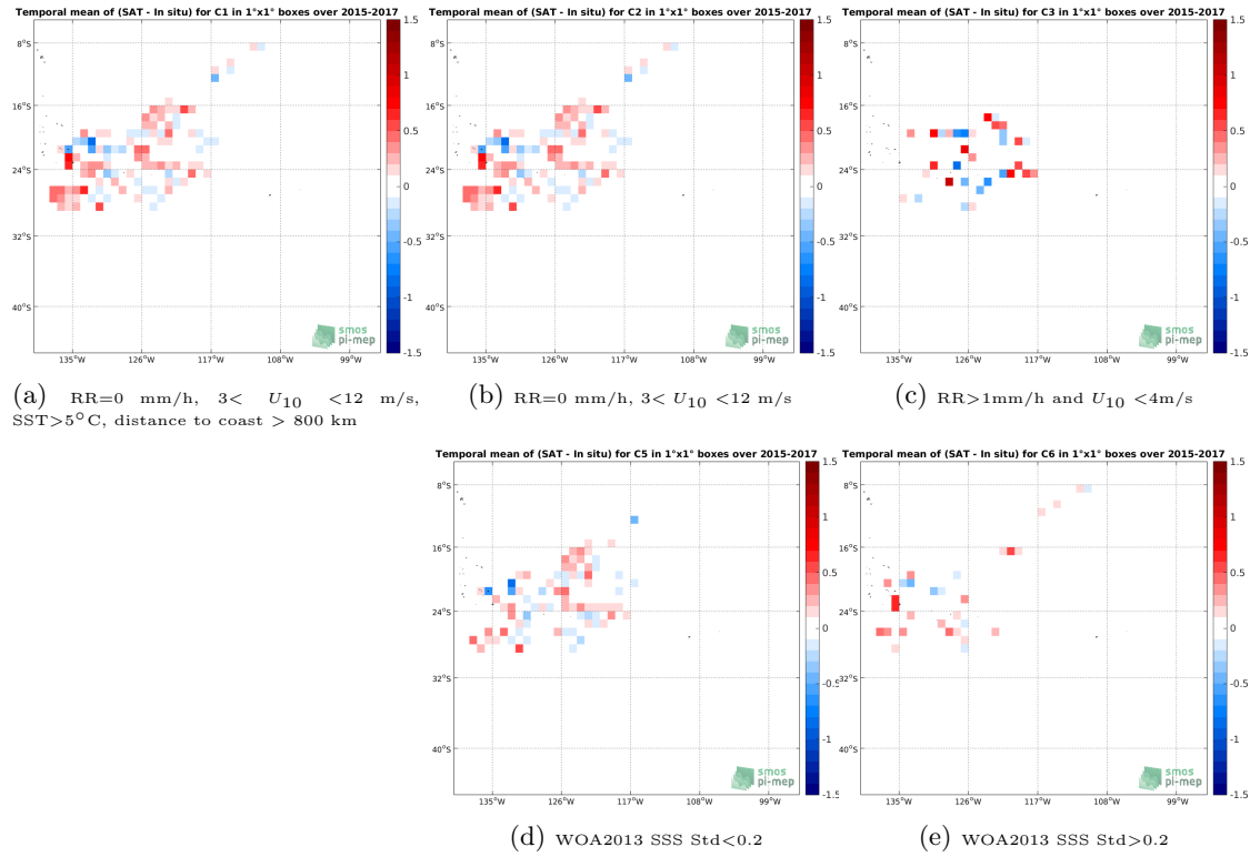
Figure 11: Temporal mean gridded over spatial boxes of size 1^\circ \times 1^\circ of \Delta SSS (SMAP-L2-RSS-V4 - Surface drifters) for 5 different subdatasets corresponding to:RR=0 mm/h, 3 < U_{10} < 12 m/s, SST >5^\circ C, distance to coast > 800 km (a), RR=0 mm/h, 3 < U_{10} < 12 m/s (b), RR >1 mm/h and U_{10} < 4 m/s (c), WOA2013 SSS Std <0.2 (d), WOA2013 SSS Std >0.2 (e).
