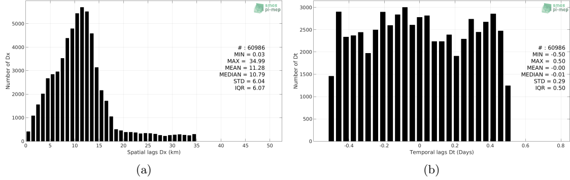
Figure 4: Histograms of the spatial (a) and temporal (b) lags between the time of the Surface drifters measurements and the date of the corresponding SMAP-L2-RSS-V4 SSS product.
