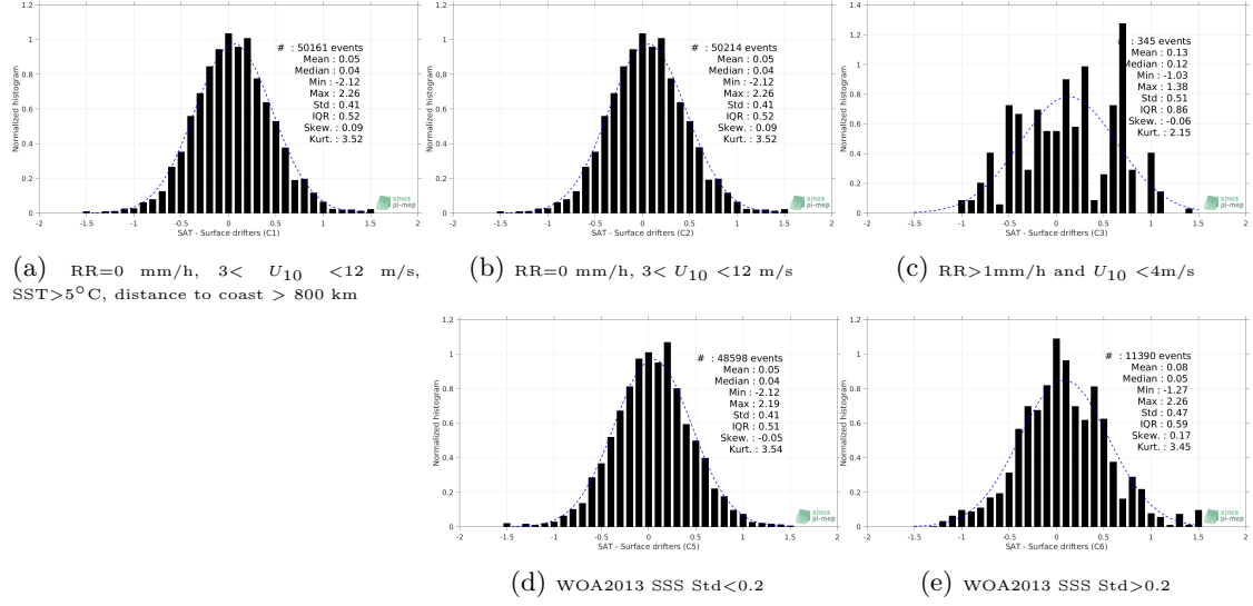
Figure 12: Normalized histogram of \Delta SSS (SMAP-L2-RSS-V4 - Surface drifters) for 5 different subdatasets corresponding to: RR=0 mm/h, 3 < U_{10} < 12 m/s, SST > 5°C, distance to coast > 800 km (a), RR=0 mm/h, 3 < U_{10} < 12 m/s (b), RR > 1mm/h and U_{10} < 4 m/s (c), WOA2013 SSS Std < 0.2 (d), WOA2013 SSS Std > 0.2 (e).
