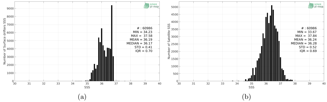
Figure 2: Histograms of SSS from Surface drifters (a) and SMAP-L2-RSS-V4 (b) considering all match-up pairs per bins of 0.1 over the OTT zone Pi-MEP region and for the full satellite product period.
