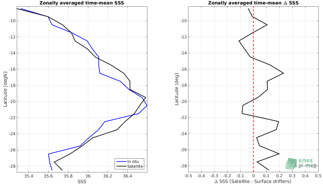
Figure 7: Left panel: Zonal mean SSS from SMAP-L2-RSS-V4 satellite product (black) and from Surface drifters (blue). Right panel: Zonal mean of \Delta SSS (Satellite - Surface drifters) for all the collected Pi-MEP match-up pairs estimated over the full satellite product period.
