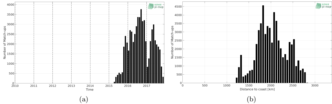
Figure 1: Number of match-ups between Surface drifters and SMAP-L2-RSS-V4 SSS as a function of time (a) and as function of the distance to coast (b) over the OTT zone Pi-MEP region and for the full satellite product period.
