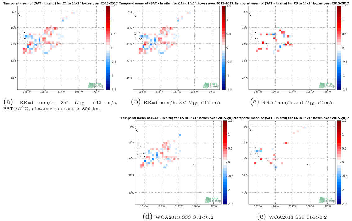
Figure 11: Temporal mean gridded over spatial boxes of size 1^\circ \times 1^\circ of \Delta SSS (SMAP-L2-RSS-V4 - Surface drifters) for 5 different subdatasets corresponding to: RR=0 mm/h, 3 < U_{10} < 12 m/s, SST > 5^\circ\text{C} , distance to coast > 800 km (a), RR=0 mm/h, 3 < U_{10} < 12 m/s (b), RR > 1 mm/h and U_{10} < 4 m/s (c), WOA2013 SSS Std < 0.2 (d), WOA2013 SSS Std > 0.2 (e).
