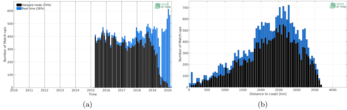
Figure 1: Number of match-ups between Argo and SMAP-L2-RSS-V4 SSS as a function of time (a) and as function of the distance to coast (b) over the OTT zone Pi-MEP region and for the full satellite product period.
