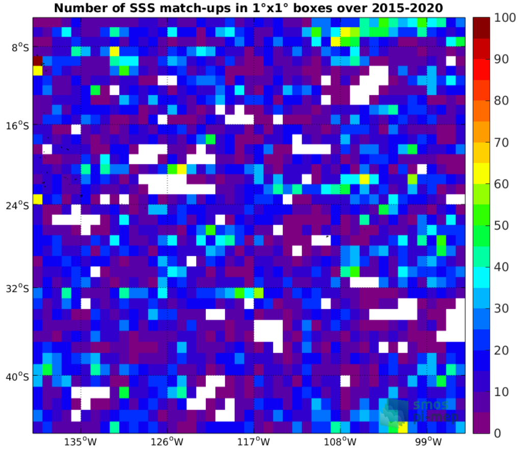
Figure 4: Number of SSS match-ups between Argo SSS and the SMAP-L2-RSS-V4 SSS product for the OTT zone Pi-MEP region over 1°x1° boxes and for the full satellite product period.
