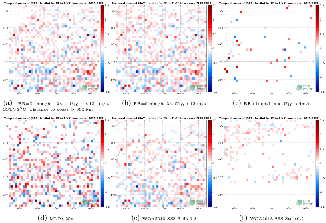
Figure 12: Temporal mean gridded over spatial boxes of size 1^\circ \times 1^\circ of \Delta SSS (SMAP-L2-RSS-V4 - Argo) for 6 different subdatasets corresponding to: RR=0 mm/h, 3 < U_{10} < 12 m/s, SST >5^\circ C, distance to coast > 800 km (a), RR=0 mm/h, 3 < U_{10} < 12 m/s (b), RR >1 mm/h and U_{10} < 4 m/s (c),MLD <20 m (d),WOA2013 SSS Std <0.2 (e),WOA2013 SSS Std >0.2 (f).
