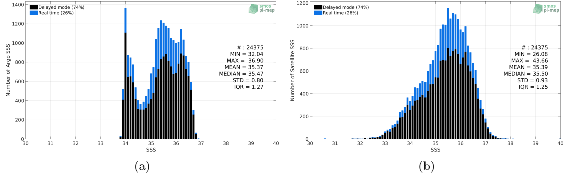
Figure 2: Histograms of SSS from Argo (a) and SMAP-L2-RSS-V4 (b) considering all match-up pairs per bins of 0.1 over the OTT zone Pi-MEP region and for the full satellite product period.
