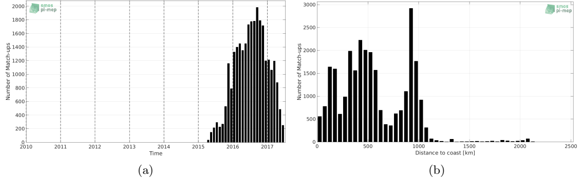
Figure 1: Number of match-ups between Surface drifters and SMAP-L2-RSS-V3-70KM SSS as a function of time (a) and as function of the distance to coast (b) over the OTT zone Pi-MEP region and for the full satellite product period.
