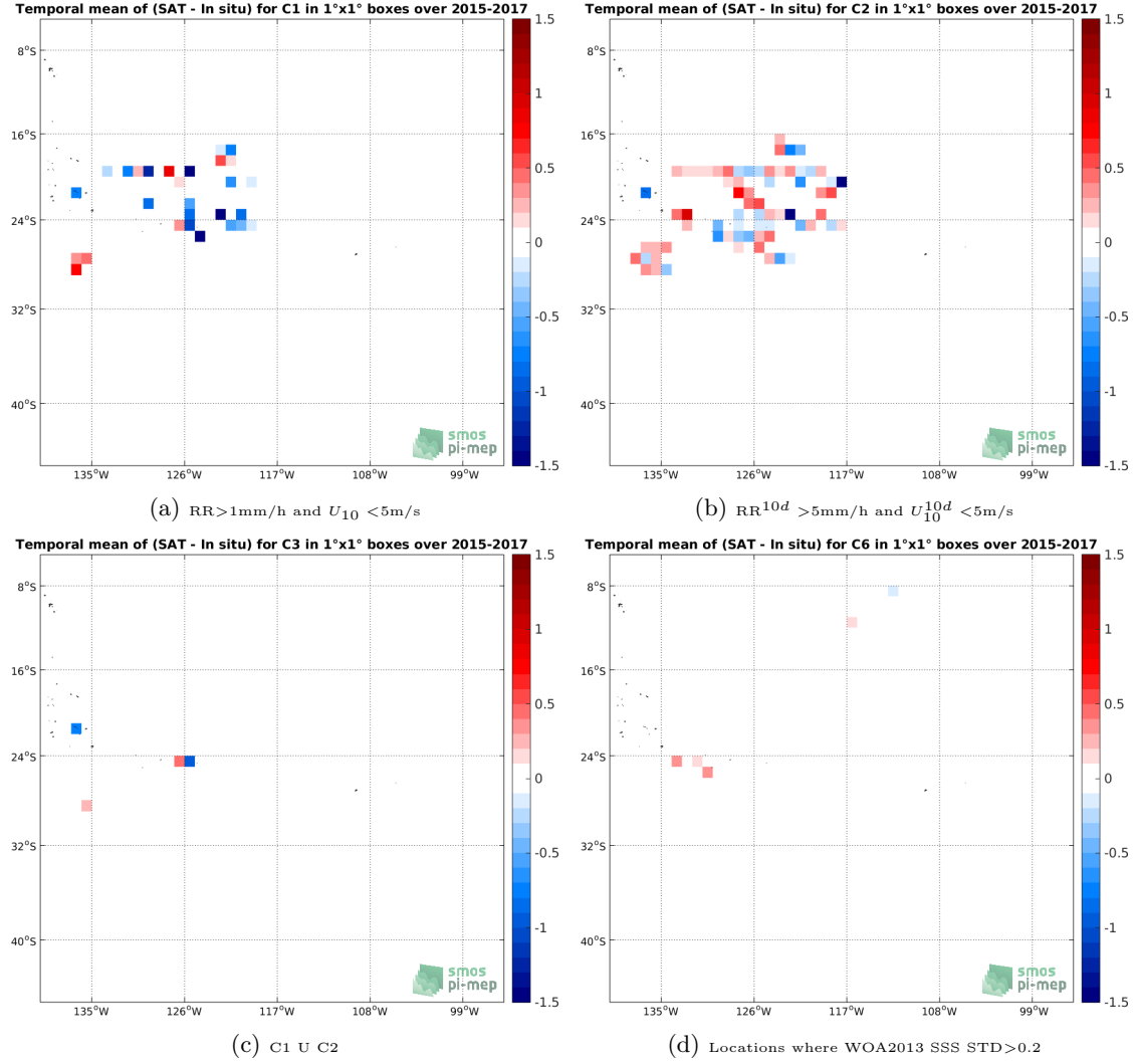
Figure 11: Temporal mean gridded over spatial boxes of size 1^\circ \times 1^\circ of \Delta SSS (SMAP-L2-RSS-V3-70KM - Surface drifters) for 4 different subdatasets corresponding to: RR > 1\text{mm/h} and U_{10} < 5\text{m/s} (a), RR^{10d} > 5\text{mm/h} and U_{10}^{10d} < 5\text{m/s} (b), C1 U C2 (c), Locations where WOA2013 SSS STD > 0.2 (d).
