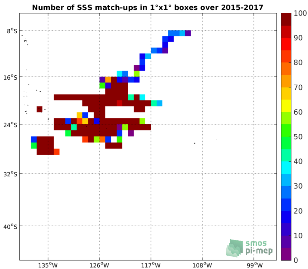
Figure 3: Number of SSS match-ups between Surface drifters SSS and the SMAP-L2-RSS-V3-70KM SSS product for the OTT zone Pi-MEP region over 1°x1° boxes and for the full satellite product period.
