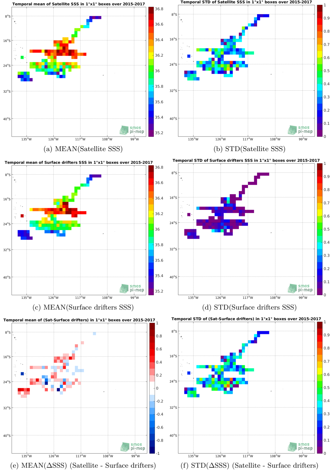
Figure 5: Temporal mean (left) and STD (right) of SSS from SMAP-L2-RSS-V3-70KM (top), Surface drifters (middle), and of \Delta SSS (Satellite - Surface drifters). Only match-up pairs are used to generate these maps.
