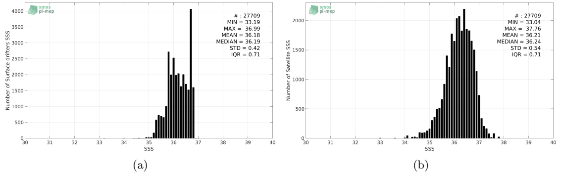
Figure 2: Histograms of SSS from Surface drifters (a) and SMAP-L2-RSS-V3-70KM (b) considering all match-up pairs per bins of 0.1 over the OTT zone Pi-MEP region and for the full satellite product period.
