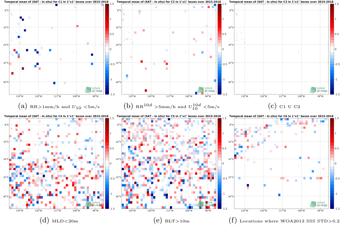
Figure 12: Temporal mean gridded over spatial boxes of size 1^\circ \times 1^\circ of \Delta\text{SSS} (SMAP-L2-RSS-V3-70KM - Argo) for 6 different subdatasets corresponding to: RR > 1mm/h and U_{10} < 5\text{m/s} (a), \text{RR}^{10d} > 5\text{mm/h} and U_{10}^{10d} < 5\text{m/s} (b), C1 U C2 (c), MLD < 20m (d), BLT > 10m (e), Locations where WOA2013 SSS STD > 0.2 (f).
