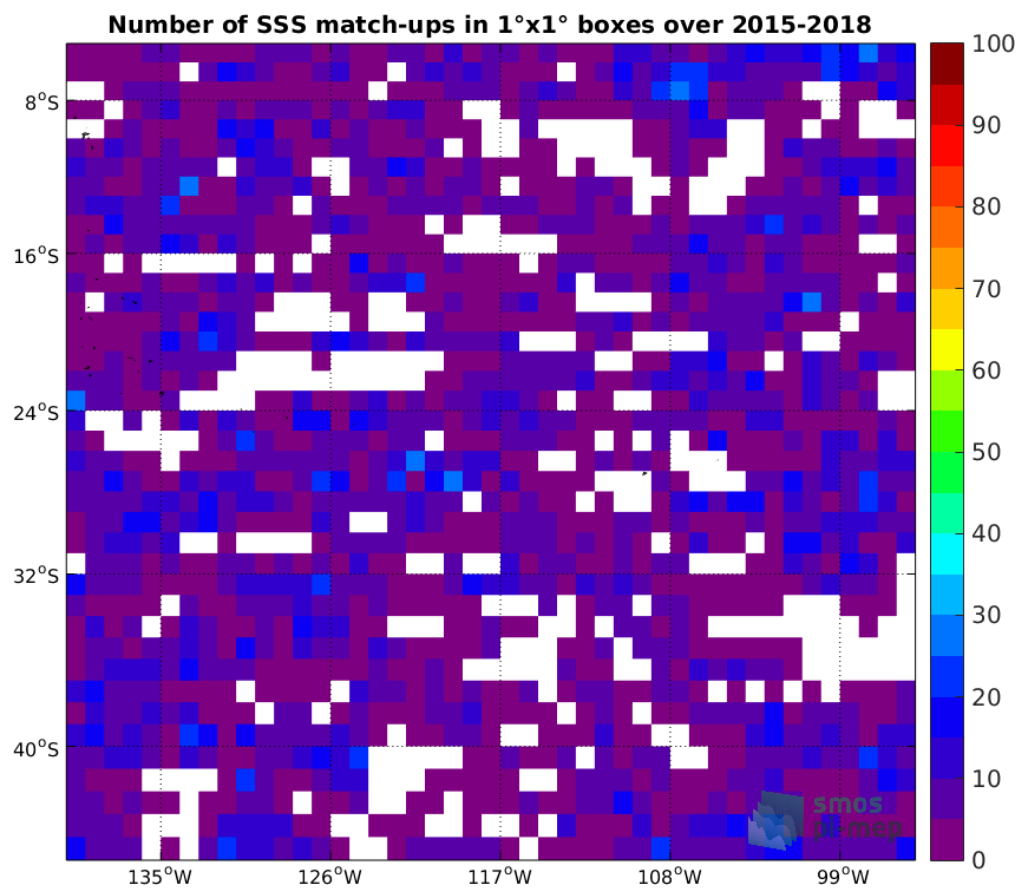
Figure 4: Number of SSS match-ups between Argo SSS and the SMAP-L2-RSS-V3-70KM SSS product for the OTT zone Pi-MEP region over 1°x1° boxes and for the full satellite product period.
