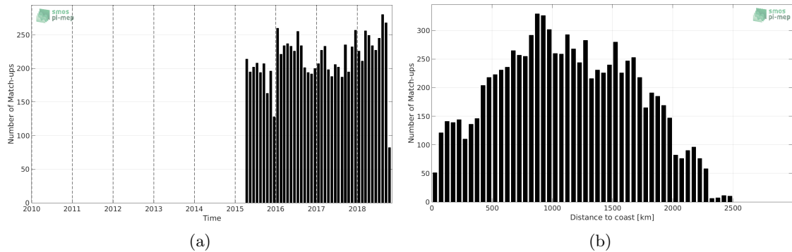
Figure 1: Number of match-ups between Argo and SMAP-L2-RSS-V3-70KM SSS as a function of time (a) and as function of the distance to coast (b) over the OTT zone Pi-MEP region and for the full satellite product period.
