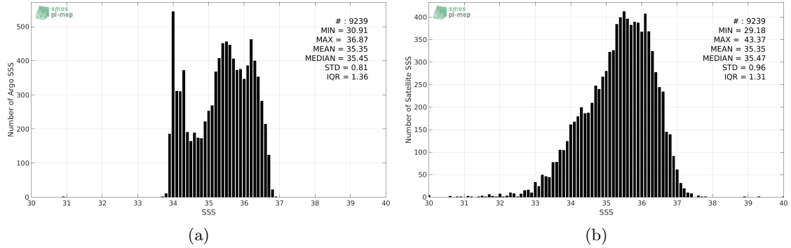
Figure 2: Histograms of SSS from Argos (a) and SMAP-L2-RSS-V3-70KM (b) considering all match-up pairs per bins of 0.1 over the OTT zone Pi-MEP region and for the full satellite product period.
