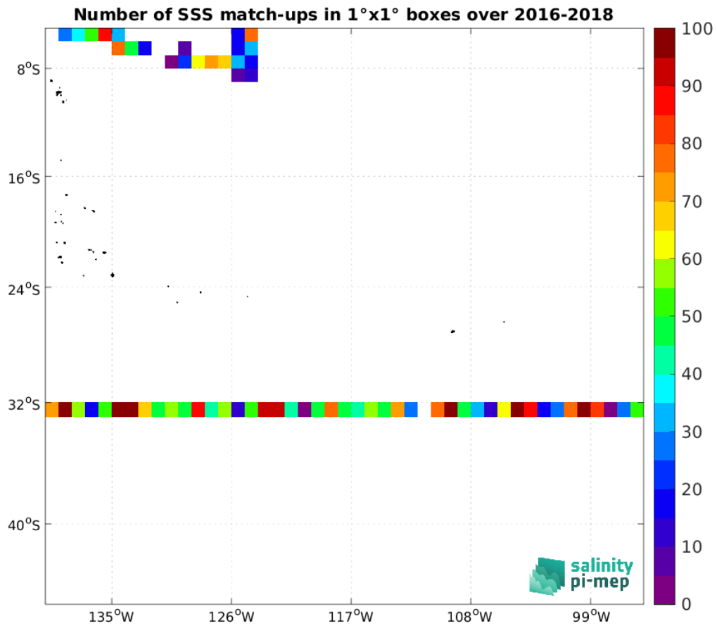
Figure 4: Number of SSS match-ups between TSG (SAMOS) SSS and the SMAP SSS L2 v5.0 (JPL) SSS product for the OTT zone Pi-MEP region over 1°x1° boxes and for the full satellite product period.
