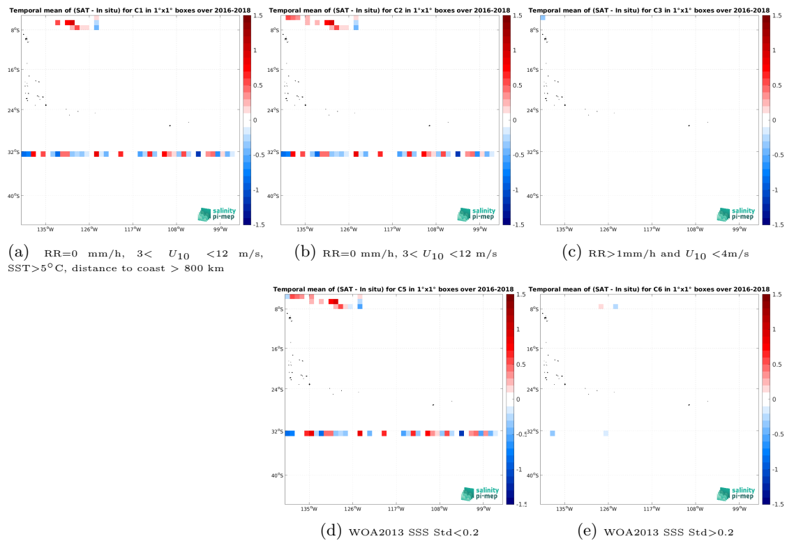
Figure 12: Temporal mean gridded over spatial boxes of size 1^\circ \times 1^\circ of \Delta\text{SSS} (SMAP SSS L2 v5.0 (JPL) - TSG (SAMOS)) for 5 different subdatasets corresponding to:RR=0 mm/h, 3 < U_{10} < 12 m/s, SST >5^\circ\text{C} , distance to coast > 800 km (a), RR=0 mm/h, 3 < U_{10} < 12 m/s (b), RR >1 mm/h and U_{10} < 4 m/s (c), WOA2013 SSS Std <0.2 (d), WOA2013 SSS Std >0.2 (e).
