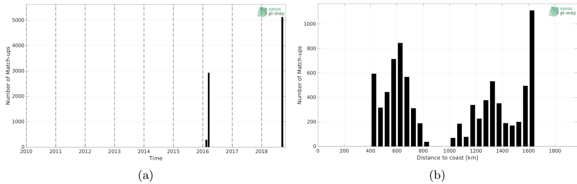
Figure 1: Number of match-ups between TSG (SAMOS) and SMAP SSS L2 v5.0 (JPL) SSS as a function of time (a) and as function of the distance to coast (b) over the OTT zone Pi-MEP region and for the full satellite product period.
