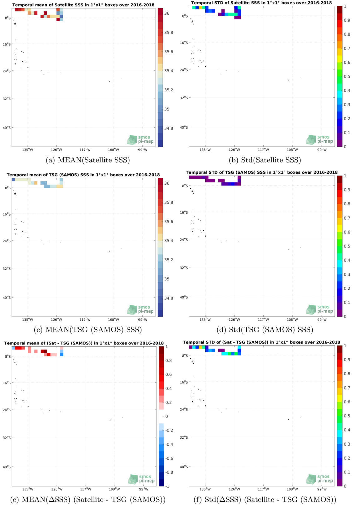
Figure 6: Temporal mean (left) and Std (right) of SSS from SMAP SSS L2 v5.0 (JPL) (top), TSG (SAMOS) (middle), and of \Delta SSS (Satellite - TSG (SAMOS)). Only match-up pairs are used to generate these maps.
