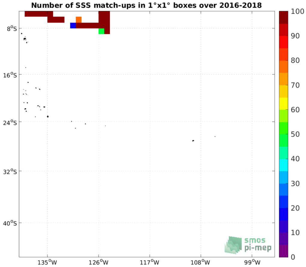
Figure 4: Number of SSS match-ups between TSG (SAMOS) SSS and the SMAP SSS L2 v5.0 (JPL) SSS product for the OTT zone Pi-MEP region over 1^\circ \times 1^\circ boxes and for the full satellite product period.
