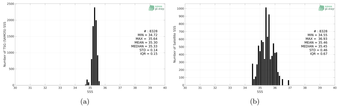
Figure 2: Histograms of SSS from TSG (SAMOS) (a) and SMAP SSS L2 v5.0 (JPL) (b) considering all match-up pairs per bins of 0.1 over the OTT zone Pi-MEP region and for the full satellite product period.
