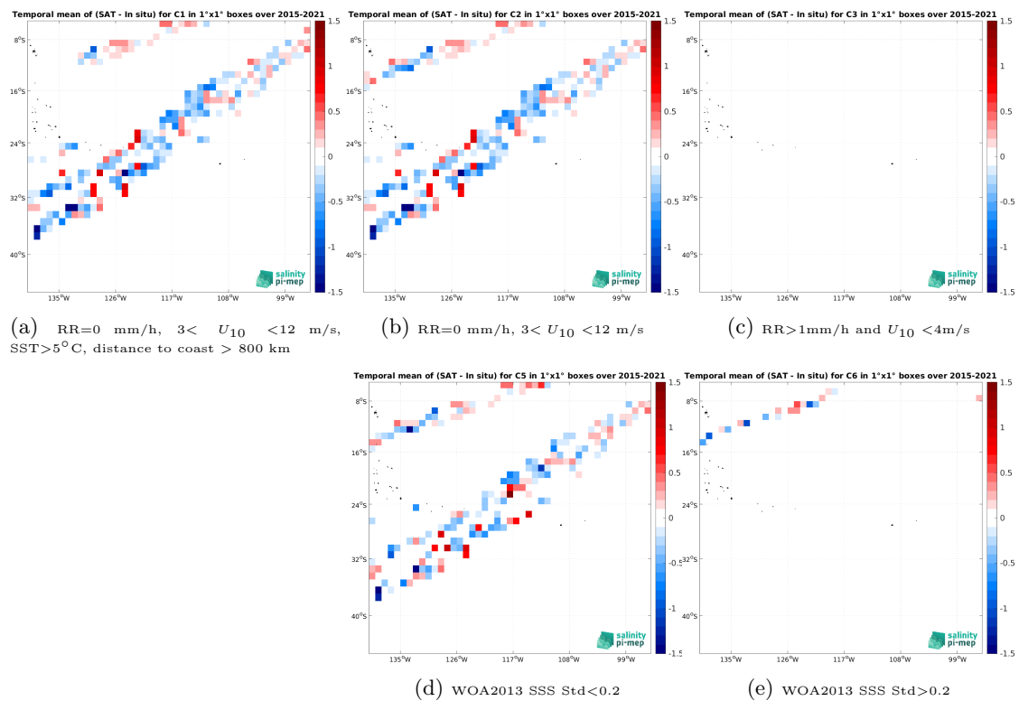
Figure 14: Temporal mean gridded over spatial boxes of size 1^\circ \times 1^\circ of \Delta SSS (SMAP SSS L2 v5.0 (JPL) - TSG (LEGOS-DM)) for 5 different subdatasets corresponding to: RR=0 mm/h, 3 < U_{10} < 12 m/s, SST > 5^\circ\text{C} , distance to coast > 800 km (a), RR=0 mm/h, 3 < U_{10} < 12 m/s (b), RR > 1 mm/h and U_{10} < 4 m/s (c), WOA2013 SSS Std < 0.2 (d), WOA2013 SSS Std > 0.2 (e).
