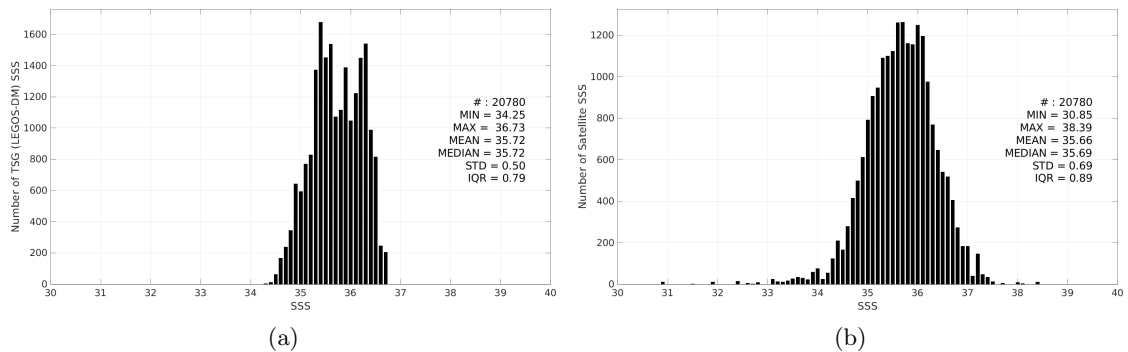
Figure 3: Histograms of SSS from TSG (LEGOS-DM) (a) and SMAP SSS L2 v5.0 (JPL) (b) considering all match-up pairs per bins of 0.1 over the OTT zone Pi-MEP region and for the full satellite product period.
