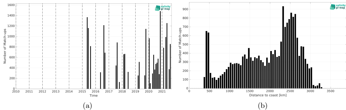
Figure 2: Number of match-ups between TSG (LEGOS-DM) and SMAP SSS L2 v5.0 (JPL) SSS as a function of time (a) and as function of the distance to coast (b) over the OTT zone Pi-MEP region and for the full satellite product period.
