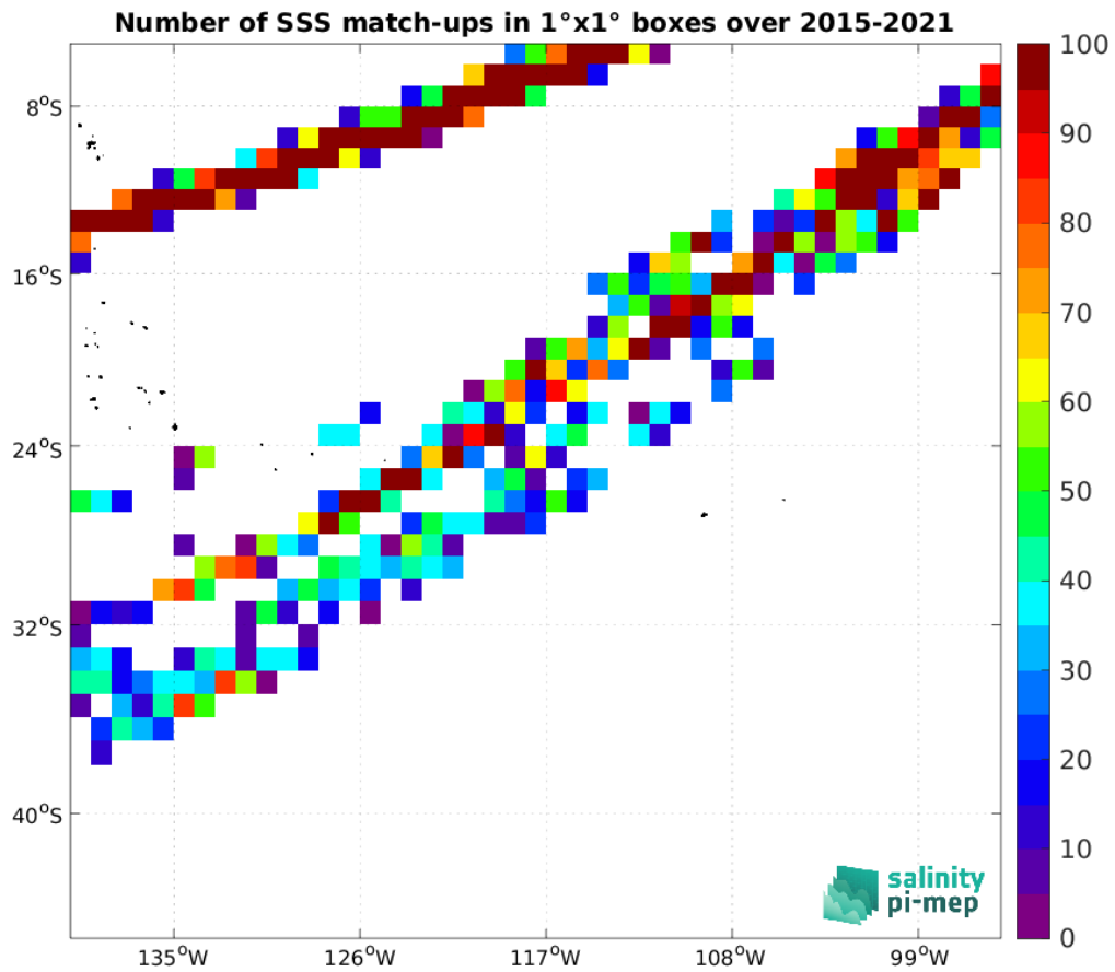
Figure 5: Number of SSS match-ups between TSG (LEGOS-DM) SSS and the SMAP SSS L2 v5.0 (JPL) SSS product for the OTT zone Pi-MEP region over 1^\circ \times 1^\circ boxes and for the full satellite product period.
