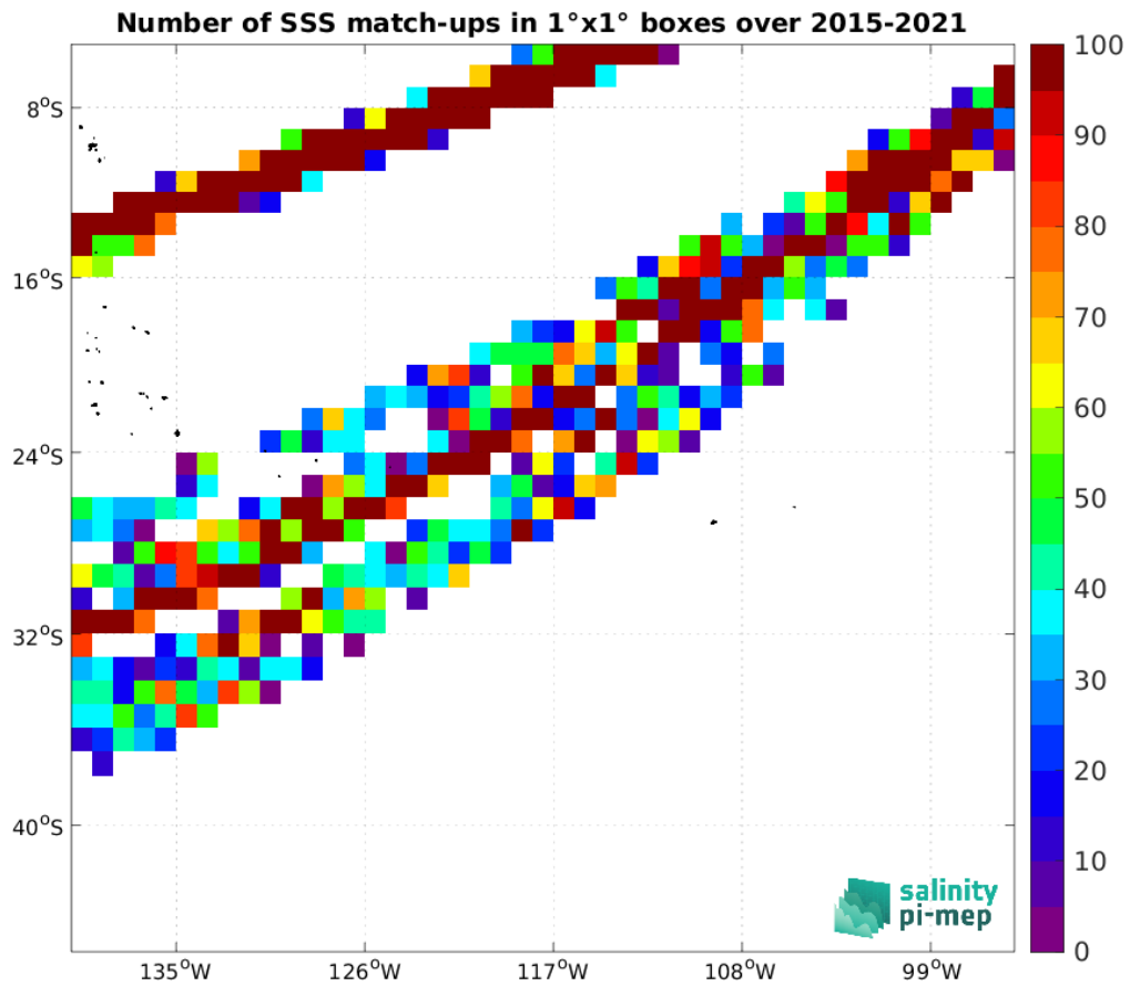
Figure 4: Number of SSS match-ups between TSG (LEGOS-DM) SSS and the SMAP SSS L2 v5.0 (JPL) SSS product for the OTT zone Pi-MEP region over 1^{\circ} \times 1^{\circ} boxes and for the full satellite product period.
