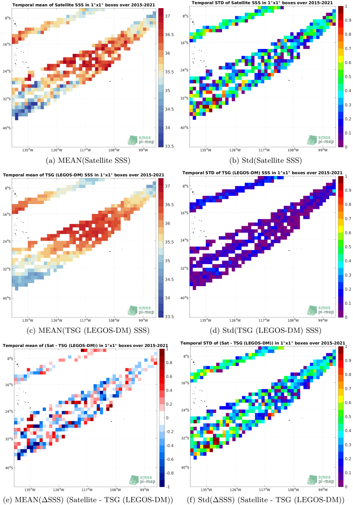
Figure 6: Temporal mean (left) and Std (right) of SSS from SMAP SSS L2 v5.0 (JPL) (top), TSG (LEGOS-DM) (middle), and of \Delta SSS (Satellite - TSG (LEGOS-DM)). Only match-up pairs are used to generate these maps.
