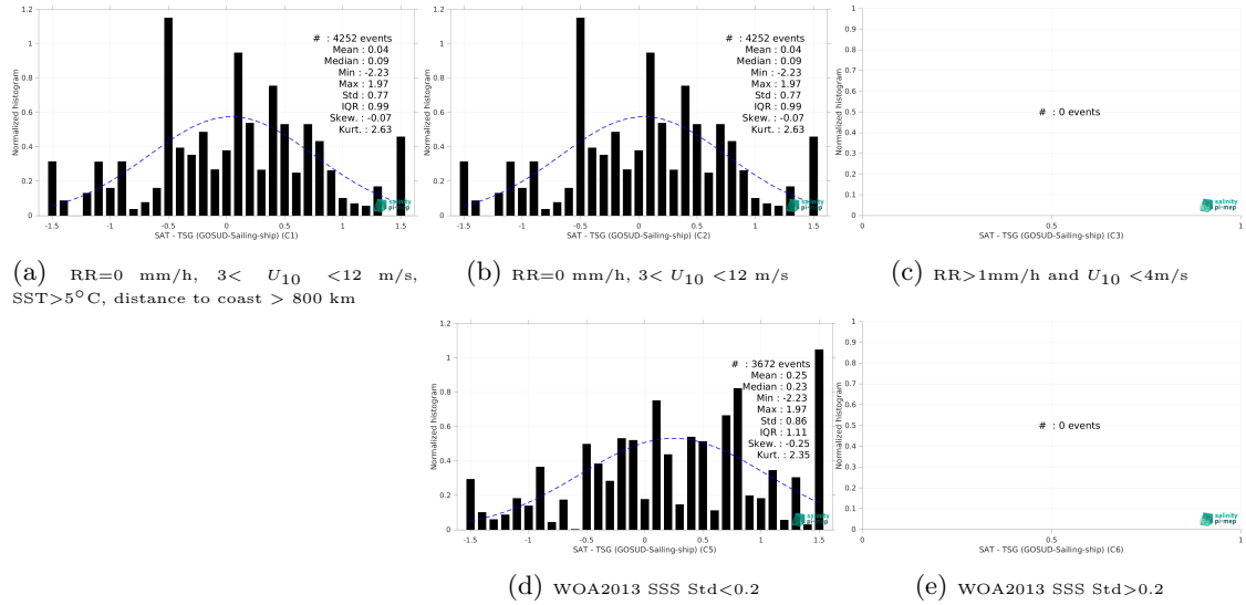
Figure 15: Normalized histogram of \Delta SSS (SMAP SSS L2 v5.0 (JPL) - TSG (GOSUD-Sailing-ship)) for 5 different subdatasets corresponding to: RR=0 mm/h, 3 < U_{10} < 12 m/s, SST >5^{\circ} C, distance to coast > 800 km (a), RR=0 mm/h, 3 < U_{10} < 12 m/s (b), RR >1 mm/h and U_{10} < 4 m/s (c), WOA2013 SSS Std <0.2 (d), WOA2013 SSS Std >0.2 (e).
