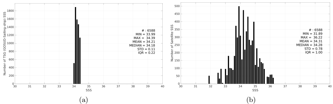
Figure 3: Histograms of SSS from TSG (GOSUD-Sailing-ship) (a) and SMAP SSS L2 v5.0 (JPL) (b) considering all match-up pairs per bins of 0.1 over the OTT zone Pi-MEP region and for the full satellite product period.
