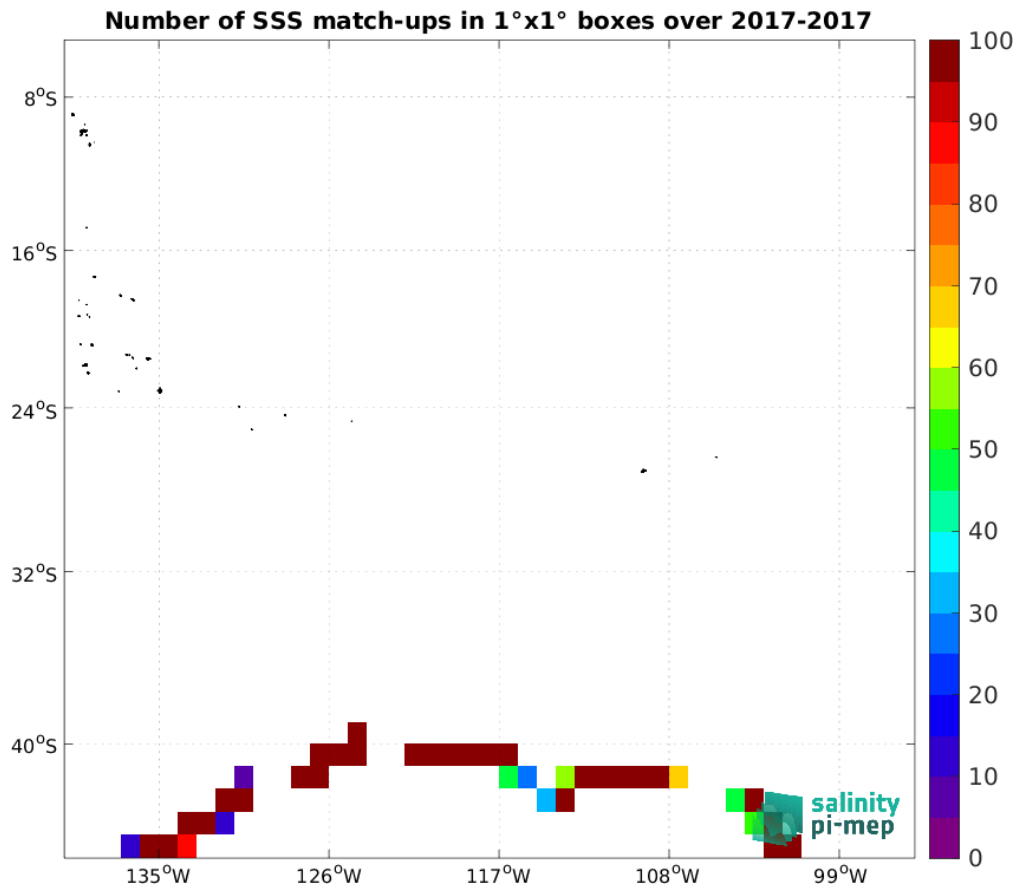
Figure 5: Number of SSS match-ups between TSG (GOSUD-Sailing-ship) SSS and the SMAP SSS L2 v5.0 (JPL) SSS product for the OTT zone Pi-MEP region over 1^\circ \times 1^\circ boxes and for the full satellite product period.
