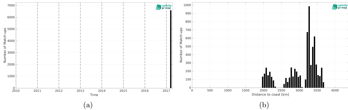
Figure 2: Number of match-ups between TSG (GOSUD-Sailing-ship) and SMAP SSS L2 v5.0 (JPL) SSS as a function of time (a) and as function of the distance to coast (b) over the OTT zone Pi-MEP region and for the full satellite product period.
