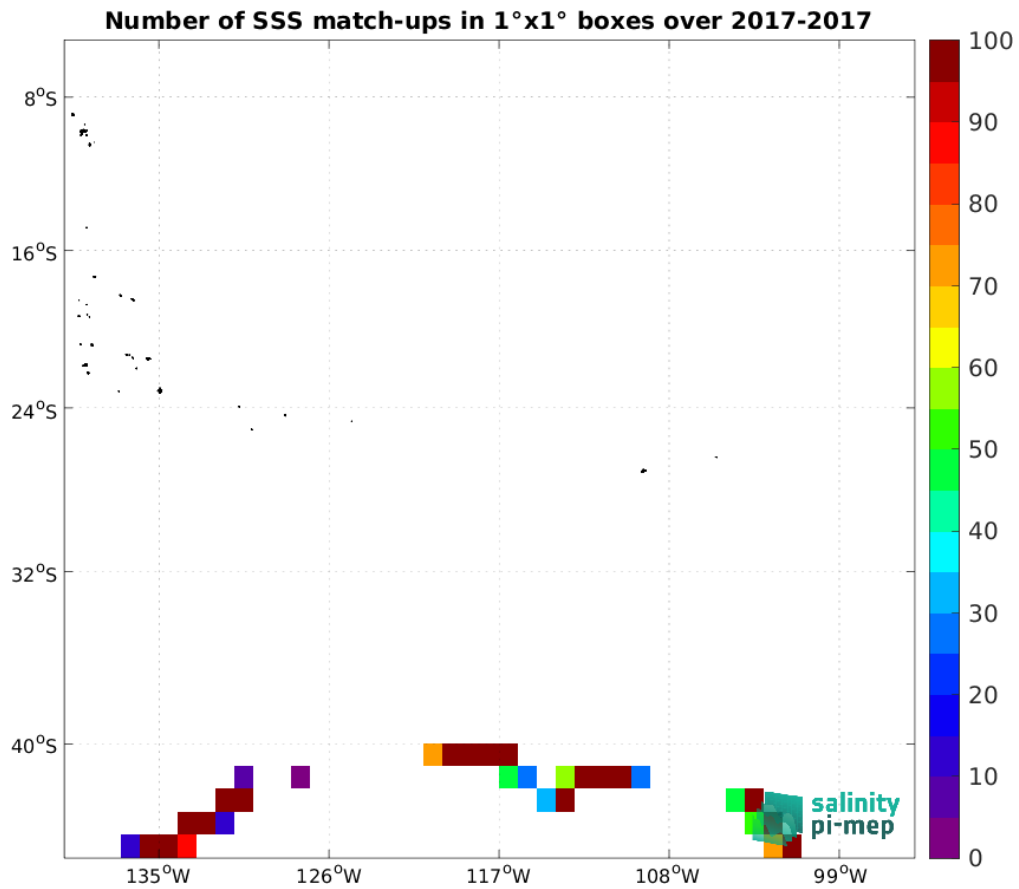
Figure 5: Number of SSS match-ups between TSG (GOSUD-Sailing-ship) SSS and the SMAP SSS L2 v5.0 (JPL) SSS product for the OTT zone Pi-MEP region over 1°×1° boxes and for the full satellite product period.
