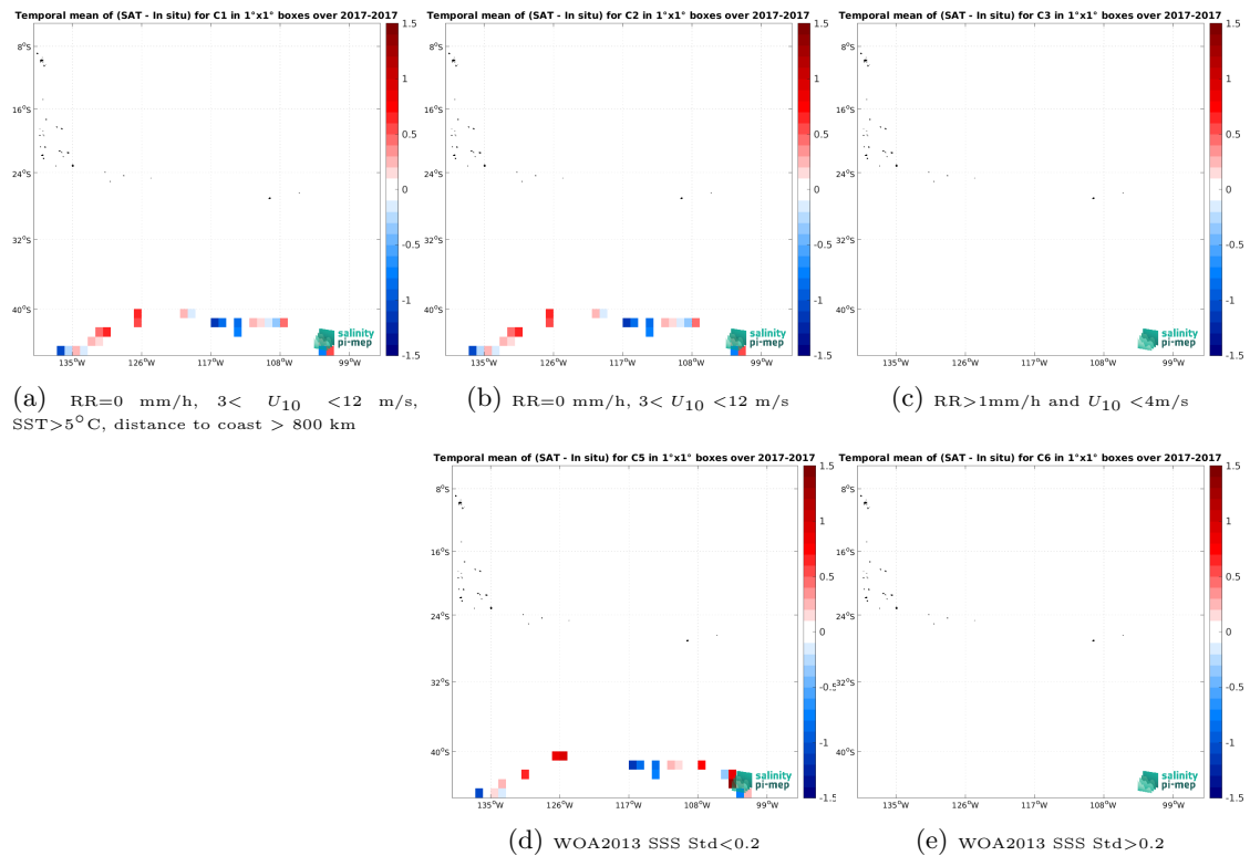
Figure 12: Temporal mean gridded over spatial boxes of size 1^\circ \times 1^\circ of \Delta\text{SSS} (SMAP SSS L2 v5.0 (JPL) - TSG (GOSUD-Sailing-ship)) for 5 different subdatasets corresponding to:RR=0 mm/h, 3 < U_{10} < 12 m/s, SST>5°C, distance to coast > 800 km (a), RR=0 mm/h, 3 < U_{10} < 12 m/s (b), RR>1mm/h and U_{10} < 4 m/s (c), WOA2013 SSS Std<0.2 (d), WOA2013 SSS Std>0.2 (e).
