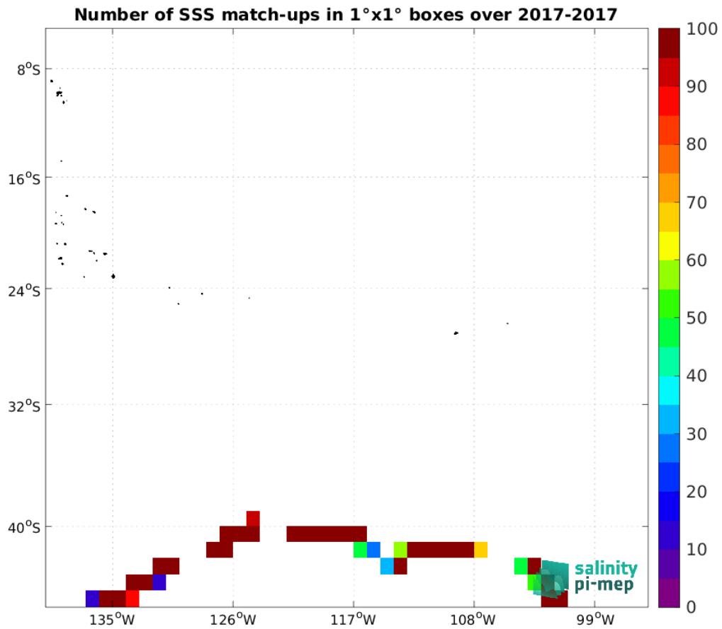
Figure 4: Number of SSS match-ups between TSG (GOSUD-Sailing-ship) SSS and the SMAP SSS L2 v5.0 (JPL) SSS product for the OTT zone Pi-MEP region over 1°×1° boxes and for the full satellite product period.
