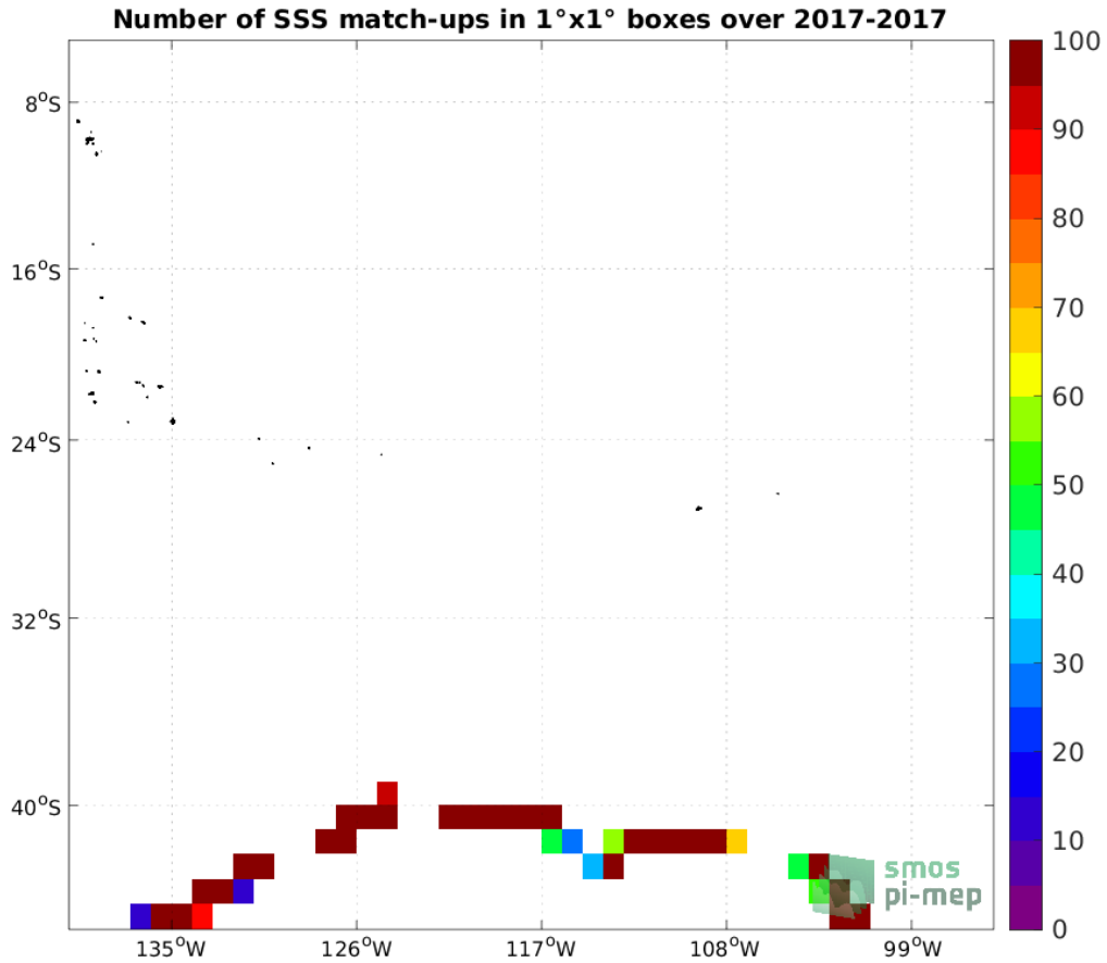
Figure 4: Number of SSS match-ups between TSG (GOSUD-Sailing-ship) SSS and the SMAP SSS L2 v5.0 (JPL) SSS product for the OTT zone Pi-MEP region over 1^\circ \times 1^\circ boxes and for the full satellite product period.
