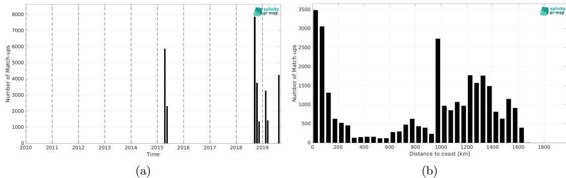
Figure 2: Number of match-ups between TSG (GOSUD-Research-vessel) and SMAP SSS L2 v5.0 (JPL) SSS as a function of time (a) and as function of the distance to coast (b) over the OTT zone Pi-MEP region and for the full satellite product period.
