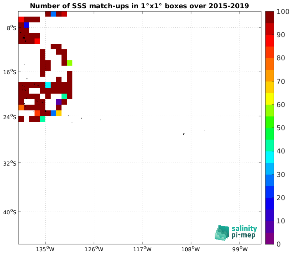
Figure 5: Number of SSS match-ups between TSG (GOSUD-Research-vessel) SSS and the SMAP SSS L2 v5.0 (JPL) SSS product for the OTT zone Pi-MEP region over 1°×1° boxes and for the full satellite product period.
