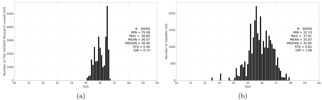
Figure 3: Histograms of SSS from TSG (GOSUD-Research-vessel) (a) and SMAP SSS L2 v5.0 (JPL) (b) considering all match-up pairs per bins of 0.1 over the OTT zone Pi-MEP region and for the full satellite product period.
