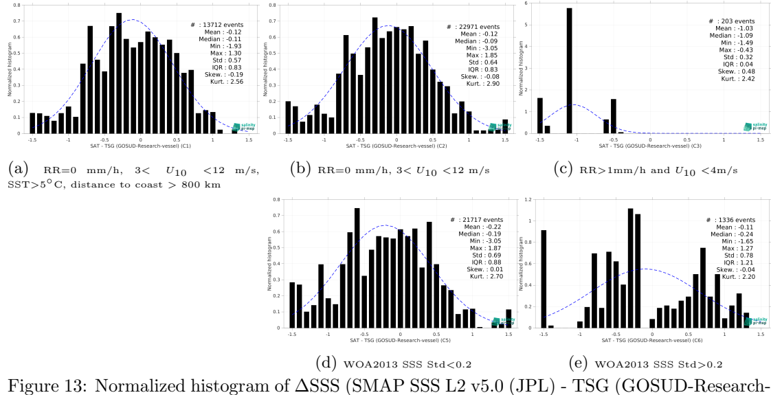
Figure 13: Normalized histogram of \Delta SSS (SMAP SSS L2 v5.0 (JPL) - TSG (GOSUD-Research-vessel)) for 5 different subdatasets corresponding to: RR=0 mm/h, 3 < U_{10} < 12 m/s, SST > 5°C, distance to coast > 800 km (a), RR=0 mm/h, 3 < U_{10} < 12 m/s (b), RR > 1mm/h and U_{10} < 4 m/s (c), WOA2013 SSS Std < 0.2 (d), WOA2013 SSS Std > 0.2 (e).
