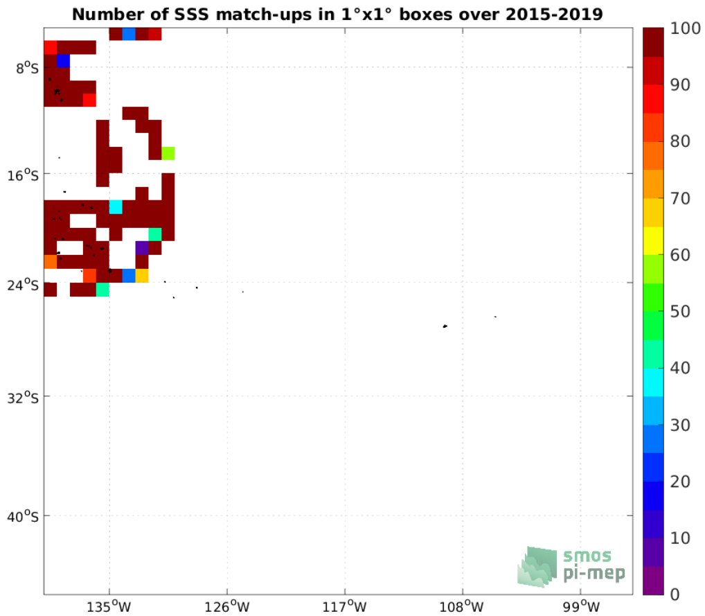
Figure 4: Number of SSS match-ups between TSG (GOSUD-Research-vessel) SSS and the SMAP SSS L2 v5.0 (JPL) SSS product for the OTT zone Pi-MEP region over 1°×1° boxes and for the full satellite product period.
