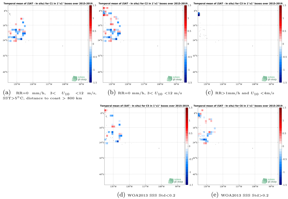
Figure 12: Temporal mean gridded over spatial boxes of size 1^\circ \times 1^\circ of \Delta SSS (SMAP SSS L2 v5.0 (JPL) - TSG (GOSUD-Research-vessel)) for 5 different subdatasets corresponding to: RR=0 mm/h, 3 < U_{10} < 12 m/s, SST > 5°C, distance to coast > 800 km (a), RR=0 mm/h, 3 < U_{10} < 12 m/s (b), RR > 1 mm/h and U_{10} < 4 m/s (c), WOA2013 SSS Std < 0.2 (d), WOA2013 SSS Std > 0.2 (e).
