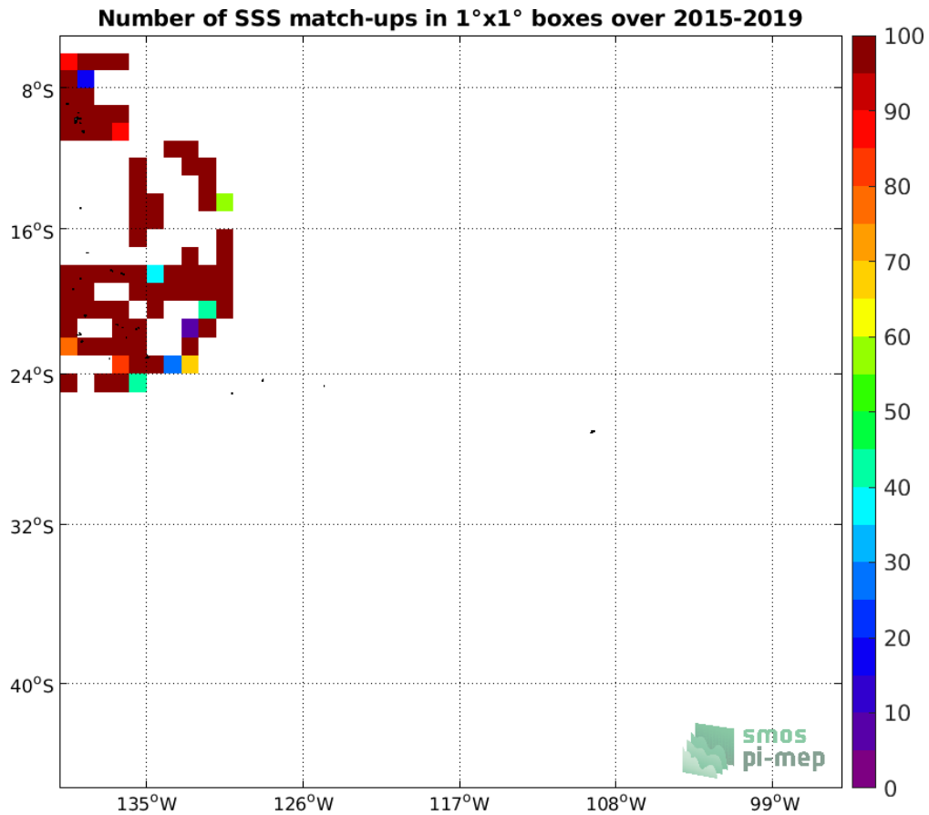
Figure 4: Number of SSS match-ups between TSG (GOSUD-Research-vessel) SSS and the SMAP SSS L2 v5.0 (JPL) SSS product for the OTT zone Pi-MEP region over 1°x1° boxes and for the full satellite product period.
