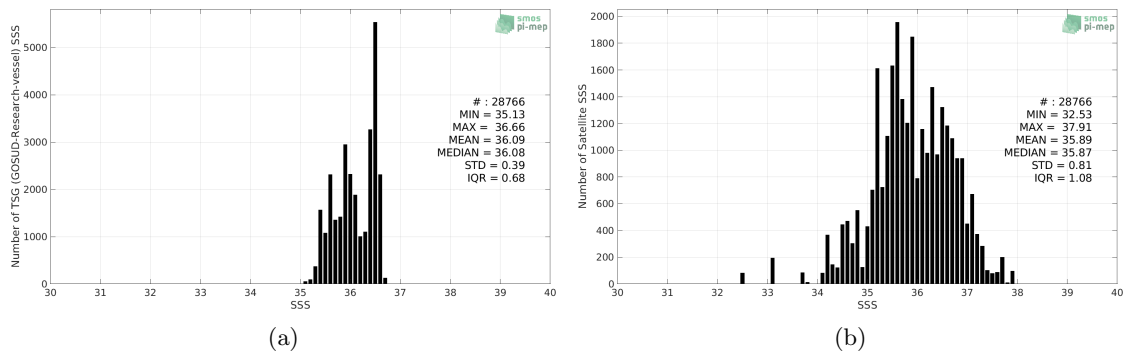
Figure 2: Histograms of SSS from TSG (GOSUD-Research-vessel) (a) and SMAP SSS L2 v5.0 (JPL) (b) considering all match-up pairs per bins of 0.1 over the OTT zone Pi-MEP region and for the full satellite product period.
