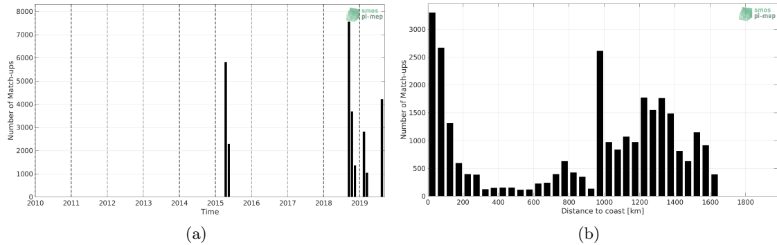
Figure 1: Number of match-ups between TSG (GOSUD-Research-vessel) and SMAP SSS L2 v5.0 (JPL) SSS as a function of time (a) and as function of the distance to coast (b) over the OTT zone Pi-MEP region and for the full satellite product period.
