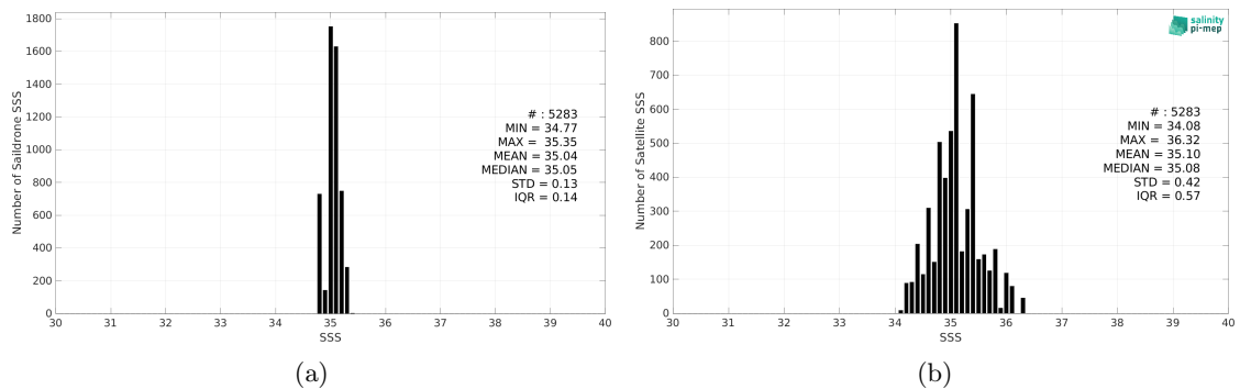
Figure 2: Histograms of SSS from Saildrone (a) and SMAP SSS L2 v5.0 (JPL) (b) considering all match-up pairs per bins of 0.1 over the OTT zone Pi-MEP region and for the full satellite product period.
