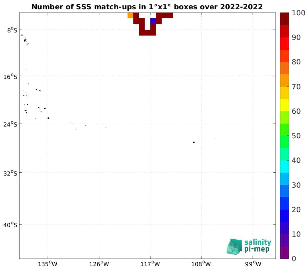
Figure 4: Number of SSS match-ups between Saildrone SSS and the SMAP SSS L2 v5.0 (JPL) SSS product for the OTT zone Pi-MEP region over 1°×1° boxes and for the full satellite product period.
