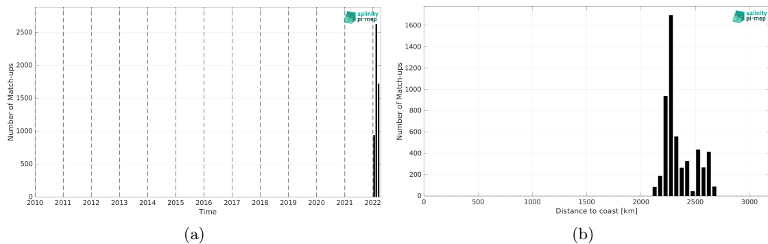
Figure 1: Number of match-ups between Saildrone and SMAP SSS L2 v5.0 (JPL) SSS as a function of time (a) and as function of the distance to coast (b) over the OTT zone Pi-MEP region and for the full satellite product period.
