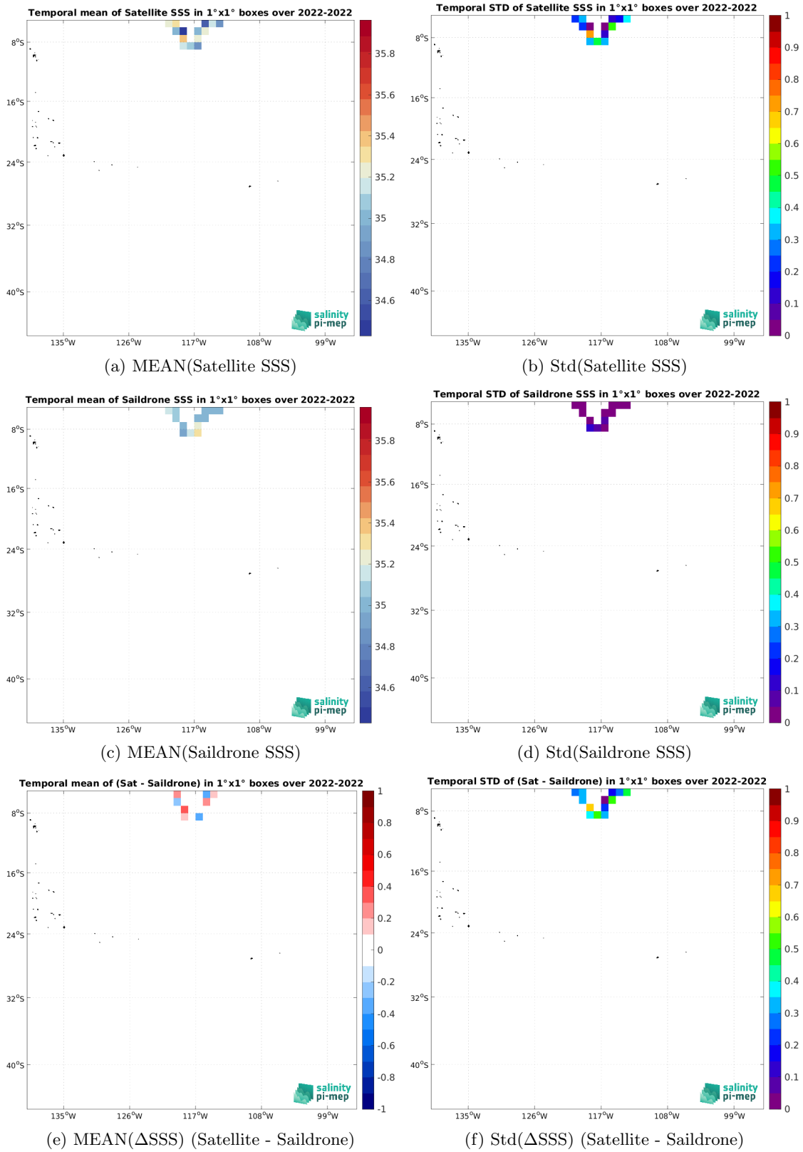
Figure 6: Temporal mean (left) and Std (right), of SSS from SMAP SSS L2 v5.0 (JPL) (top), Saildrone (middle), and of \Delta SSS (Satellite - Saildrone). Only match-up pairs are used to generate these maps.
