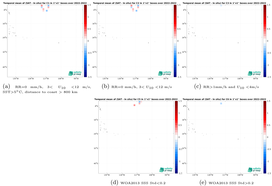
Figure 12: Temporal mean gridded over spatial boxes of size 1^\circ \times 1^\circ of \Delta SSS (SMAP SSS L2 v5.0 (JPL) - Saildrone) for 5 different subdatasets corresponding to:RR=0 mm/h, 3 < U_{10} < 12 m/s, SST > 5^\circ\text{C} , distance to coast > 800 km (a), RR=0 mm/h, 3 < U_{10} < 12 m/s (b), RR > 1 mm/h and U_{10} < 4 m/s (c), WOA2013 SSS Std < 0.2 (d), WOA2013 SSS Std > 0.2 (e).
