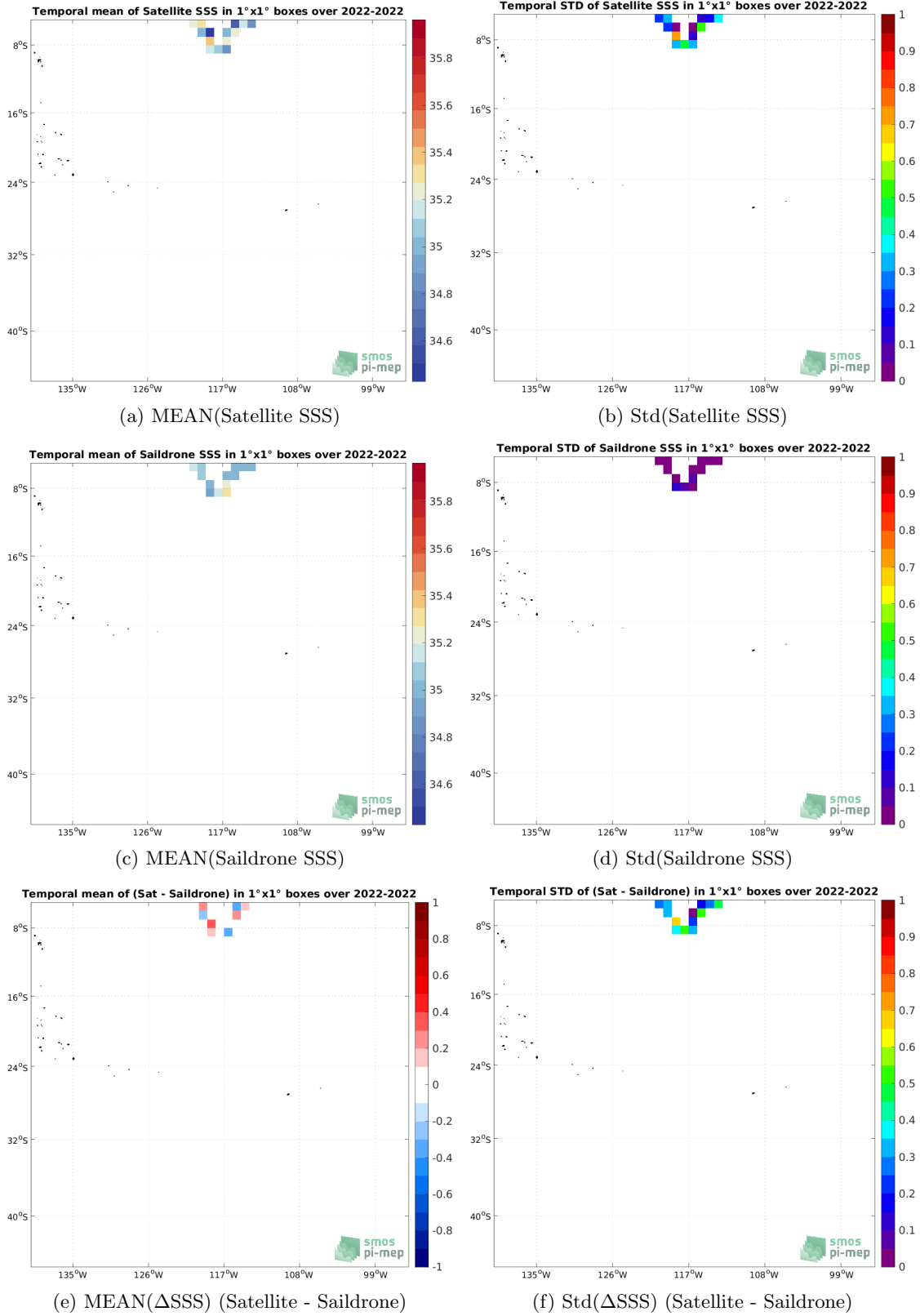
Figure 6: Temporal mean (left) and Std (right) of SSS from SMAP SSS L2 v5.0 (JPL) (top), Saildrone (middle), and of \Delta SSS (Satellite - Saildrone). Only match-up pairs are used to generate these maps.
