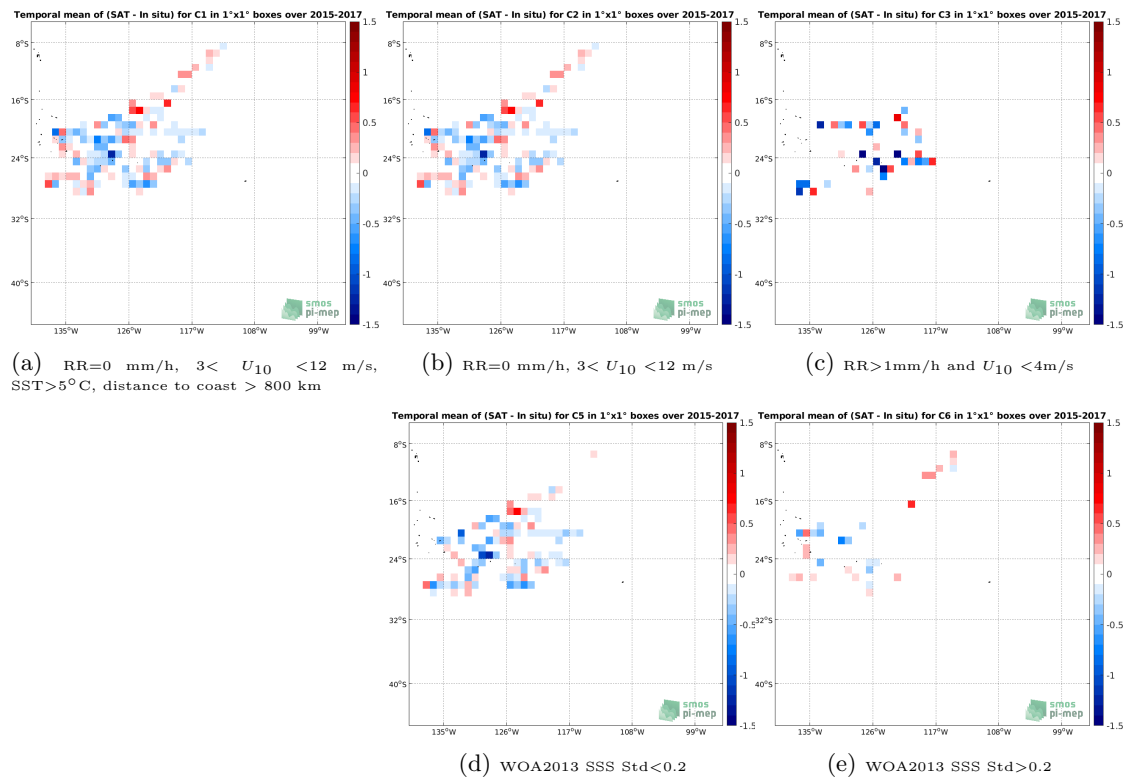
Figure 11: Temporal mean gridded over spatial boxes of size 1^\circ \times 1^\circ of \Delta\text{SSS} (SMAP SSS L2 v5.0 (JPL) - Surface drifters) for 5 different subdatasets corresponding to:RR=0 mm/h, 3 < U_{10} < 12 m/s, SST >5^\circ\text{C} , distance to coast > 800 km (a), RR=0 mm/h, 3 < U_{10} < 12 m/s (b), RR >1 mm/h and U_{10} < 4 m/s (c), WOA2013 SSS Std <0.2 (d), WOA2013 SSS Std >0.2 (e).
