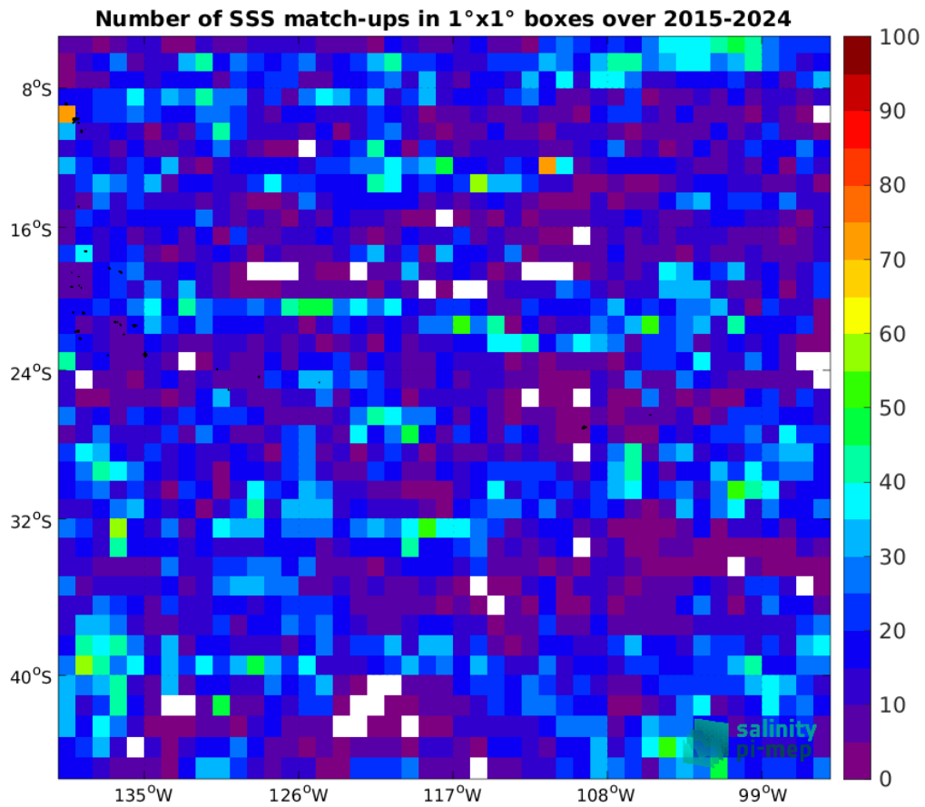
Figure 5: Number of SSS match-ups between Argo SSS and the SMAP SSS L2 v5.0 (JPL) SSS product for the OTT zone Pi-MEP region over 1°x1° boxes and for the full satellite product period.
