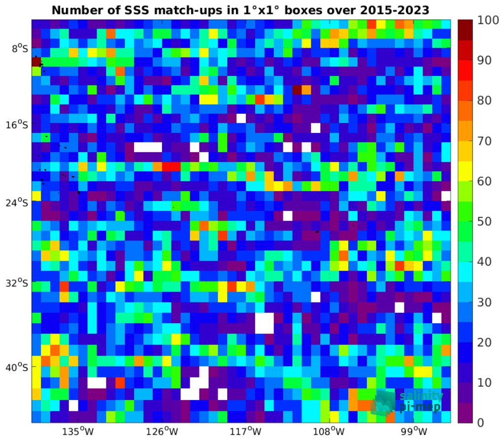
Figure 4: Number of SSS match-ups between Argo SSS and the SMAP SSS L2 v5.0 (JPL) SSS product for the OTT zone Pi-MEP region over 1^\circ \times 1^\circ boxes and for the full satellite product period.
