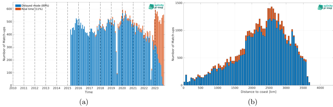
Figure 1: Number of match-ups between Argo and SMAP SSS L2 v5.0 (JPL) SSS as a function of time (a) and as function of the distance to coast (b) over the OTT zone Pi-MEP region and for the full satellite product period.
