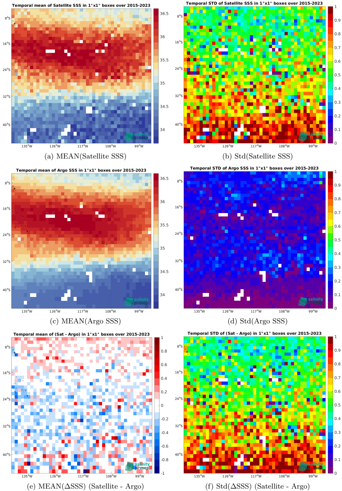
Figure 6: Temporal mean (left) and Std (right) of SSS from SMAP SSS L2 v5.0 (JPL) (top), Argo (middle), and of \Delta SSS (Satellite - Argo). Only match-up pairs are used to generate these maps.
