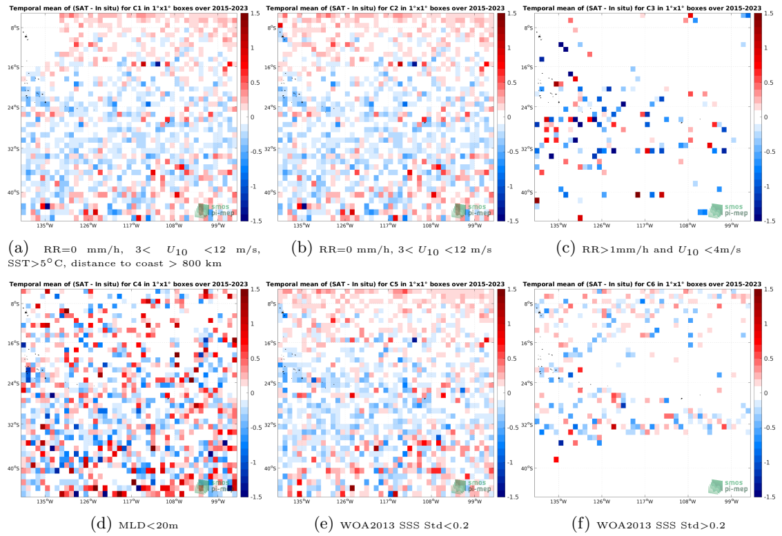
Figure 12: Temporal mean gridded over spatial boxes of size 1^\circ \times 1^\circ of \Delta SSS (SMAP SSS L2 v5.0 (JPL) - Argo) for 6 different subdatasets corresponding to:RR=0 mm/h, 3 < U_{10} < 12 m/s, SST > 5^\circ\text{C} , distance to coast > 800 km (a), RR=0 mm/h, 3 < U_{10} < 12 m/s (b), RR > 1 mm/h and U_{10} < 4 m/s (c),MLD < 20 m (d),WOA2013 SSS Std < 0.2 (e),WOA2013 SSS Std > 0.2 (f).
