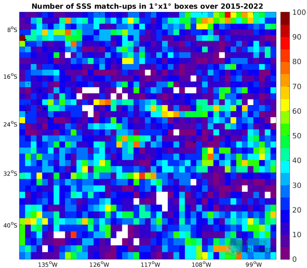
Figure 4: Number of SSS match-ups between Argo SSS and the SMAP SSS L2 v5.0 (JPL) SSS product for the OTT zone Pi-MEP region over 1°x1° boxes and for the full satellite product period.
