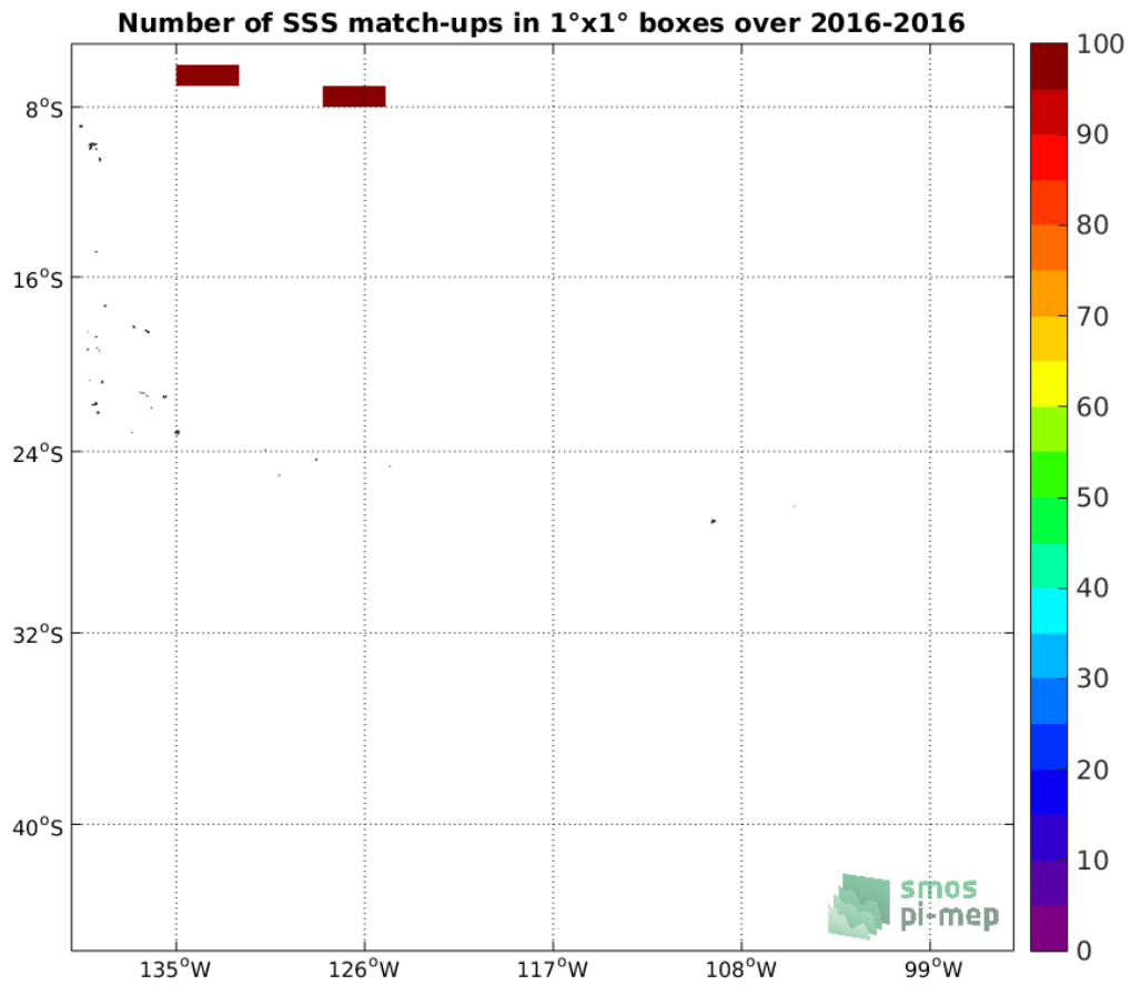
Figure 4: Number of SSS match-ups between TSG-SAMOS SSS and the SMAP-L2-JPL-V4 SSS product for the OTT zone Pi-MEP region over 1°x1° boxes and for the full satellite product period.
