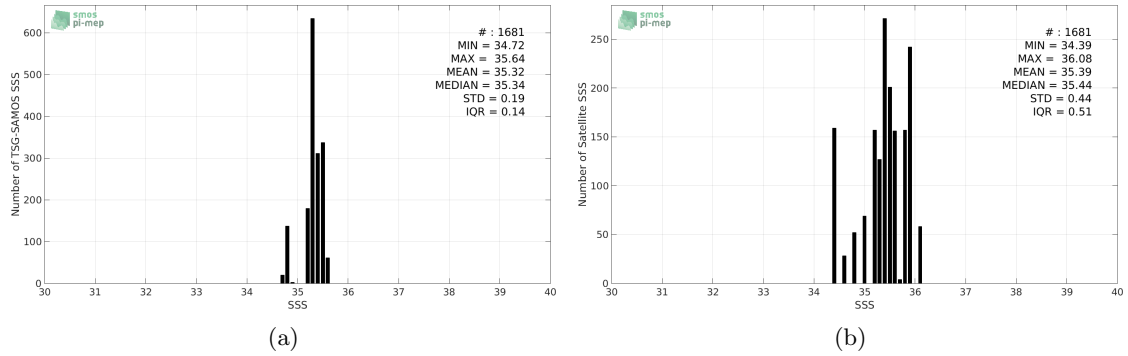
Figure 2: Histograms of SSS from TSG-SAMOS (a) and SMAP-L2-JPL-V4 (b) considering all match-up pairs per bins of 0.1 over the OTT zone Pi-MEP region and for the full satellite product period.
