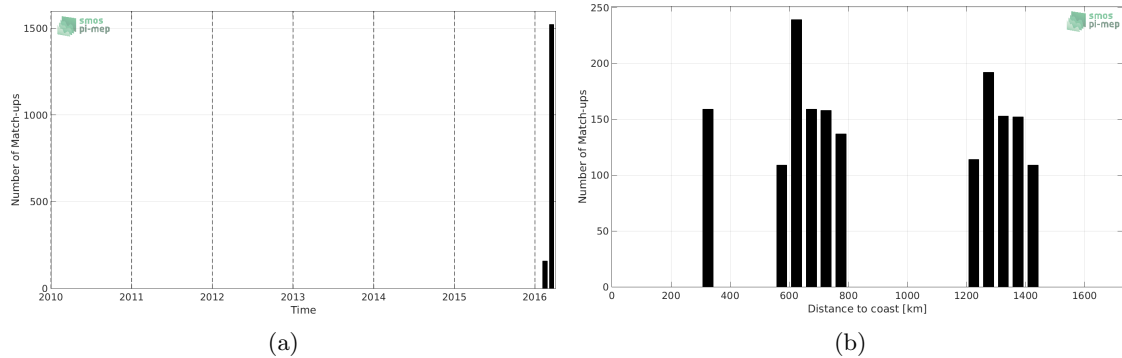
Figure 1: Number of match-ups between TSG-SAMOS and SMAP-L2-JPL-V4 SSS as a function of time (a) and as function of the distance to coast (b) over the OTT zone Pi-MEP region and for the full satellite product period.
