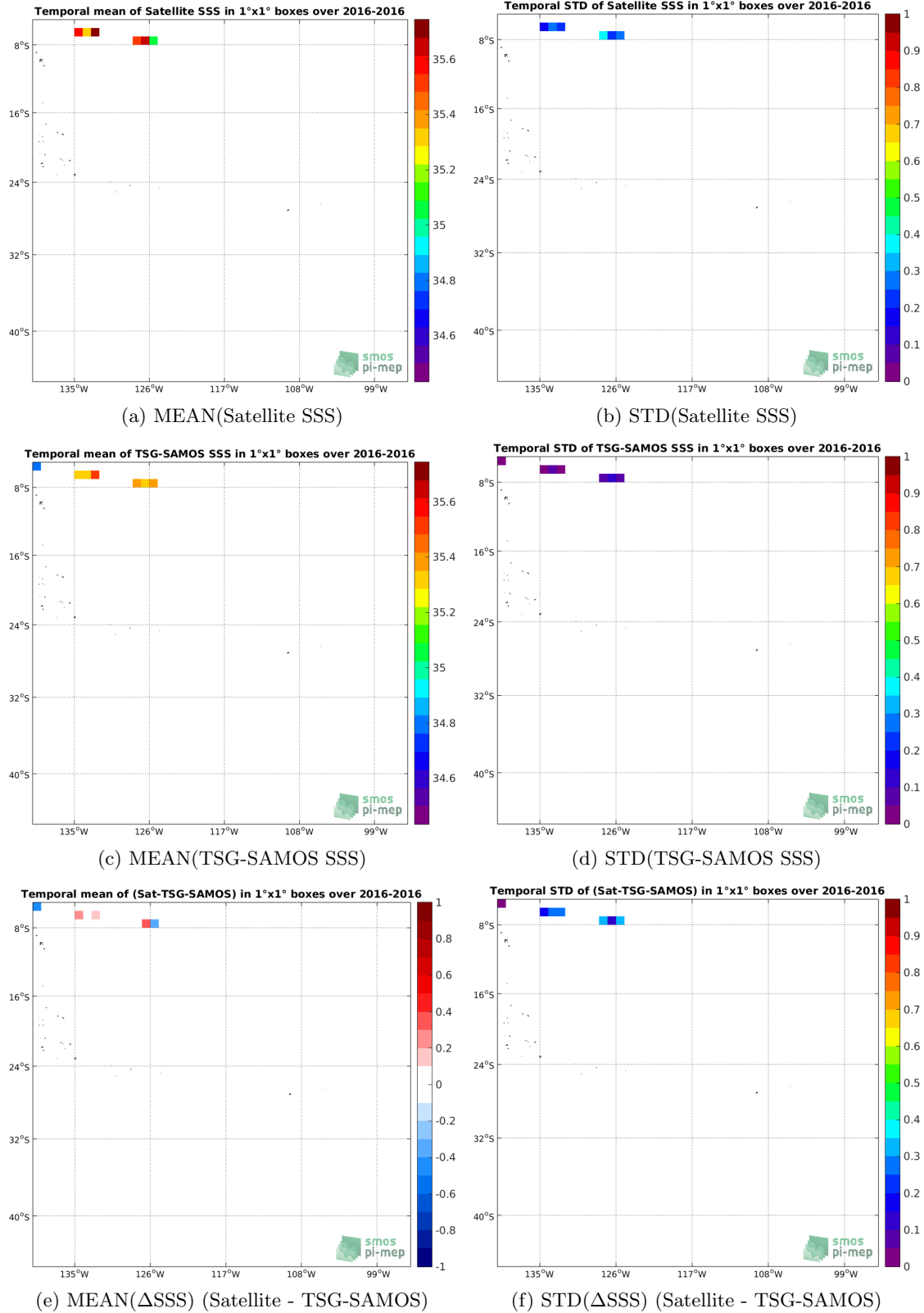
Figure 6: Temporal mean (left) and STD (right) of SSS from SMAP-L2-JPL-V4 (top), TSG-SAMOS (middle), and of \Delta SSS (Satellite - TSG-SAMOS). Only match-up pairs are used to generate these maps.
