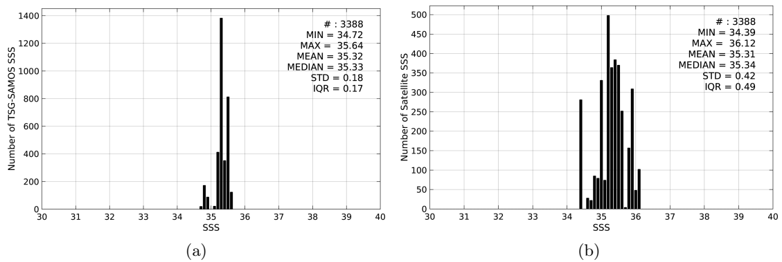
Figure 2: Histograms of SSS from TSG-SAMOS (a) and SMAP-L2-JPL-V4 (b) considering all match-up pairs per bins of 0.1 over the OTT zone Pi-MEP region and for the full satellite product period.
