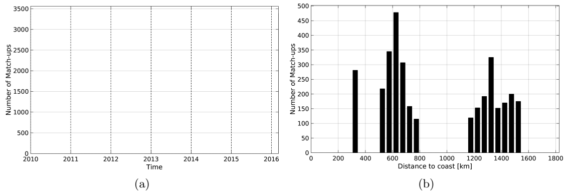
Figure 1: Number of match-ups between TSG-SAMOS and SMAP-L2-JPL-V4 SSS as a function of time (a) and as function of the distance to coast (b) over the OTT zone Pi-MEP region and for the full satellite product period.
